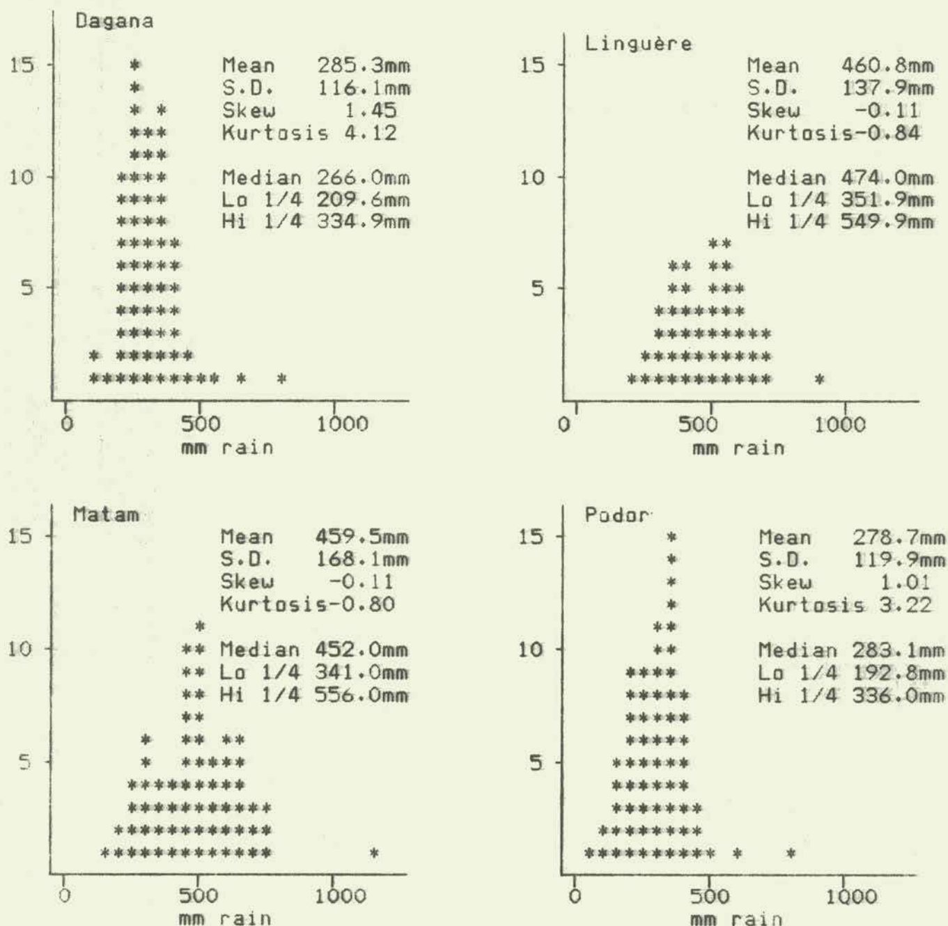
Figure 4: Frequency distributions of annual rainfall at four stations in the Ferlo
