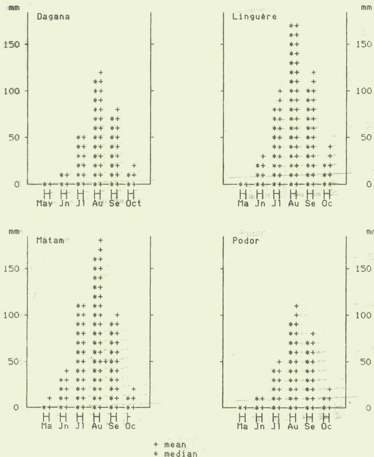
Figure 5: Medians and mean monthly rainfall at four stations in the Ferlo
