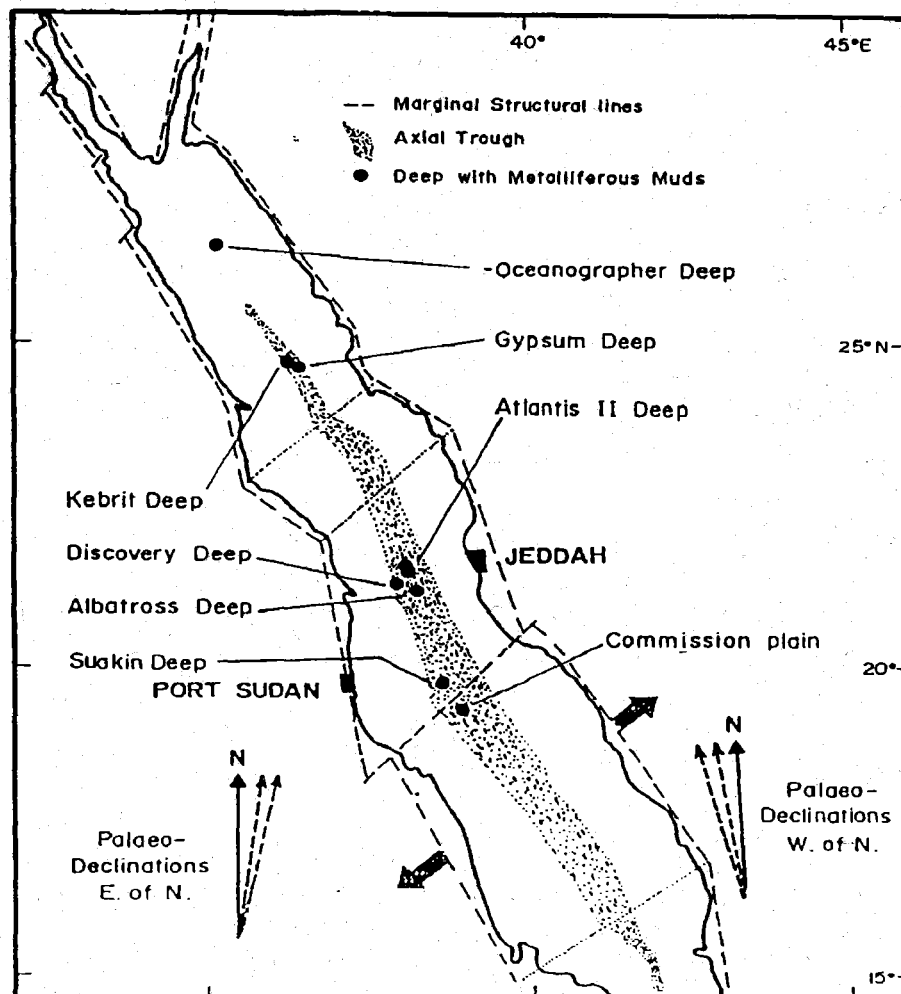
Figure 21: Red Sea structural map showing some of the metalliferous muds. (Source: Nawab, 1983).
