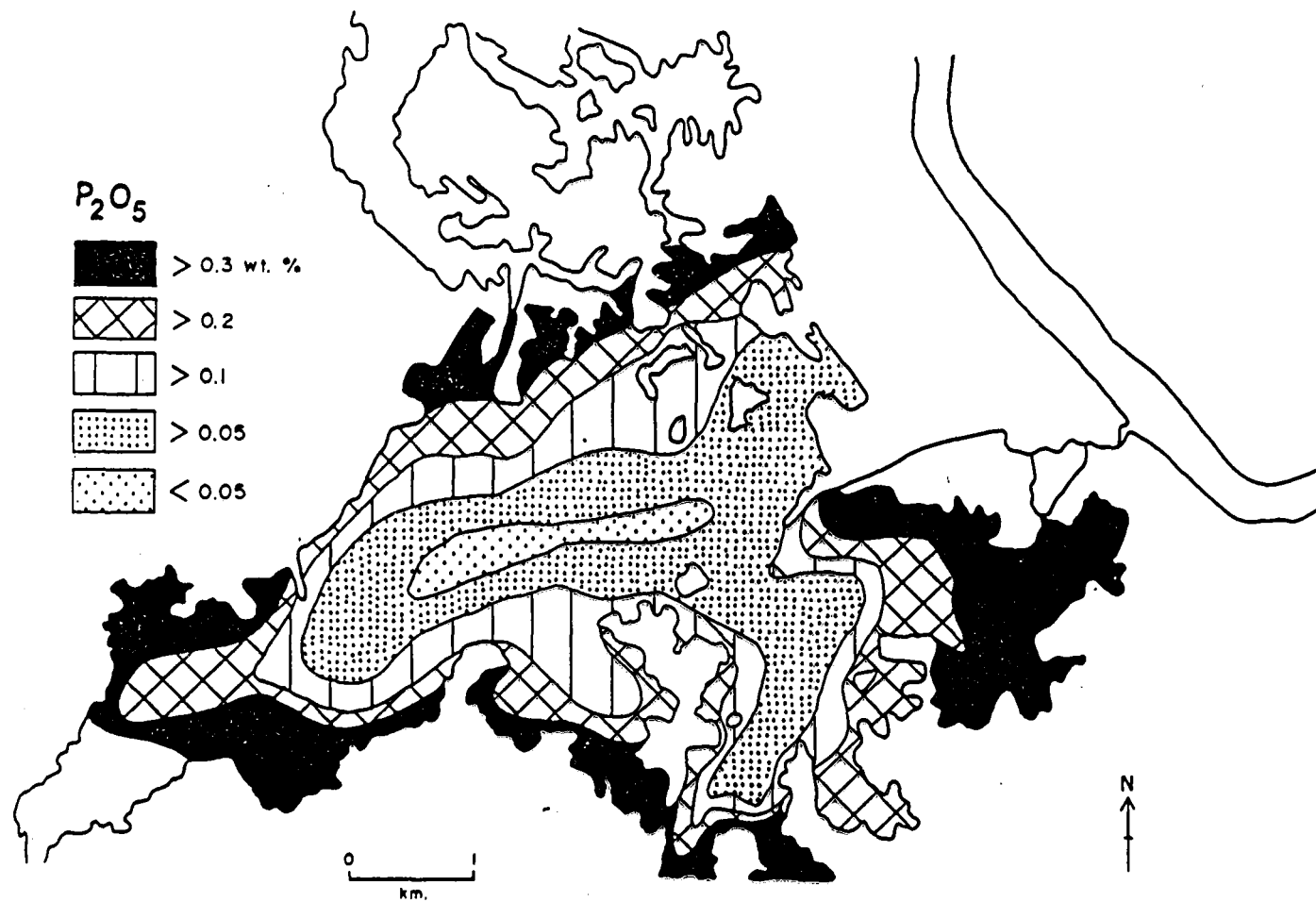
Figure 2. Distribution of phosphorus in surface sediments collected from 32 sites in Lake Daviumbu, Papua New Guinea. (Reproduced with permission from Osborne et al. , (in press). Geochemical traces of riverine influence on a tropical lateral lake. Verh. Internat. Verein. Limnol., 23.)
