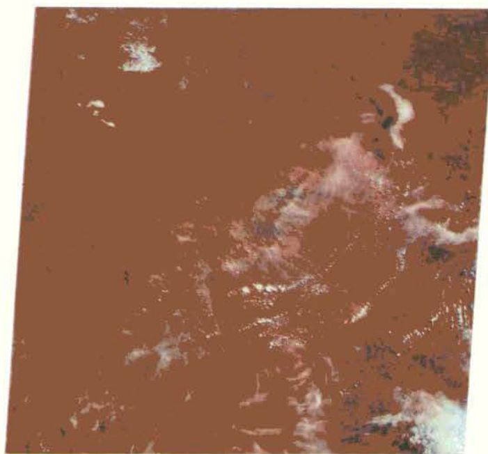
Figure 2. Scene 2134-08470, 5 June 1975. Except for the extreme southern part the area lies to the north of that mapped in Cameroon. The overwhelming spectral response of the new grass cover early in the rainy season is well illustrated, as well as the incidence of cloud.
