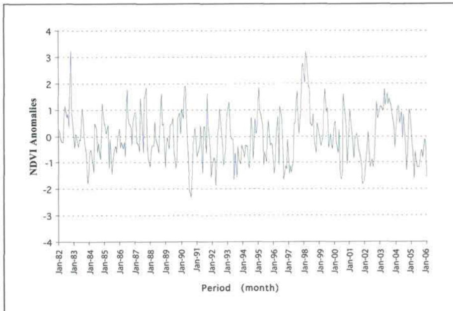
Fig. ii. Monthly NDVI anomalies between 1982 and 2006 for Kwale district
