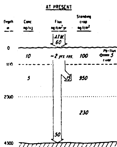
Fig. 2. Oceanic outputs, river and atmospheric inputs, and reservoirs of soluble lead at present times in the open North Pacific (Schaule & Patterson, 1980).
