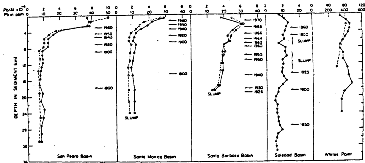
Fig. 4. Lead content (•) and lead/aluminium ratios (o) in Southern California Basin sediments, and Whites Point sewer outfall sediments; note change of scale, Whites Point. Vertical dating of sediments is indicated. From: Bertine (1980).
