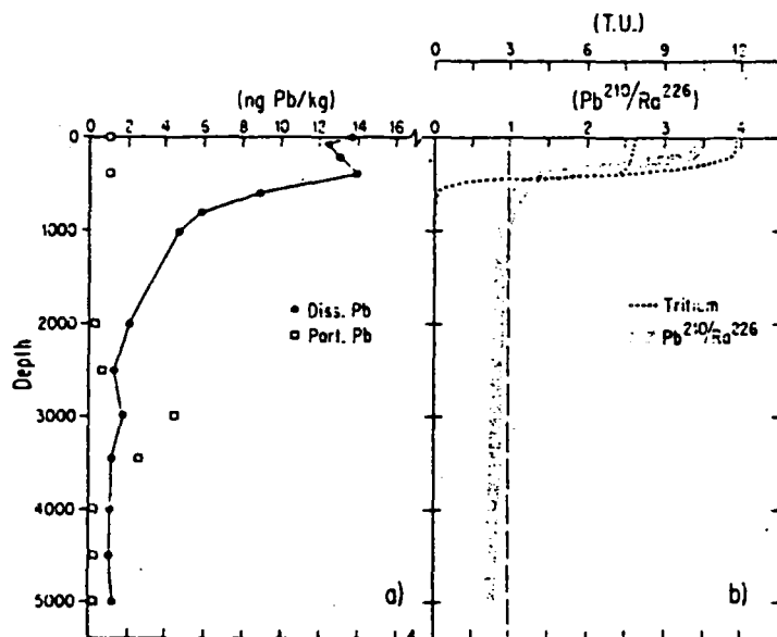
Fig. 3. (a) Generalized depth profile of common lead concentration in the central northeast Pacific Ocean. (b) General structure of tritium and ^{210}Pb distribution in the central northeast Pacific Ocean. From: Schaule & Patterson (1980).
