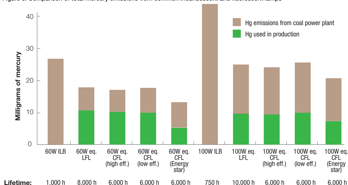
Figure 6: Comparison of total mercury emissions from common incandescent and fluorescent lamps 41
