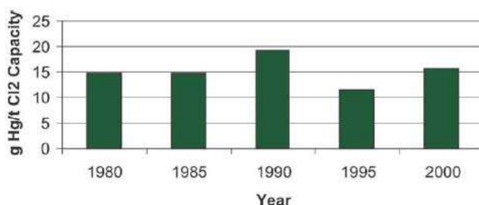
Figure 1.6 - Mercury in solid waste from chlor-alkali plants in EU-15+Switzerland (from Garny, 2001).
