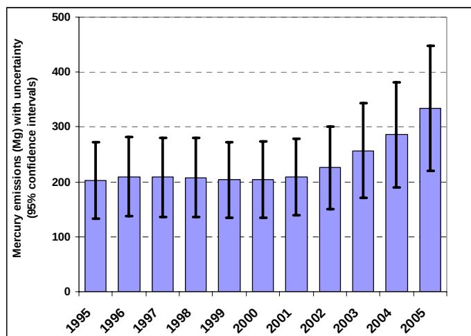
Figure 2.7 - Uncertainty in mercury emission estimates for coal combustion, as 95% confidence intervals.
