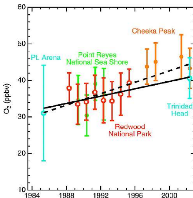
Figure 13.6 - Spring mean mixing ratio \pm 1 standard deviation for background O_3 at 5 sites representing the marine boundary layer along the U.S. Pacific coast, with linear regression lines. The linear fit to the data from the 4 sea level sites (solid line), yields a slope and year 2000 O_3 mixing ratio (with 95% confidence intervals) of 0.50 \pm 0.36 ppbv/year, 39.9 \pm 3.3 ppbv, and an r^2 of 0.44. If the higher altitude and latitude Cheeka Peak site is included (dashed line), the calculated slope and year 2000 mixing ratio become 0.78 \pm 0.28 ppbv/year, 42.9 \pm 2.4 ppbv, and the r^2 is 0.68. (Jaffe et al., 2003).
