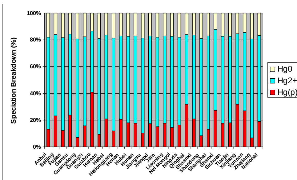
Figure 2.8 - Speciation of mercury emitted from coal combustion in 1999, by province.
