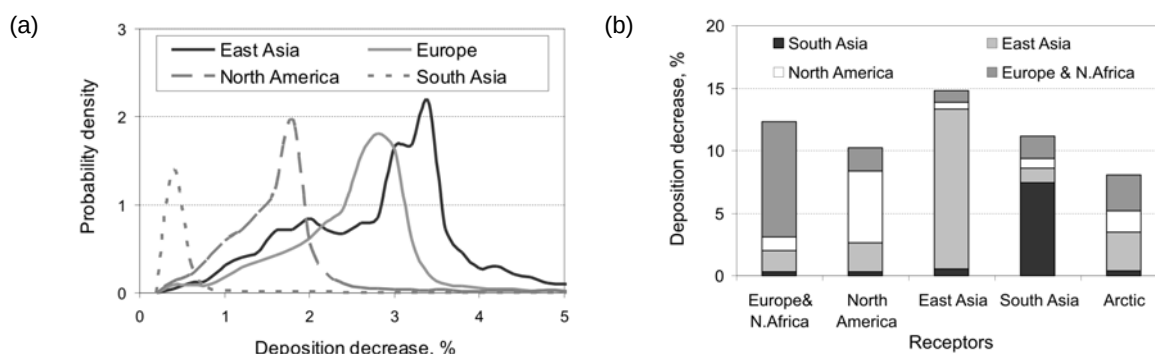
Figure 20.9 - Probability distribution of mercury deposition decrease over the Northern Hemisphere due to 20% emission reduction in the selected source regions (a) and contribution of the source regions to the deposition decrease in different receptor regions (b).
