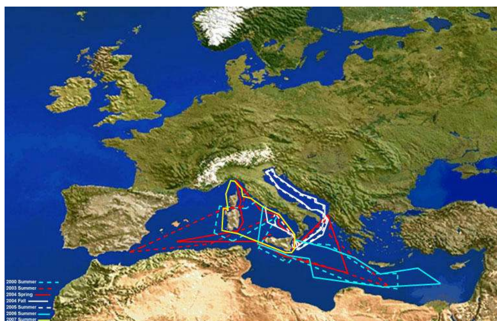
Figure 11.7 -Routes followed during the oceanographic campaigns in the Mediterranean Sea Basin during different seasons and covering two sectors of the Mediterranean (Eastern and Western) from 2000 to 2007.
