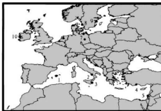
Figure 9.18 - The measurement sites: 1. Mallorca (39°40'30" N, 2°41'36"E); 2. Calabria (39°25'N, 16°00'E); 3. Sicily (36°40'N, 15°10'E); 4. Turkey (36°28'12"N, 30°20'24"E); 5. Israel (32°40'N, 34°56'E); 6. Germany (53°08'34"N, 13°02'00"); 7. Germany (54°26'14"N, 12°43'30"E); 8. Sweden (57°24'48"N, 11°56'06"E); 9. Sweden (58°48'00", 17°22'54"E); 10. Ireland (53°20'N, 9°54'W)
