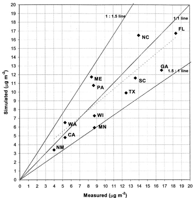
Figure 16.4 - Comparison of simulated and measured 1998 wet deposition fluxes ( \mu\text{g m}^{-2} ) of total mercury over the United States (CA, California; FL, Florida; GA, Georgia; ME, Maine; MN, Minnesota; NC, North Carolina; NM, New Mexico; PA, Pennsylvania; SC, South Carolina; TX, Texas; WA, Washington; WI, Wisconsin).
