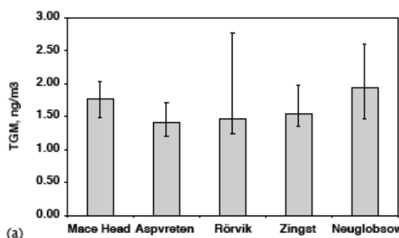
Figure 9.15 - Regional differences of TGM concentrations measured during the MOE project (Munthe et al., 2003).
