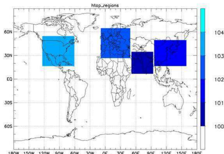
Figure 21.3 - UNEP source areas used in the global emission scenarios.
