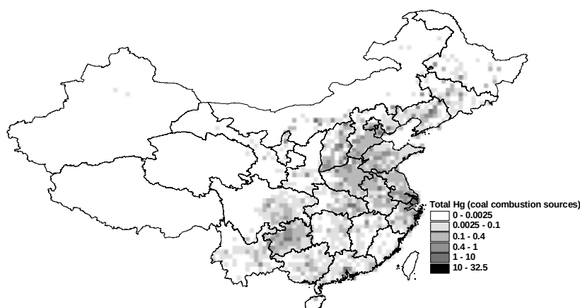
Figure 2.9 - Gridded mercury emissions from coal combustion for the year 1999 at 30 min × 30 min spatial resolution (units are Mg yr -1 per grid cell).
