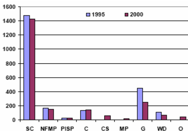
Figure 1.3 - Global mercury emissions to the atmosphere by source category in 1995 and 2000 (based on Pacyna et al., 2003; Pacyna et al., 2006b).
