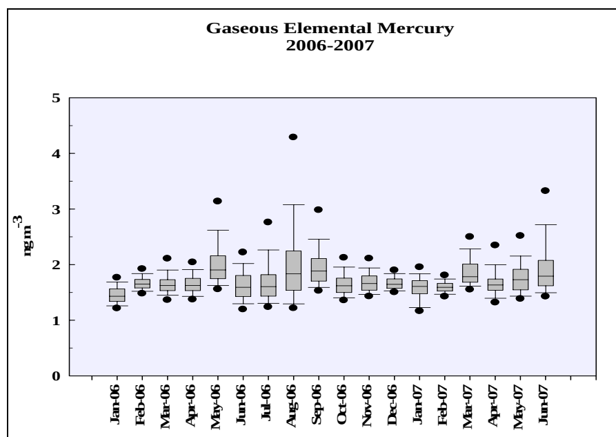
Figure 9.2 - Monthly Box-whisker plot trends of Gaseous Elemental Mercury from 2006 and 2007 at Halifax (Nova Scotia, Canada).
