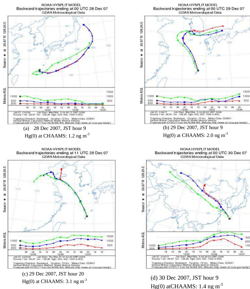
Figure 12.4 – NOAA HYSPLIT backward trajectory for Episode #3 Japanese Standard Time (JST) = Coordinate Universal Time (UTC) + 9 hours.
