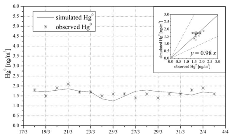
Figure 13.11 - The measured and calculated \text{Hg}^0_{(\text{g})} concentration during the Med-Oceanor 2004 oceanographic campaign. (Hedgecock et al. 2006).
