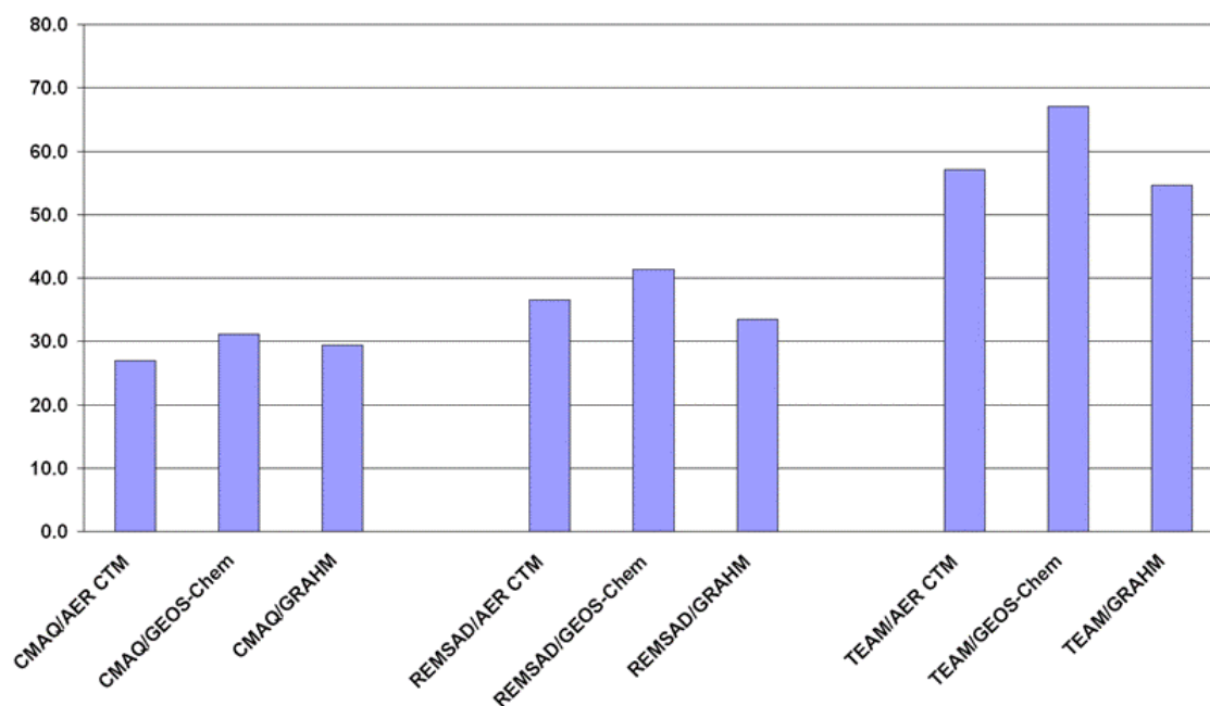
Figure 16.10 - Mean fractional error (percent) for simulated annual Hg wet deposition compared to observed values for each of the regional model simulations conducted in the North American Mercury Model Intercomparison Study.
