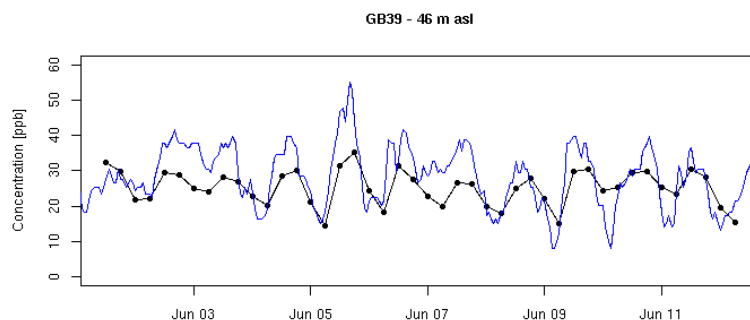
Figure 19.6 - Simulated O 3 concentrations [ppb] versus observations, June 2001.
