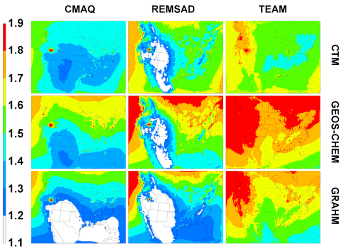
Figure 13.2 - Simulated annual surface-level \text{Hg}^0 (nanograms per cubic meter of standard air) from three regional-scale models (CMAQ, REMSAD, TEAM) for North America using results from three different global models (CTM, GEOS-CHEM and GRAHM) as boundary conditions. From Bullock et al. (2007).
