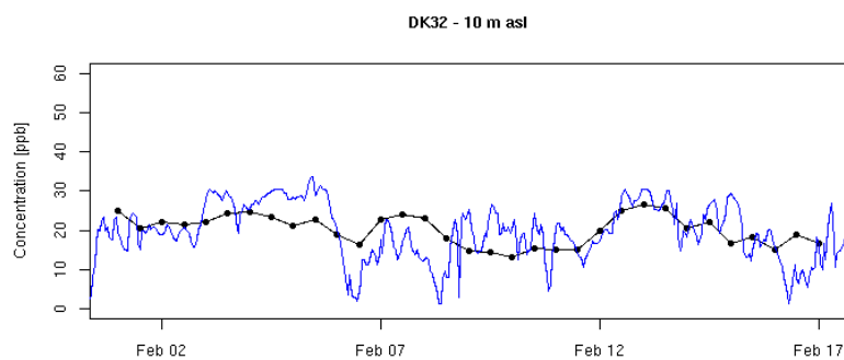
Figure 19.5 - Simulated O 3 concentrations [ppb] versus observations, February 2001.
