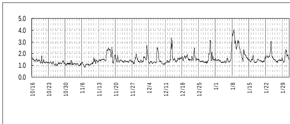
Figure 12.2 - Observation of gaseous elemental Hg(0) at CHAAMS from October 2007 to January 2008
