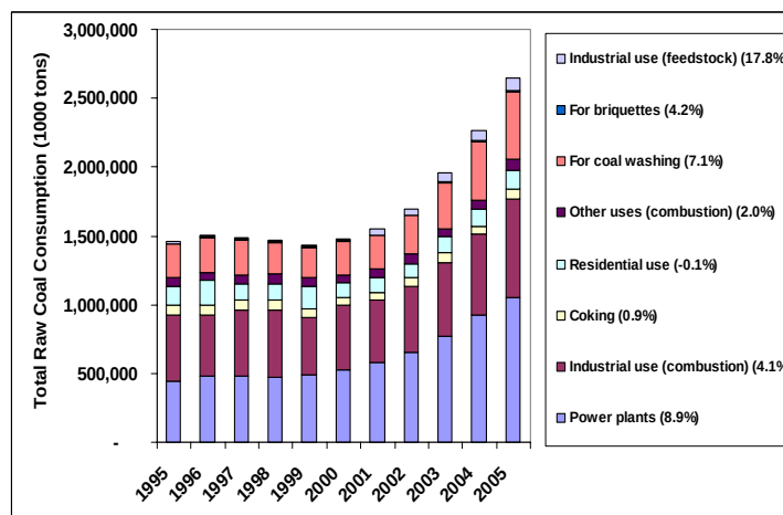
Figure 2.1 - Trends in total raw coal consumption in China, 1995-2005; annual-average growth rates for the entire period are shown in the caption.
