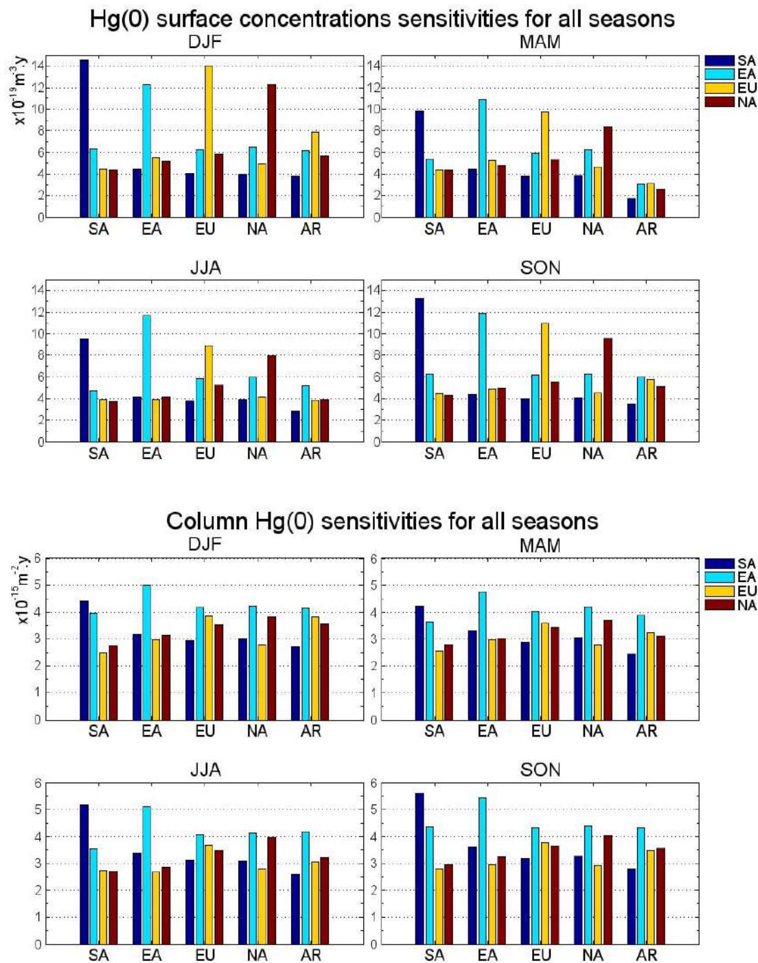
Figure 17.4 - The surface air GEM concentration (top) and column GEM burden (bottom) sensitivities at receptor regions (x axis) and the Arctic to unit emission reductions from the source regions defined as South Asia (SA), East Asia (EA), Europe and North Africa (EU) and North America (NA).
