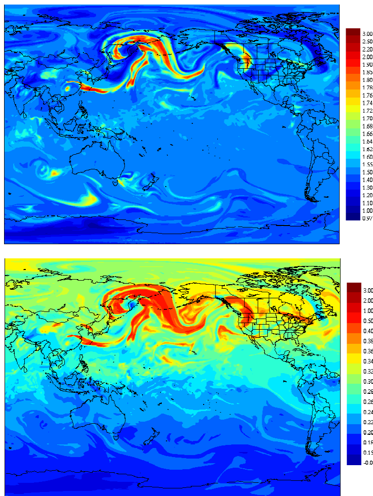
Figure 17.6 - GRAHM air concentrations of mercury (ng/standard m3) on 18Z April 25, 2004 at 500mb showing episode of Asian outflow of mercury reaching N. America which was observed at Mt. Bachelor in central Oregon. The top panel shows simulation from all emissions and the bottom panel shows simulation from anthropogenic Asian emissions.
