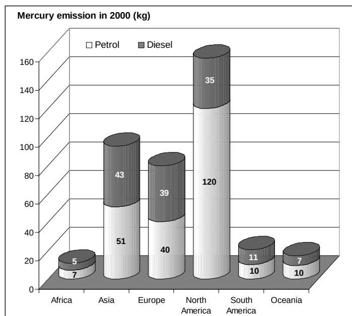
Figure 1.4 - Global mercury emissions to the atmosphere by petrol and diesel consumption in 2000.
