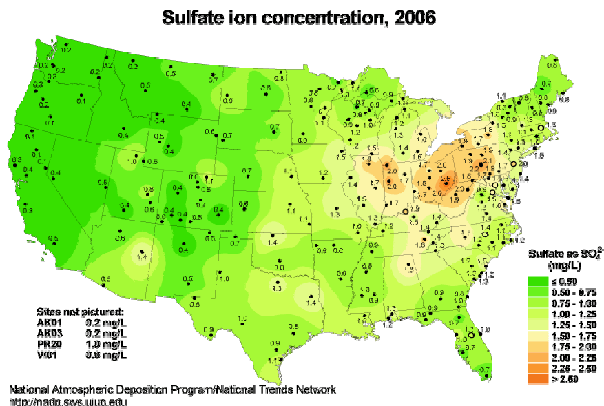
Figure 9.9 - Sulfate concentration from the National Trends Network in 2006.
