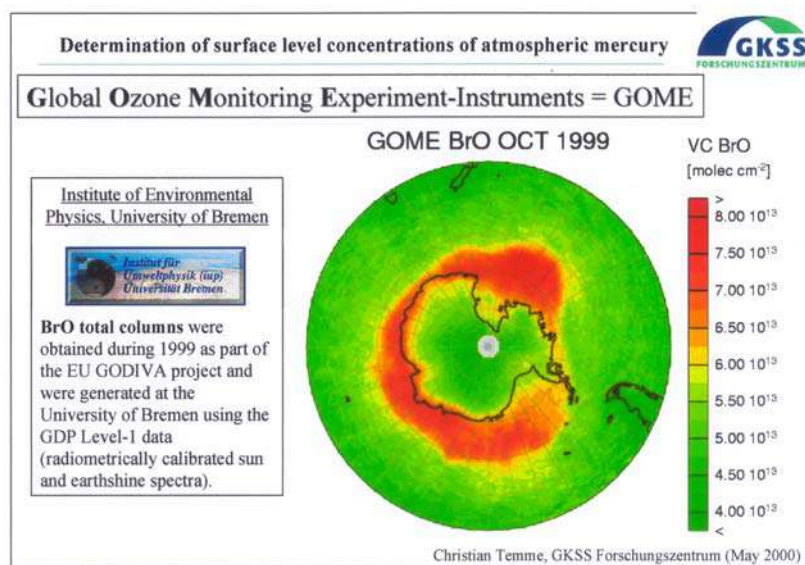
Figure 10.4 - Distribution of BrO around the Antarctic Continent (Richter et al., 2002).
