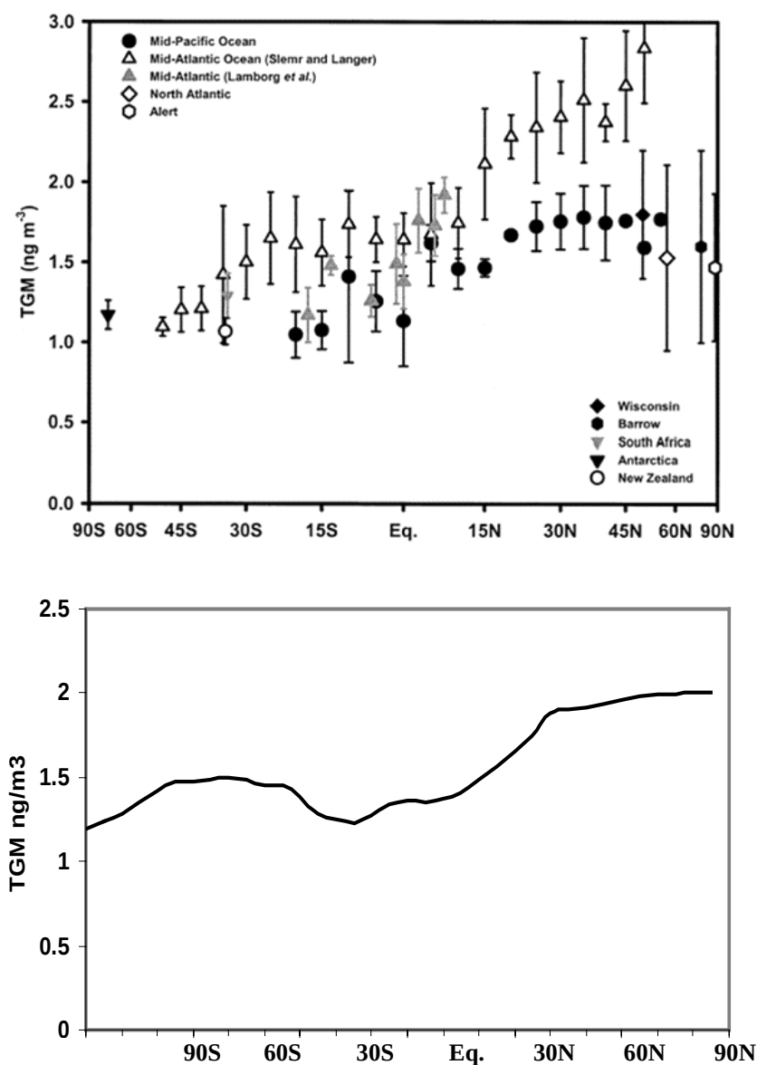
Figure 17.1 - Inter-hemispheric gradient of TGM from observations (top: Lamborg et al. (2002)) and GRAHM model simulation (bottom).
