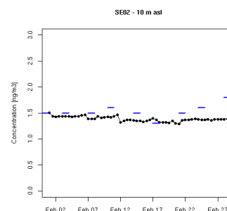
Figure 19.7 - Simulated TGM concentrations [ng/m 3 ] versus observations, February 2001.
