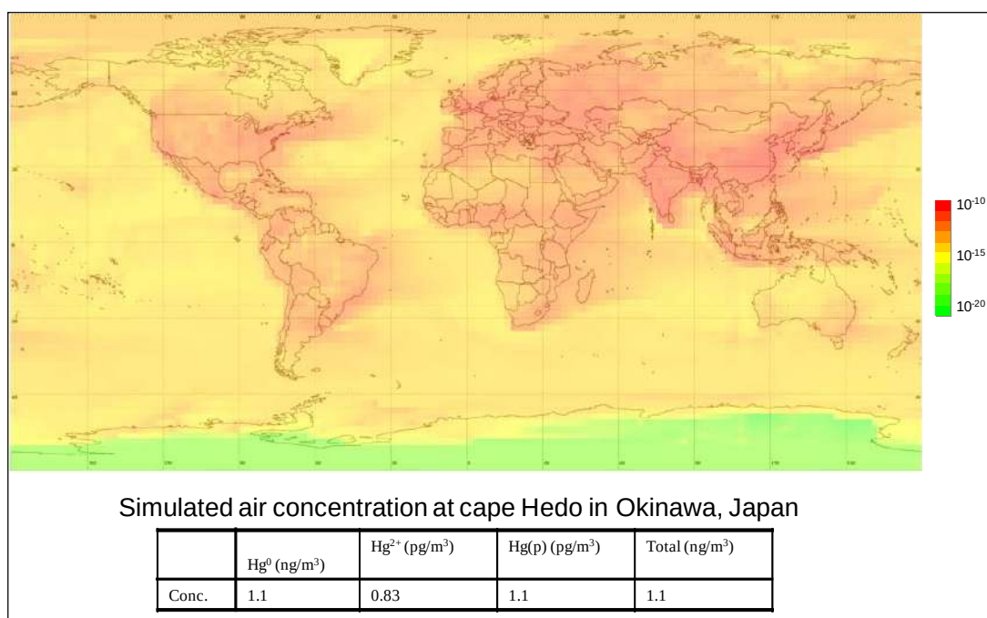
Figure 12.7 - Preliminary results of atmospheric concentration and comparison to the simulated air concentration at the Cape Hedo location.
