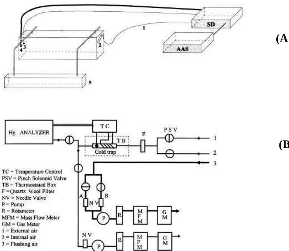
Figure 11.9 - (A) Floating flux chamber. 1) Teflon tube for external air sampling; 2) inlet port; 3) and 4), outlet ports; 5) floating PVC foam bar the second floating bar is not shown in the figure.; AAS, atomic absorption spectrometer; SD, sampling device; (B) Semi-automatic air sampling device for measurements of mercury degassing rate.
