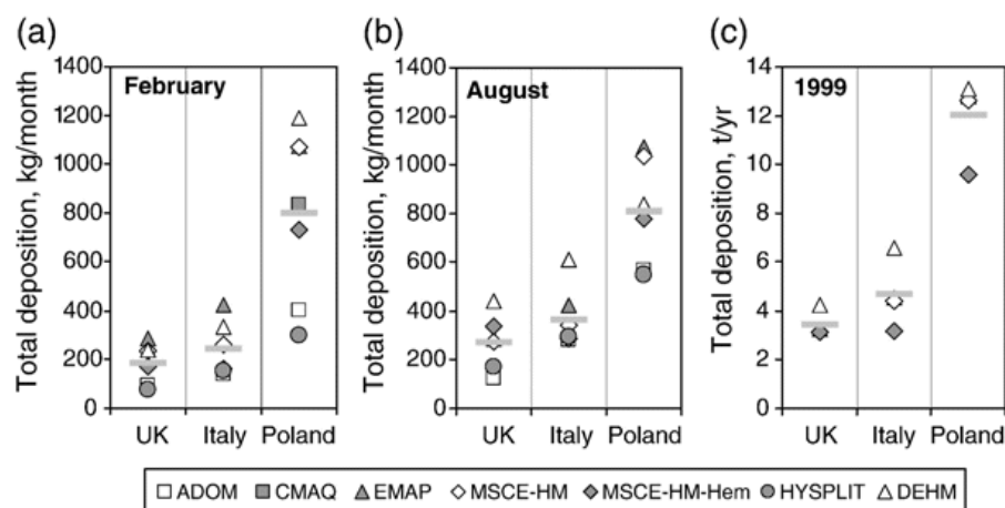
Figure 16.1 - Total Hg deposition to the UK, Italy and Poland: (a) in February 1999; (b) in August 1999; and (c) in the whole year 1999. Symbols depict modelling results, light grey dashes show the ensemble average.
