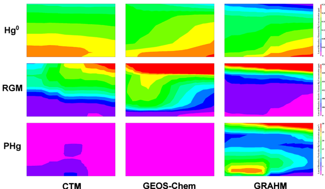
Figure 13.7 - Annual Average Western Boundary Values for the three mercury species determined by the three Global Mercury Models for the NAMMIS.
