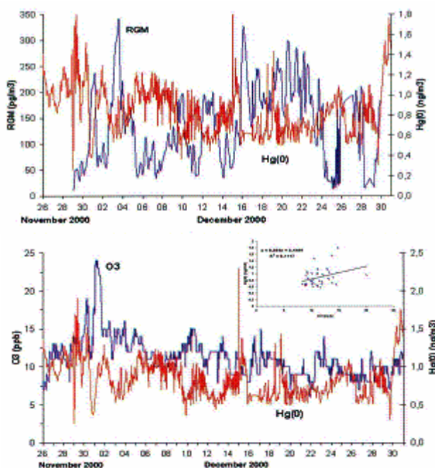
Figure 10.6 - Two-hourly mean concentrations of GEM and RGM measured at Terra Nova Bay, Antarctica from November to December, 2000 (Source: Sprovieri et al., 2002).
