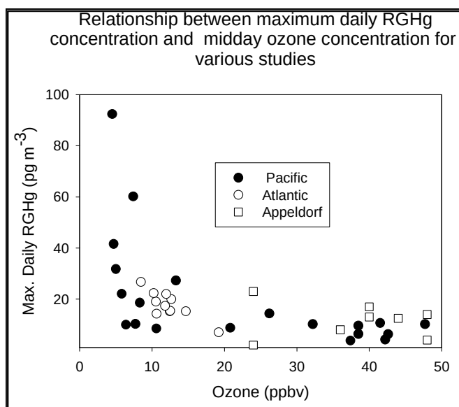
Figure 11.5 - Relationship between the maximum measured daily reactive gaseous mercury concentration (2 hr average) and the midday ozone concentration from a number of different measurements over the ocean. Taken from Laurier and Mason (2007).
