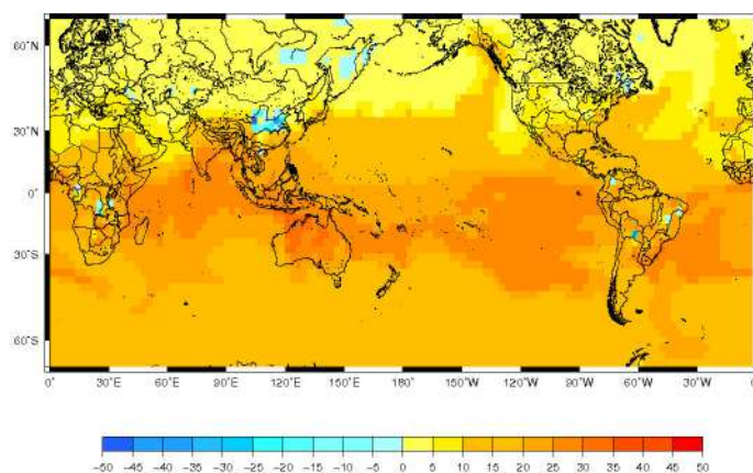
Figure 19.1 - Difference [ppq] in \text{Hg}^0 concentrations between a run excluding and one including the reaction of OH with \text{Hg}^0 , both using the \text{Hg}+\text{O}_3 reaction rate constant of Hall (1995).
