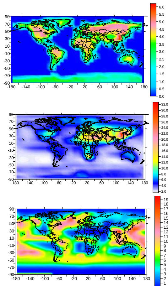
Figure 21.2 - Atmospheric deposition of mercury (µg/m²-y) in the base simulation: Top: Hg(0) dry deposition; middle: Hg(II) dry deposition; bottom: Hg(II) wet deposition.
