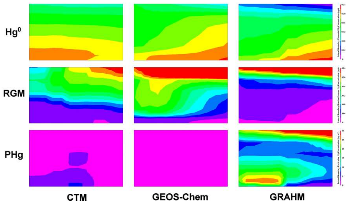
Figure 16.7 - Annual average air concentrations of Hg^0 , RGM and particulate Hg (PHg) across the western boundary of the NAMMIS regional domain as determined from the CTM, GEOS-Chem and GRAHM global simulations.
