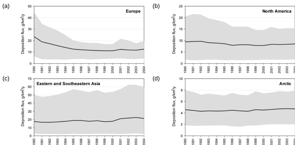
Figure 20.4 - Long-term changes of mercury deposition flux in Europe (a), North America (b), Eastern and Southeastern Asia (c), and in the Arctic (d). Solid line presents average flux over the region; shaded area shows 90%-confidence interval of the flux variation over the region.
