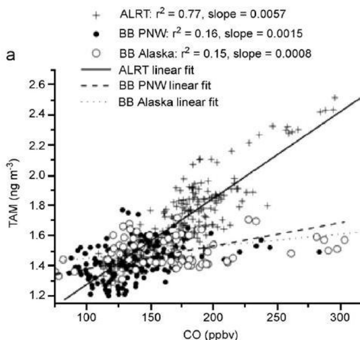
Figure 9.13 - Scatter plot of total airborne mercury (TAM) vs. CO measured during 22 pollution events at Mt. Bachelor Observatory, Oregon during 2004-2005. The events are categorized as Asian long-range transport (ALRT), and biomass burning from Alaska or the Pacific Northwest (Weiss-Penzias et al., 2007).
