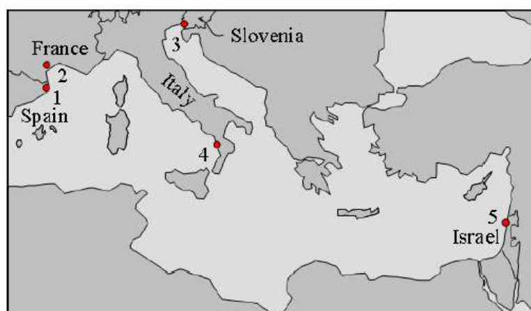
Figure 9.22 - MERCYMS coastal measurement sites.
