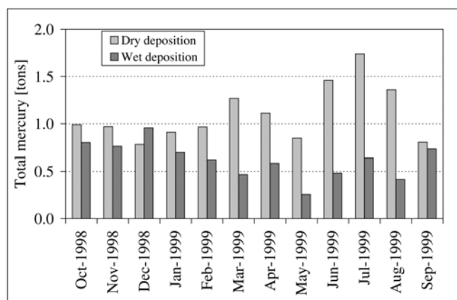
Figure 13.10 - Calculated monthly dry and wet deposition to the surface of the Mediterranean Sea during the MAMCS campaign. (Hedgecock et al. 2006).
