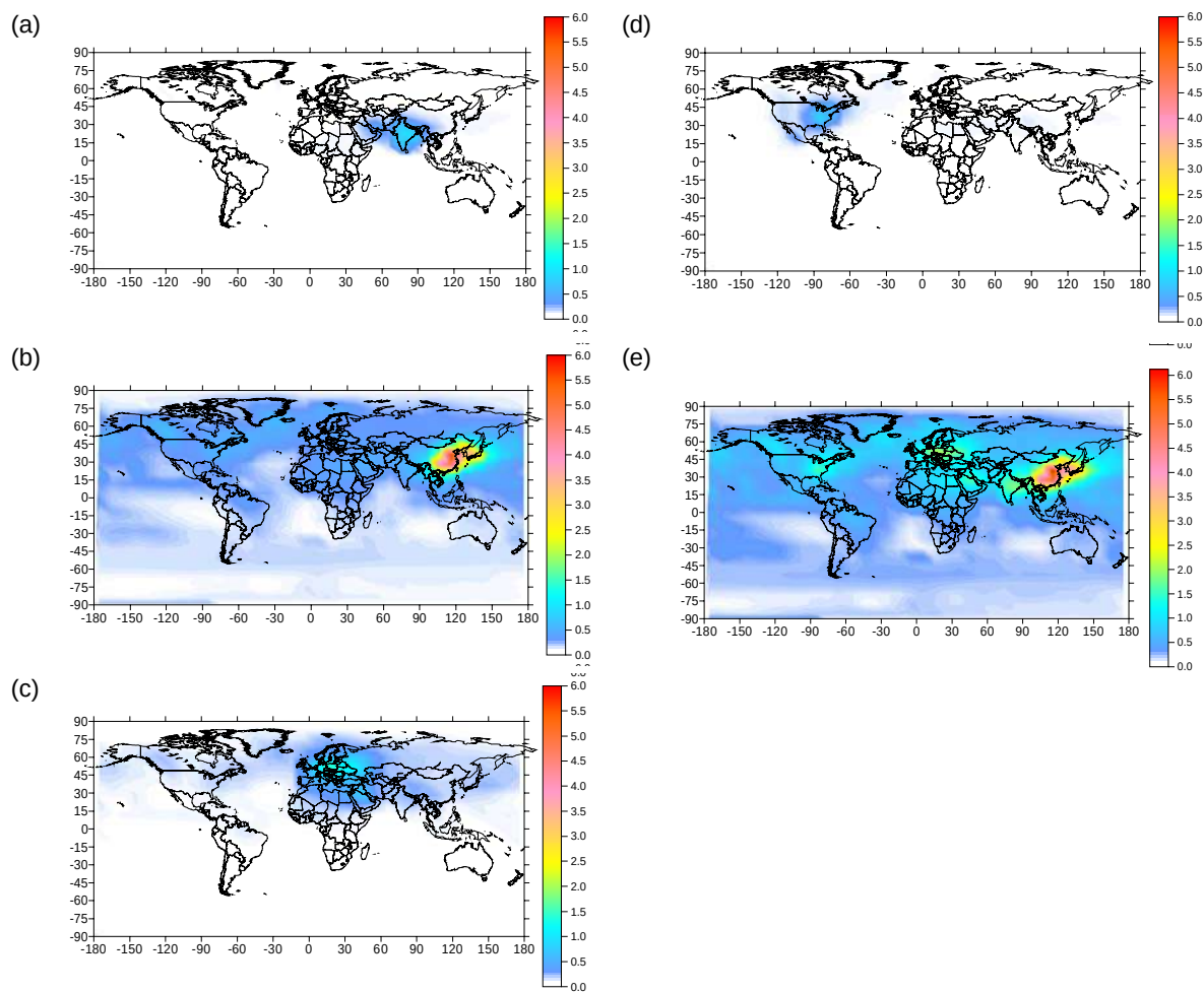
Figure 21.4 - Contribution of 20% of anthropogenic emissions from a region to total atmospheric mercury deposition ( \mu\text{g m}^{-2} \text{y}^{-1} ): (a) South Asia, (b) East Asia, (c) Europe and North Africa, (d) North America, (e) all four regions.
