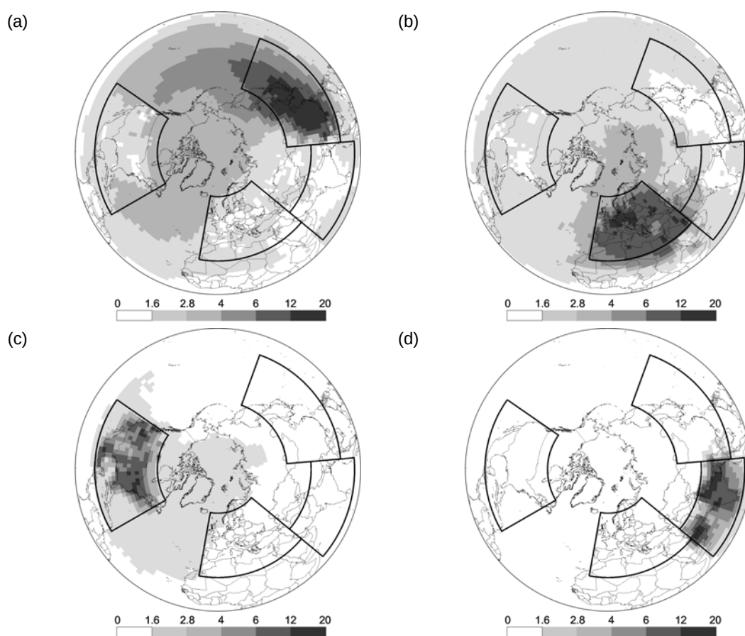
Figure 20.8 - Spatial distribution of relative decrease of mercury deposition due to 20% emission reduction in East Asia (a), Europe (b), North America (c), and South Asia (d).
