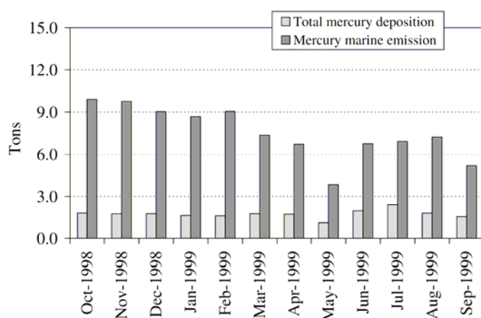
Figure 1.2 - Modeled monthly total emission and deposition fluxes to the Mediterranean Sea (from Hedgecock et al., 2006).
