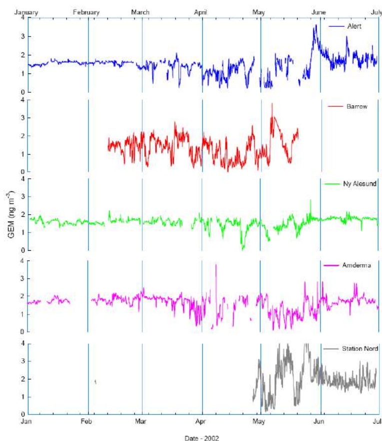
Figure 10.2 - Temporal trends of GEM measurements conducted in the Arctic in 2002.
