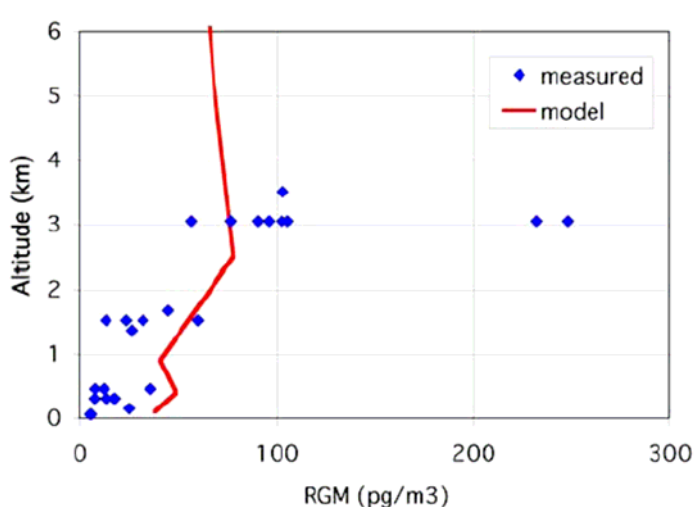
Figure 13.8 - Measured RGM ( \text{pg m}^{-3} ) versus altitude (km) from aircraft measurements over the Atlantic Ocean off the coast of south Florida during June 2000 (points). The line represents model RGM versus altitude, based on an average of model results during the afternoon on the 5 d (9, 12, 14, 25 and 26 June) that coincide with measurements. (After Sillman et al. 2007).
