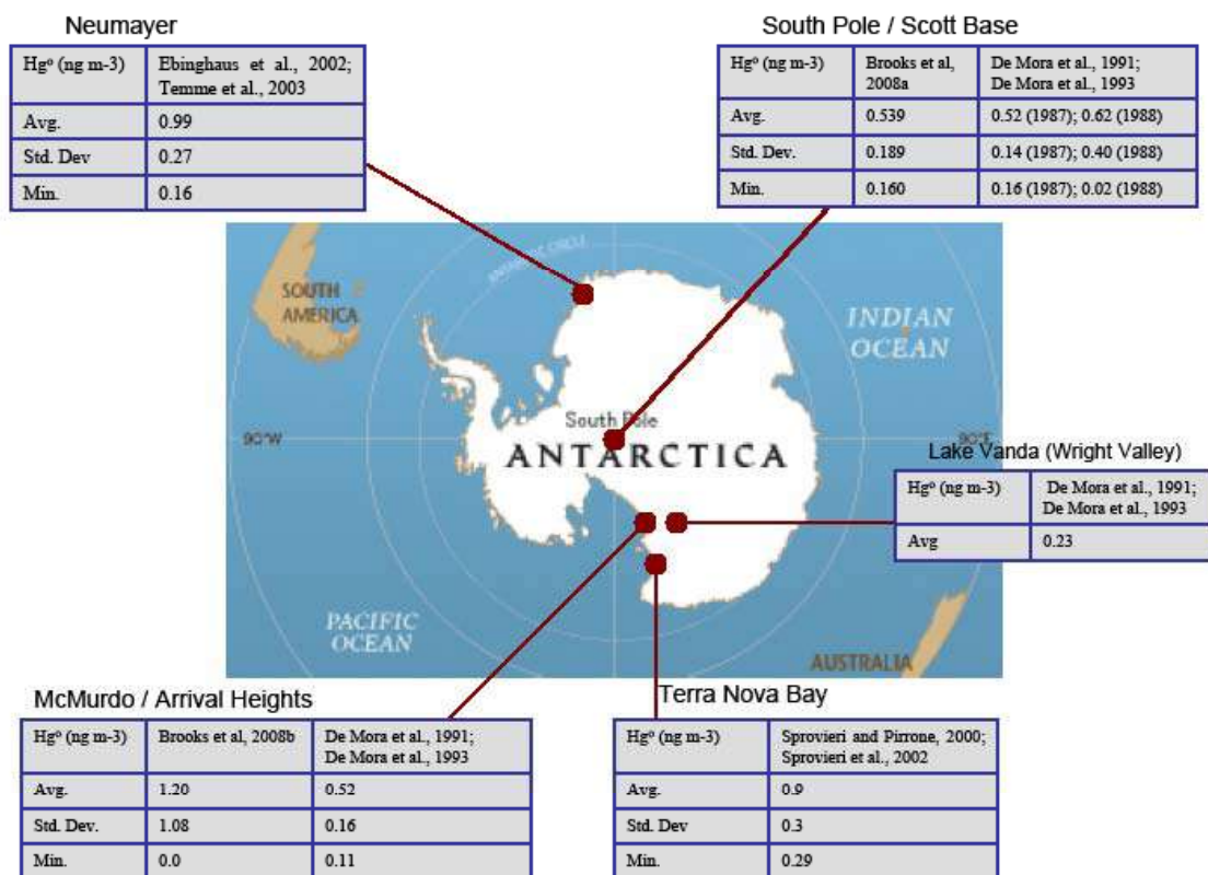
Figure 10.3 - Measurement sites for atmospheric mercury in Antarctica.
