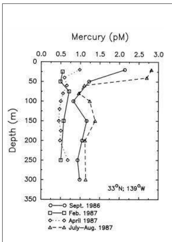
Figure 11.15 - Concentrations of reactive mercury measured at the VERTEX site over a season in 1986/87 showing the changes in the concentrations in the upper waters over time. Taken from Laurier et al. (2004).
