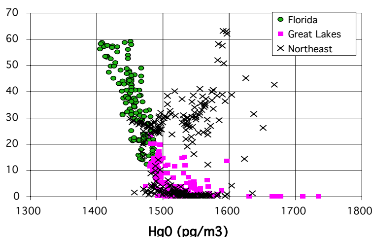
Figure 13.5 - Model correlation between Hg^0 and RGM in pg\ m^{-3} for Florida (green circles), the northeast corridor (X's) and Great Lakes (pink squares). Negative correlations identify photochemical production of RGM from global background Hg^0 . Positive correlations identify directly emitted RGM and Hg^0 . (From Sillman et al., 2007).
