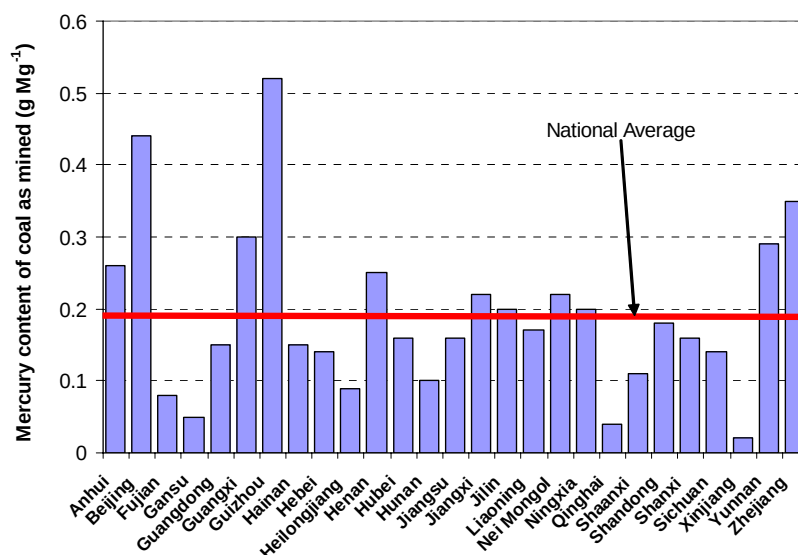
Figure 2.3 - Mercury content of raw coal, as mined, \text{g Mg}^{-1} .
