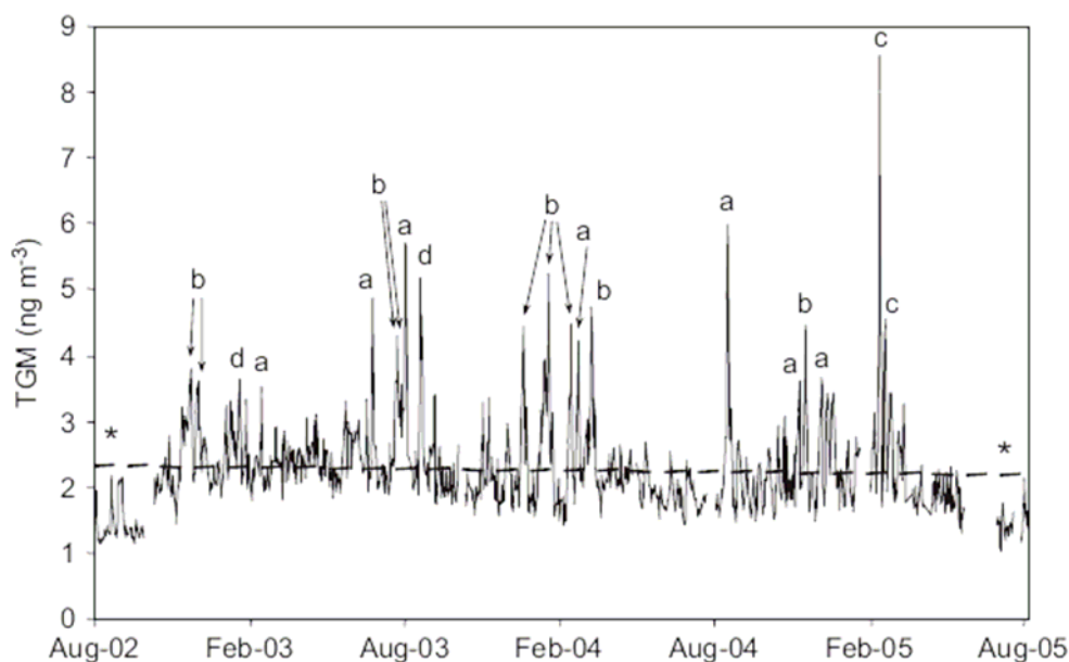
Figure 9.6 - Time series plot of average daily concentrations of TGM measured at Desert Research Institute (Reno, Nevada) from 2002 to 2005. Fitted trend equation for all data: y = 2.3 - 0.00013t (in days). Letters indicate potential sources/causes of elevated TGM (a) following precipitation), atmospheric signature of pollution plumes (b), elevated NO x , CO or PM 10 concentrations), marked change in meteorological conditions (c), change in barometric pressure), or no specific indicator (d). Asterisks denote periods of unusually low TGM (Stamenkovic et al., 2005).
