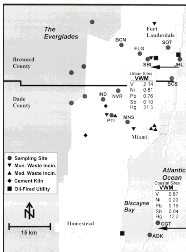
Figure. 13.3 - Volume-weighted mean concentrations of V, Ni, Pb, and Sb ( \mu\text{g L}^{-1} ) and Hg ( \text{ng L}^{-1} ) in precipitation arriving from the east at SoFAMMS urban (BCN, BCS, FLG, IND, MNS, NVR, PTI, SBI, and SOT) and coastal (ADK, CGT, and JHL) sites. (After Dvonch et al. 2006).
