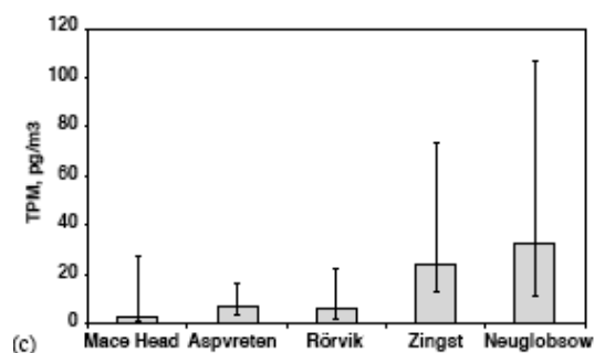
Figure 9.16 - Regional differences of TPM concentrations measured during the MOE project (Munthe et al., 2003).
