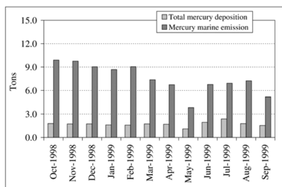
Figure 13.9 - Calculated monthly total deposition and evasion of mercury to and from the surface of the Mediterranean Sea during the MAMCS campaign. (Hedgecock et al. 2006).
