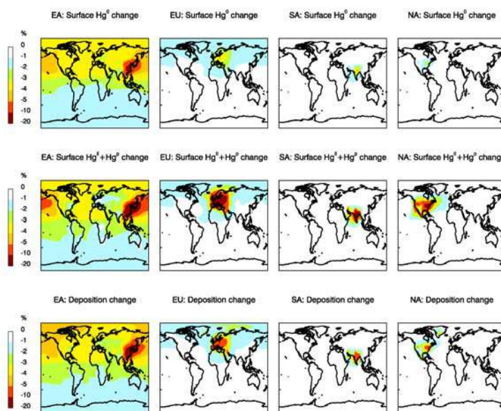
Figure 18.3 - Percentage change in annual surface concentrations of \text{Hg}^0 and \text{Hg}^{\text{II}} + \text{Hg}^{\text{p}} (top 2 rows) and in deposition (bottom row) for each perturbation simulation. The perturbation simulations are shown from left to right: East Asia (EA), Europe and North Africa (EU), South Asia (SA), and North America (NA).
