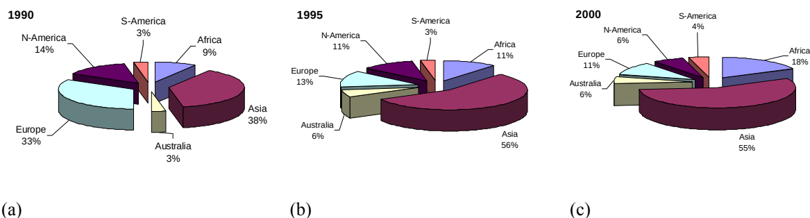
Figure 1.7 - Trend of global anthropogenic emissions by region (based on Pirrone et al., 1996 (a); Pacyna et al., 2003 (b); Pacyna et al., 2006b (c)).
