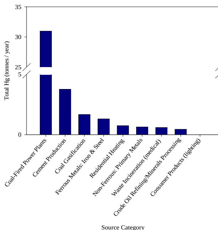
Figure 5.3 - Average atmospheric Hg emissions estimated for different source categories in South Africa during 2004.
