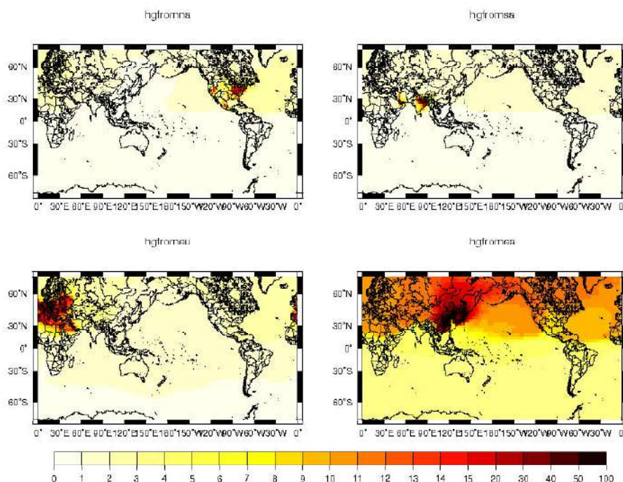
Figure 19.11- Hg-like tracer (lifetime 360 days) for 4 different source regions, concentration [ppq] in surface layer, July 2001.
