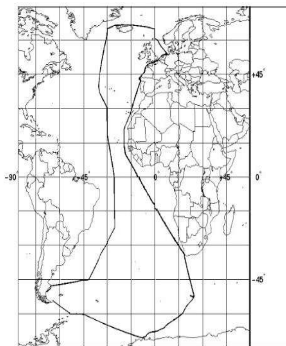
Figure 11.2 - Tracks of the Polarstern cruises from Bremerhaven to Punta Quilla (Argentina) in 1996, from Bremerhaven over Cape Town (South Africa) to Antarctica in 1999–2000, and from Antarctica to Punta Arenas (Chile) in 2001.
