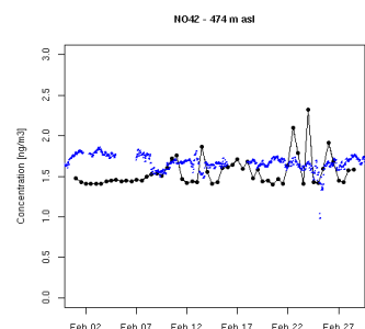
Figure 19.7 - Simulated TGM concentrations [ng/m 3 ] versus observations, February 2001.
