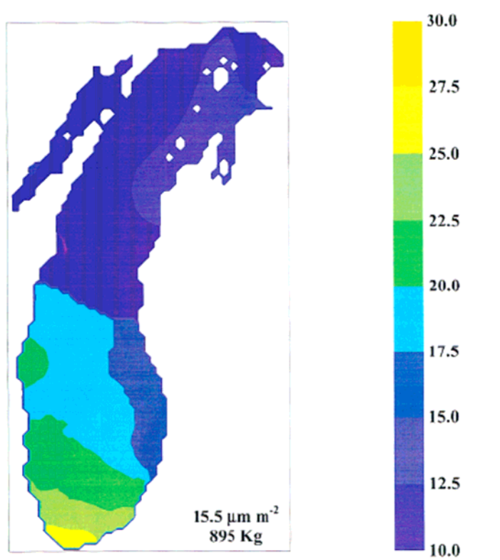
Figure 9.11 - Estimated over-water wet deposition flux (July 1, 1994-October 31, 1995) (Landis and Keeler, 2002). The annual mean wet deposition value and total Hg deposited to the lake during the study period is shown at the bottom of the figure.
