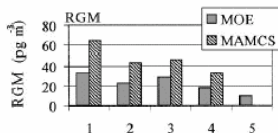
Figure 9.21 - Average TGM, IPM and RGM values obtained at campaign MOE 1-5 and MAMCS 1-4. The IGM value from the MAMCS campaign 4 should be regarded with some caution since it is based on measurements from two sites only.
