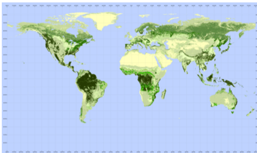
Figure 8.1 - Olson's major world ecosystem complexes ranked by carbon in live vegetation: An updated database using the GLC2000 land cover product (cdiac.ornl.gov).
