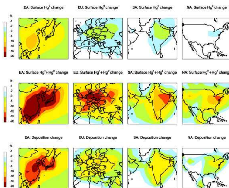
Figure 18.4 - Same as Figure 18.3, but focusing on the source regions where anthropogenic emissions are reduced by 20%
