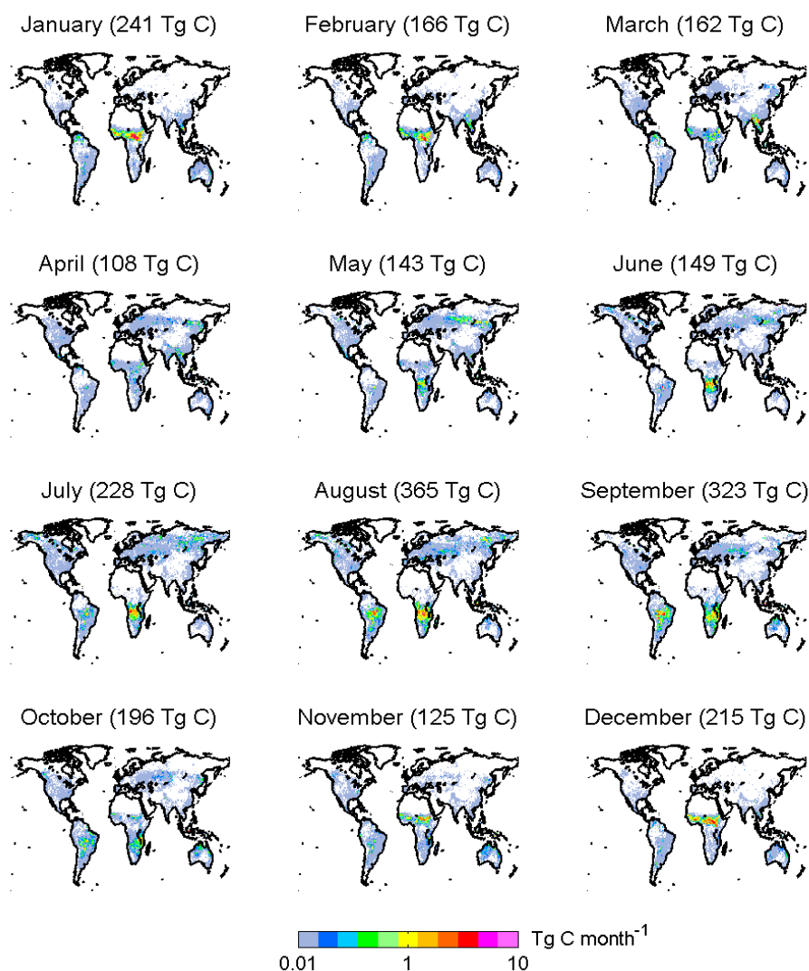
Figure 8.2 - Average monthly carbon emissions for the period 1997-2006.
