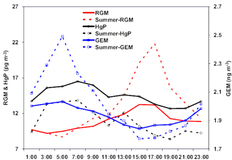
Figure 9.12 - Diurnal variation of Hg species (median concentrations) in Detroit (2003) (Liu et al., 2007) Note the inverse relationship between RGM and Hg(0) . Hgp has the least amount of diel variability.
