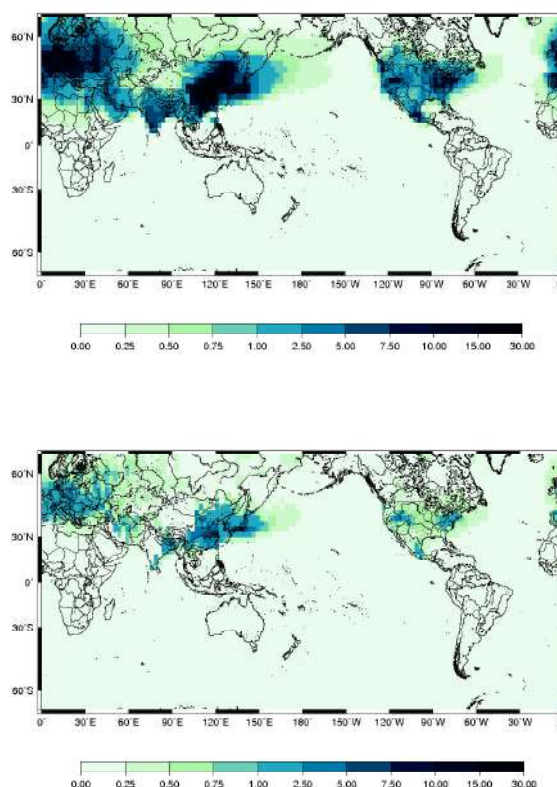
Figure 19.16 - Changes (control run minus reduction experiment) in wet (below) and dry (up) deposition due to a 20% emission reduction in all 4 source regions, Jan-Mar 2001.
