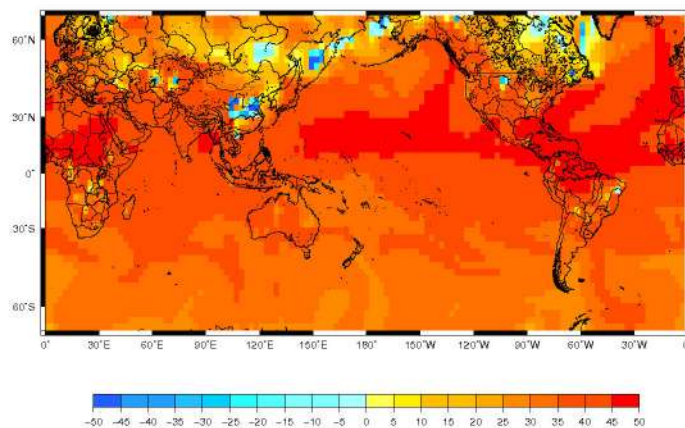
Figure 19.2 - Difference [ppq] in \text{Hg}^0 concentrations between a run including the \text{Hg}+\text{O}_3 reaction rate constant of Hall (1995) and excluding the OH reaction and one run including OH reaction and using the \text{Hg}+\text{O}_3 reaction rate constant of Pal and Ariya (2004)
