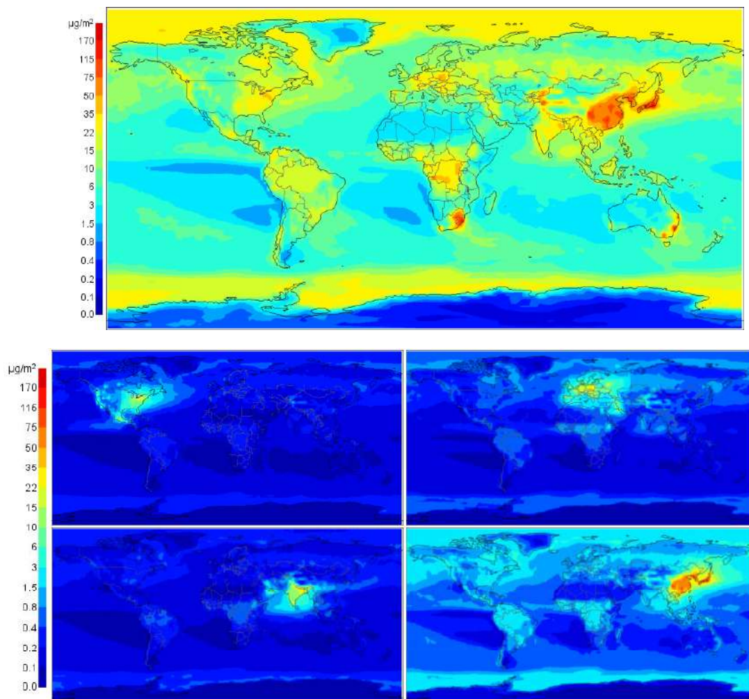
Figure 17.3 - Total mercury deposition for year 2001 from reference simulation (top) and reduction in deposition due to 20% reduction in anthropogenic emissions (scaled to 100% in the figure) from North America (middle left), Europe and North Africa (middle right), South Asia (bottom left) and East Asia (bottom right).
