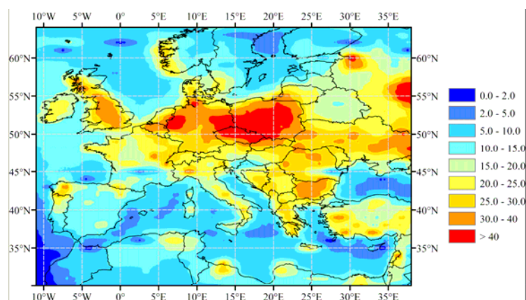
Figure 1.1 - Modeled annual total deposition flux in g km -2 (equivalent to mg m -2 ) over the modeling domain (from Hedgecock et al., 2006).
