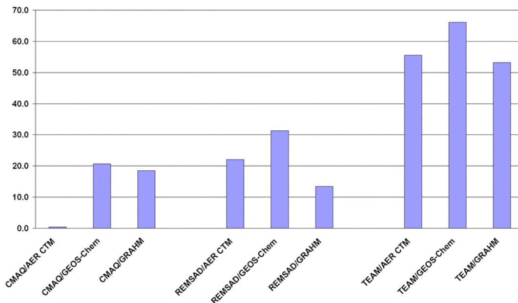
Figure 16.9 - Mean fractional bias (percent) for simulated annual Hg wet deposition compared to observed values for each of the regional model simulations conducted in the North American Mercury Model Intercomparison Study.
