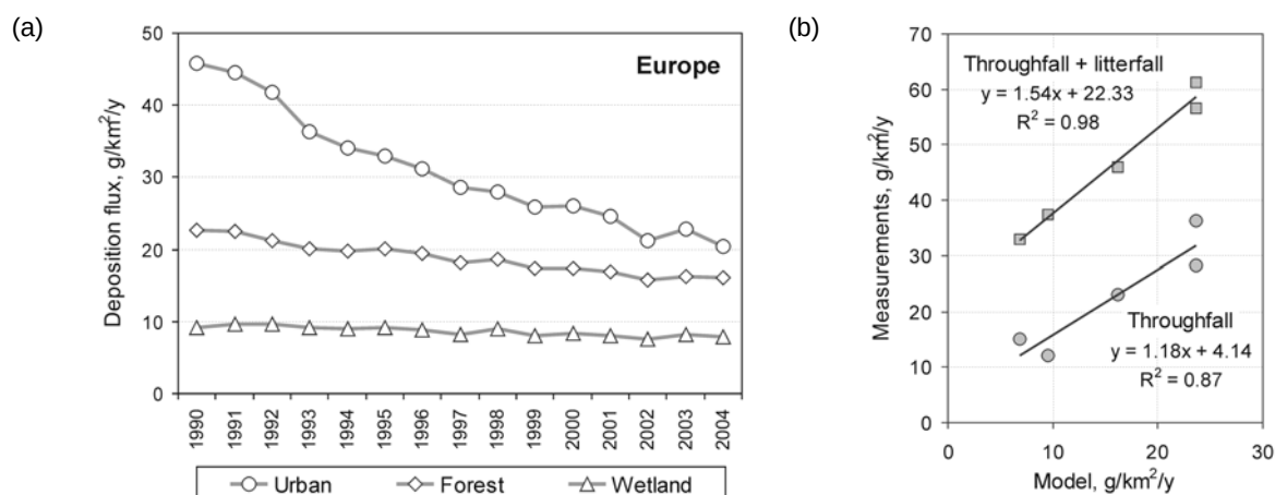
Figure 20.5 - Long-term changes of mercury deposition flux to different landuse categories in Europe (a) and comparison of calculated mercury deposition to forests with throughfall measurements at forest sites in Europe (b).
