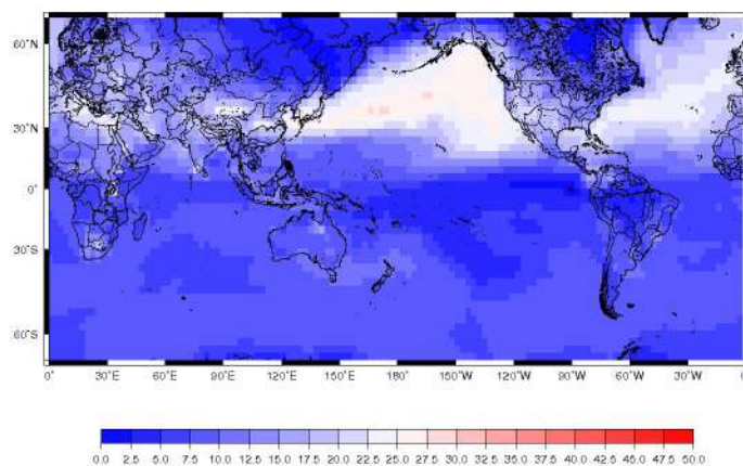
Figure 19.3 - Monthly mean ozone concentration [ppb], January 2001.
