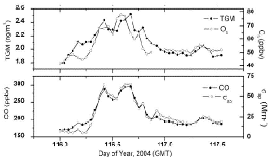
Figure 13.4 - Measured O_3 , CO, particulate scattering ( \sigma_{sp} ) and total gaseous mercury (TGM) during a pollution transport event at Mt. Bachelor, Oregon. Simultaneous elevated concentrations is interpreted as evidence of transport, most likely from Asia. (From Weiss-Penzias et al., 2006).
