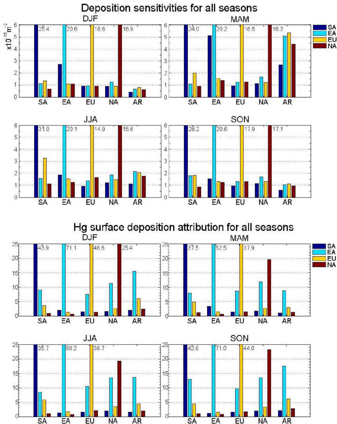
Figure 17.5 - Mercury deposition sensitivities at receptor regions and the Arctic to unit emission reductions from the source regions defined as South Asia (SA), East Asia (EA), Europe and North Africa (EU) and North America (NA) (top). Percentage change in mercury deposition at receptor regions and the Arctic from 20% reduction in emissions at the source regions defined as above (the values are scaled to 100% reduction in the figure).
