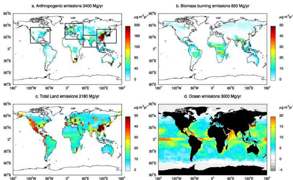
Figure 18.1 - Global distribution of annual emissions ( \mu\text{g m}^{-2} \text{yr}^{-1} ) in the GEOS-Chem model: a) Anthropogenic, b) biomass burning, c) land, and d) ocean emissions. The domains for the four HTAP regions are indicated on panel a).
