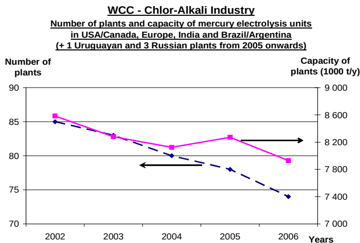
Figure 4.3 - The scenario of world's chlorine plants and production capacity, 2006 (WCC, 2007; Reproduced with permission, Veronique Garny, 2007).
