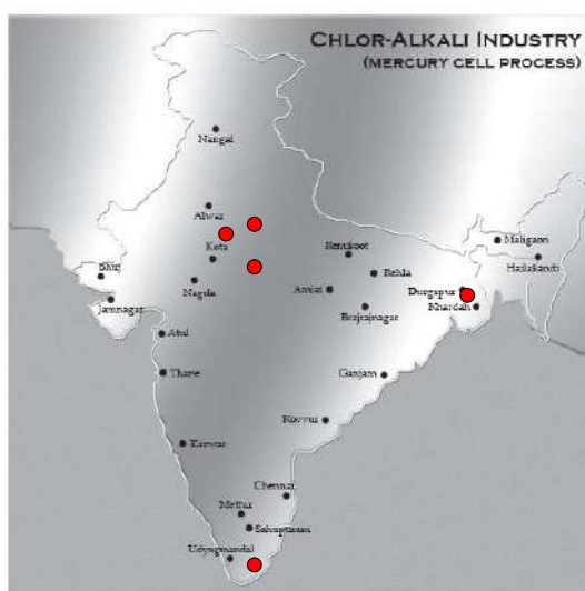
Figure 4.4 - Mercury cell Chlor-alkali industry in India. Red circles indicate Hg-based thermometer industry. Adapted from Toxicslink, New Delhi. See Appendix I which indicates conversion of major number of chlor-alkali plants from Hg-cell to Membrane cell process where no mercury is used http://www.toxicslink.org/docs/06035_publications-1-33-2.pdf .
