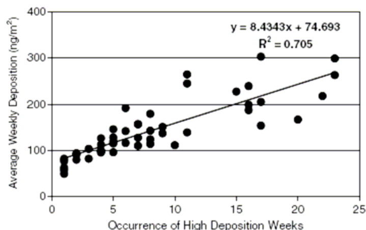
Figure 9.10 - The relationship between the annual occurrence (sum) of high mercury deposition weeks ( >250 \text{ ng m}^{-2} ) and the average annual deposition for those weeks for 13 MDN monitoring sites located in northeast North America (Van Arsdale et al., 2005).
