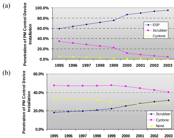
Figure 2.4 - Time development of the penetration of PM control devices in China in (a) the power sector (upper) and (b) the industrial sector (lower), 1995-2003.
