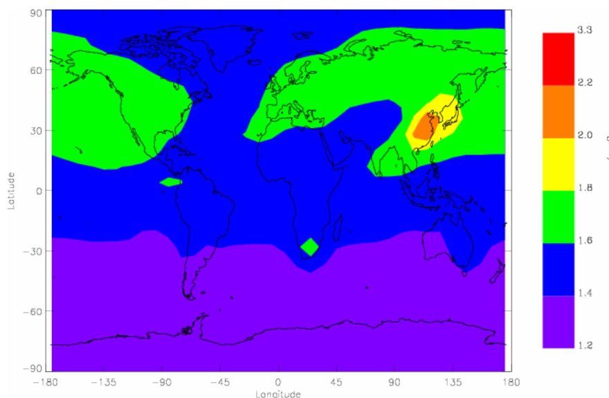
Figure 21.1 - Modeled global Hg(0) concentrations (ng/m 3 ).
