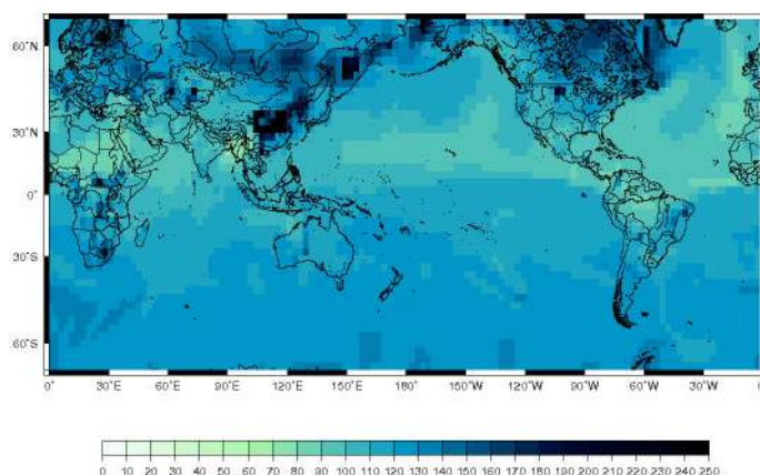
Figure 19.4 - \text{Hg}^0 concentration [ppq] using the \text{Hg}^0 + \text{O}_3 reaction rate of Pal and Ariya (2004) and including the \text{Hg}^0 + \text{OH} reaction.
