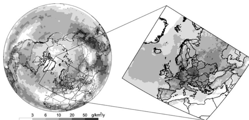
Figure 20.3 - Spatial distribution of total mercury deposition in the Northern Hemisphere and in Europe in 2001.
