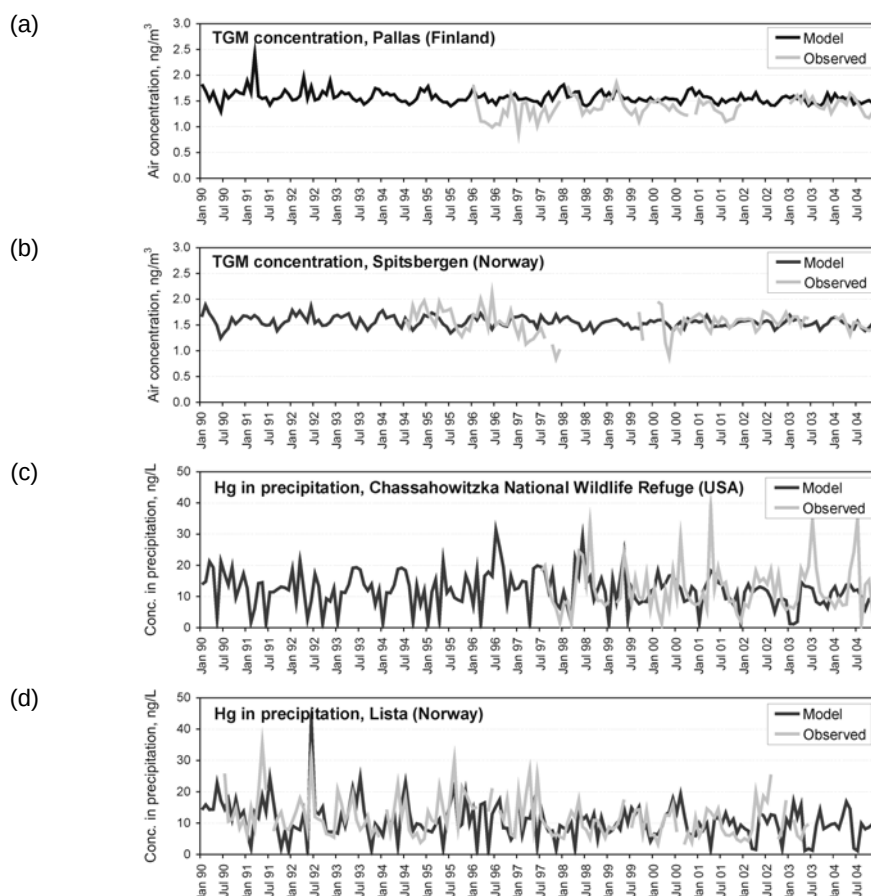
Figure 20.7 - Modelled vs. measured long-term variation of monthly mean total gaseous mercury concentration in air (a, b) and total mercury concentration in precipitation (c, d) at some monitoring sites in Europe (Aas and Breivik, 2006) and North America ( http://nadp.sws.uiuc.edu/mdn/ ).
