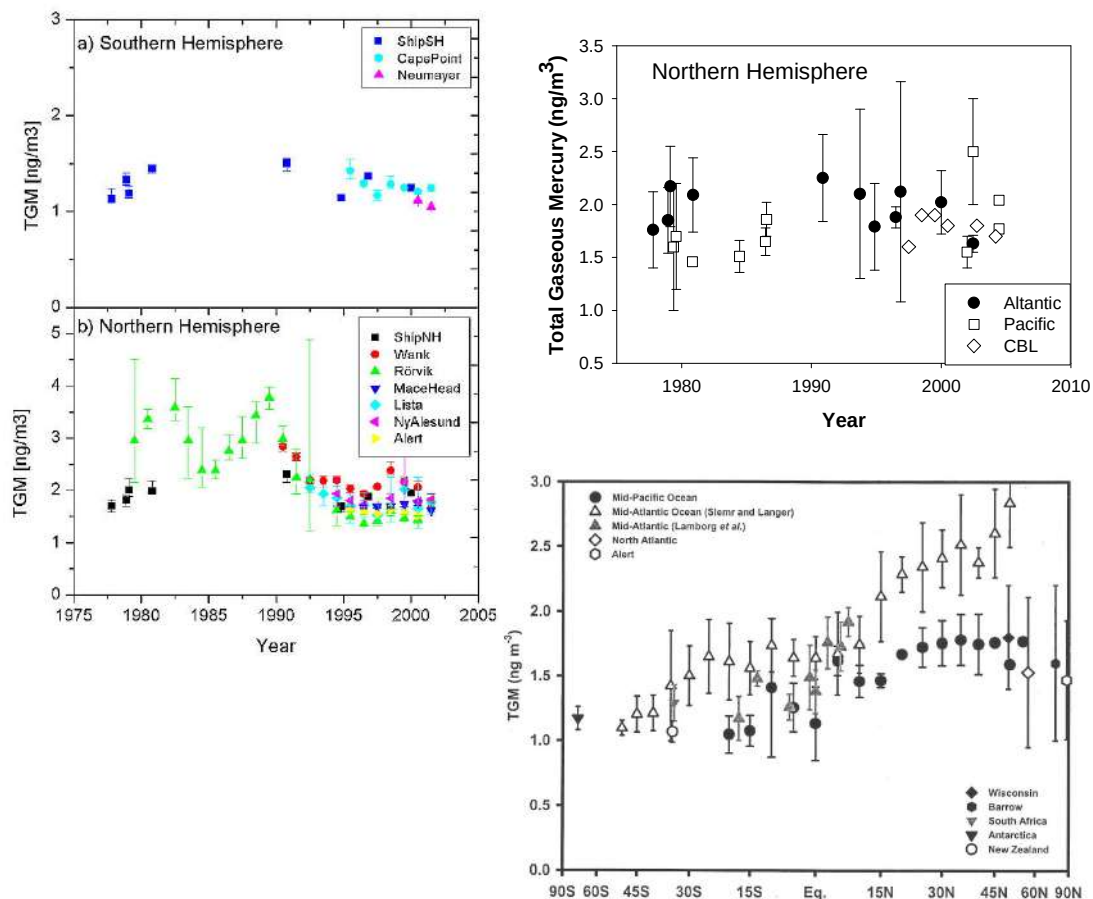
Figure 11.3 - Total Gaseous Mercury concentrations over the ocean and other remote locations as reported by a) Slemr et al. (2003) and b) Laurier and Mason (2007). Both papers are a compilation of data from numerous sources. c) Latitudinal gradient in total gaseous Hg in the atmosphere at several locations. Notice the discernible inter-hemispheric gradient, resulting from greater emissions of Hg to the atmosphere in the more industrialized Northern Hemisphere. Data from Fitzgerald (1995) - Mid-Pacific (filled circles); Slemr and Langer (1992) - Mid-Atlantic (open triangles); Lamborg et al. (1999) - Mid-Atlantic (shaded triangles); Mason et al. (1998) - North Atlantic (open diamonds); Schroeder et al. (1998) - Alert, N.W.T. (open hexagons); Lamborg et al. (1995) - rural Wisconsin, U.S.A. (filled diamonds); Lindberg et al. (2000) - Point Barrow, Alaska, U.S.A. (filled hexagons); Ebinghaus et al. (2000) - Cape Town, R.S.A. (shaded inverted triangles) and Antarctica (filled inverted triangles); Fitzgerald (1989) - Ninety Mile Beach, N.Z. (open circles). Taken from Lamborg et al., (2002).
