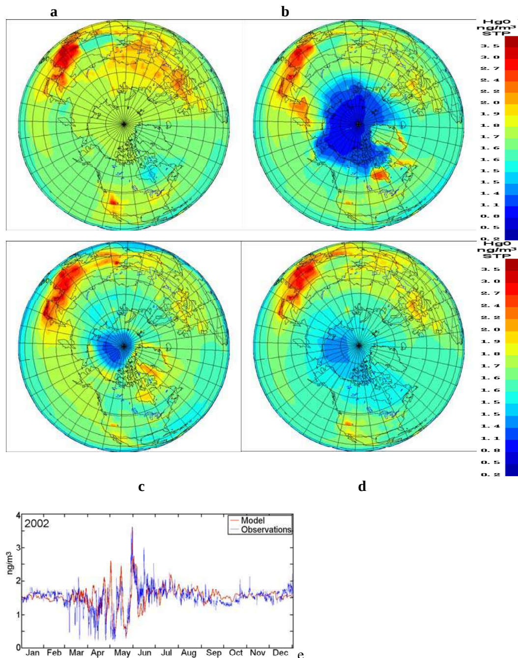
Figure 17.2 - GRAHM simulated average surface air Hg(0) concentrations (ng standard m -3 ) for (a) winter, (b) spring, (c) summer and (d) fall and observed and model simulated time series of surface air Hg(0) concentrations at Alert, Canada for 2002.
