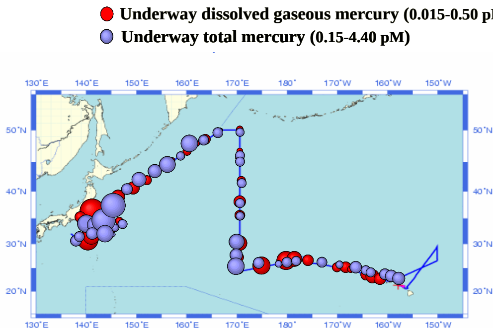
Figure 11.8 -Concentrations of total mercury and dissolved gaseous mercury for surface samples collected using the fish sampler during the may/June 2002 cruise. Adapted from Laurier et al. (2004). Size of the circle illustrates the relative concentrations between the maximum and minimum values shown in the leg.
