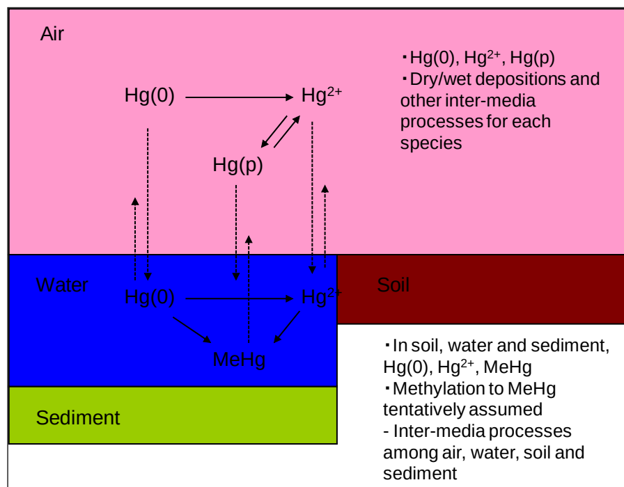
Figure 12.6 – Transformation scheme of mercury species in the modeling study.
