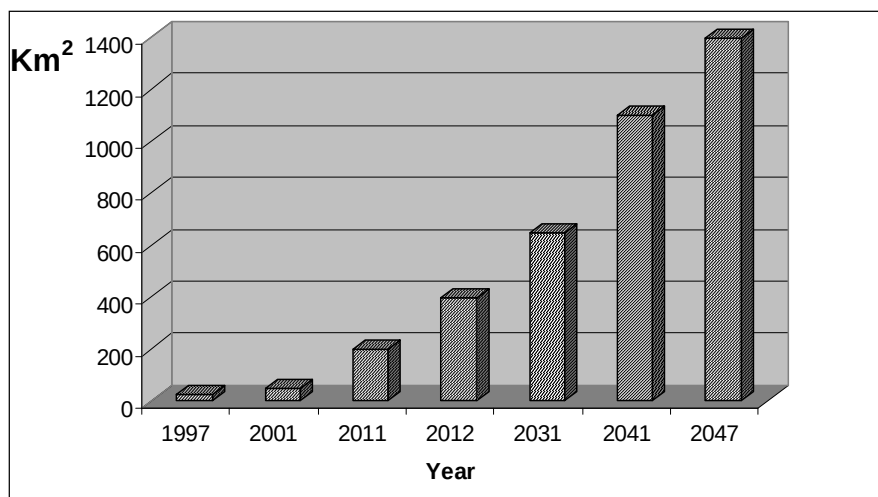
Figure 4.7 - Land requirement (km 2 ) for disposal of municipal solid waste (reproduced from Singhal and Pandey 2001).
