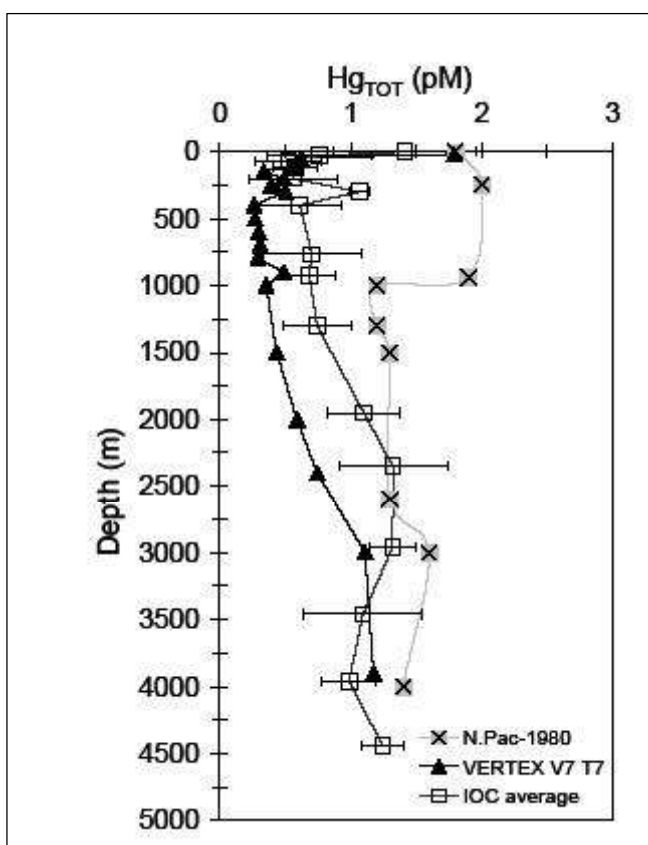
Figure 11.14 - Concentrations of total mercury (reactive mercury for the earlier studies) measured on the three cruises discussed in the text: the 1980 North Pacific cruise, the VERTEX cruise data and the 2002 IOC cruise. Taken from Laurier et al. (2004).
