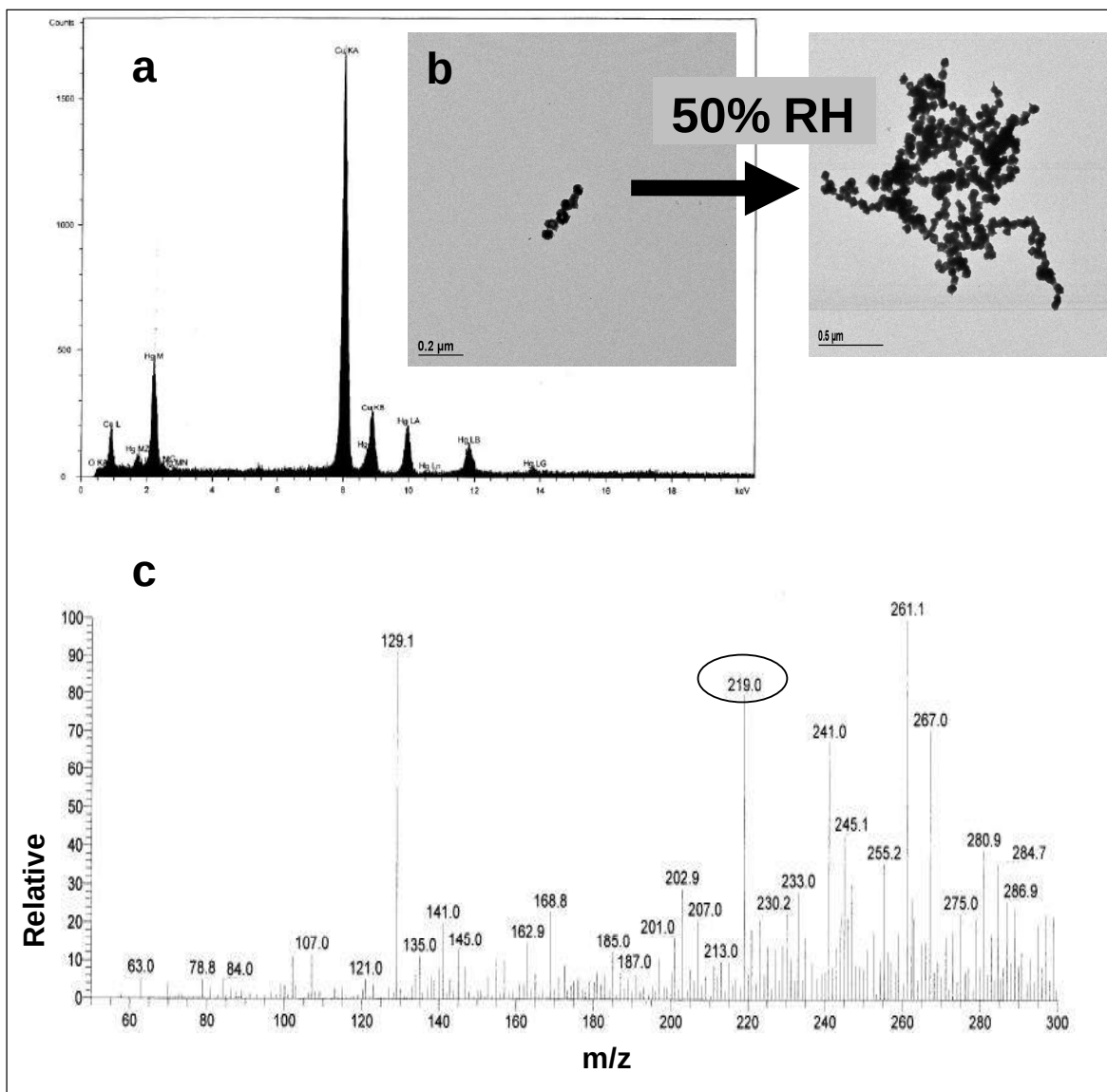
Figure 15.2 - - Energy dispersive spectroscopy (EDS) image of HgO b) Comparative HRTEM image of HgO deposit at RH = 0% and 50%, and c) CI of HgO product at RH = 0% and 50%. From Snider et al., 2008.
