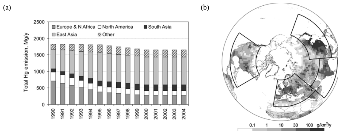
Figure 20.2 - Long-term changes of mercury anthropogenic emissions in the Northern Hemisphere (a) and spatial distribution of Hg anthropogenic emissions in 2000 (b). Solid lines depict source regions selected for the analysis.
