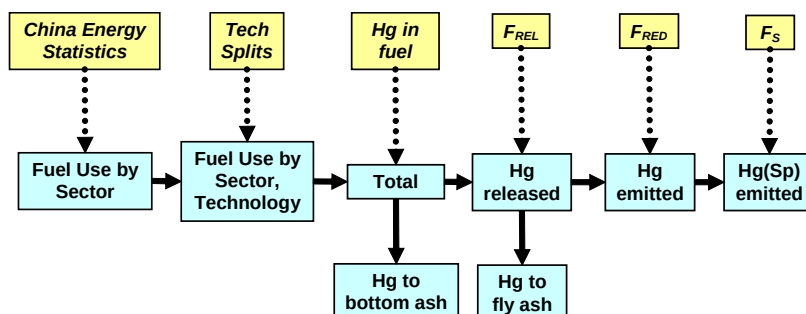
Figure 2.5 - Calculation procedure for mercury emissions; F_{REL} = fraction released to the air during combustion; F_{RED} = fraction reduced by emission control devices; F_S = fraction emitted by species type.
