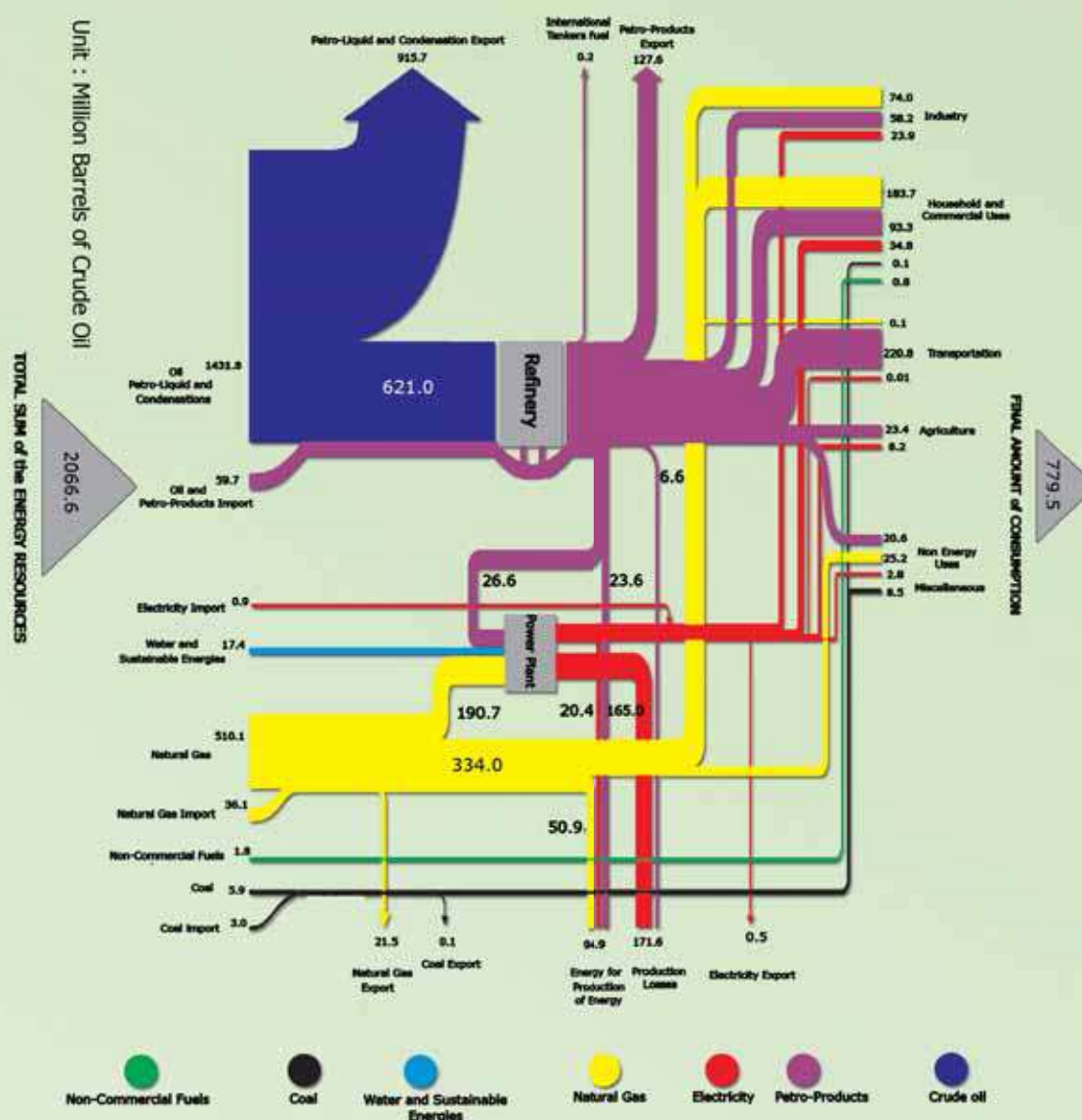
Picture 2-5: Energy flows in 2004 Source: Ministry of Energy
