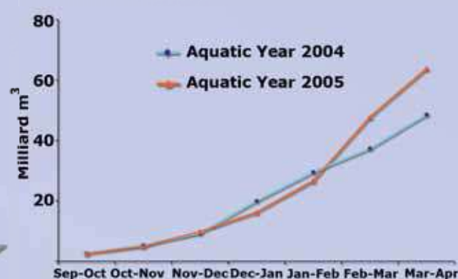
Figure 6-4: Comparison of the volume accumulation of surface water in the present and the previous year.
