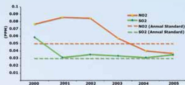
Figure 4-15: SO 2 and NO 2 releases in Tehran, 1999-2004
