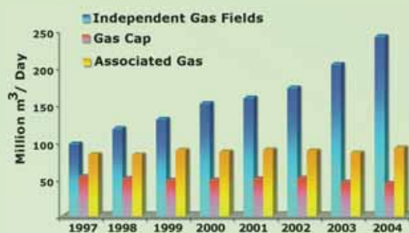
Figure 2- 11: Production trend of enriched gas, 1997-2004 Source: Ministry of Energy, 2004b
