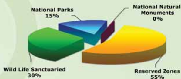
Figure 2-5: Percentage distribution of areas under DoE management in 2006 Source: DoE, 2006
