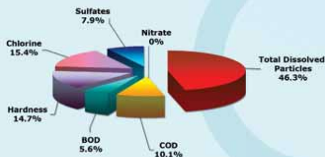
Figure 7-3: Total percentages of pollutants discharged into the Karoon and Dez rivers (rural and urban catchments)
