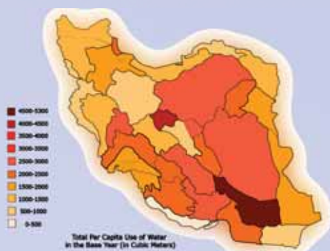
Picture 6-1: Map of water consumption in different catchment areas, 1995
