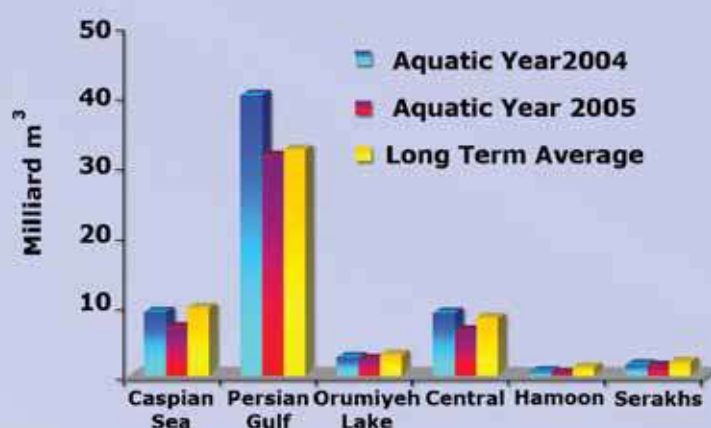
Figure 6-3: Volume of surface water in the main catchment areas, up to the March, 2005.
