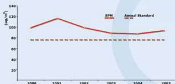
Figure 4-17: Trend of SPM release in Tehran, 2000-2004
