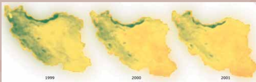
Picture 9-1: The process of change in vegetation cover, 1999-2001
