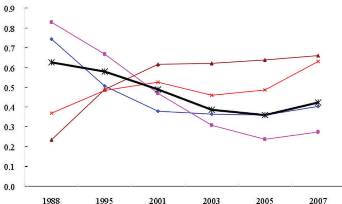
Figure 1.14. Jiaozhou Bay coastal ecosystem evaluation index from 1988 to 2007 .
