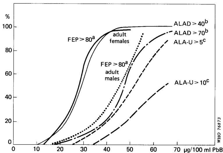
Fig. 4. Dose response relationships for some effects of lead. a = \mu\text{g}/100\text{ ml} of erythrocytes; b = % inhibition; c = mg/litre.
