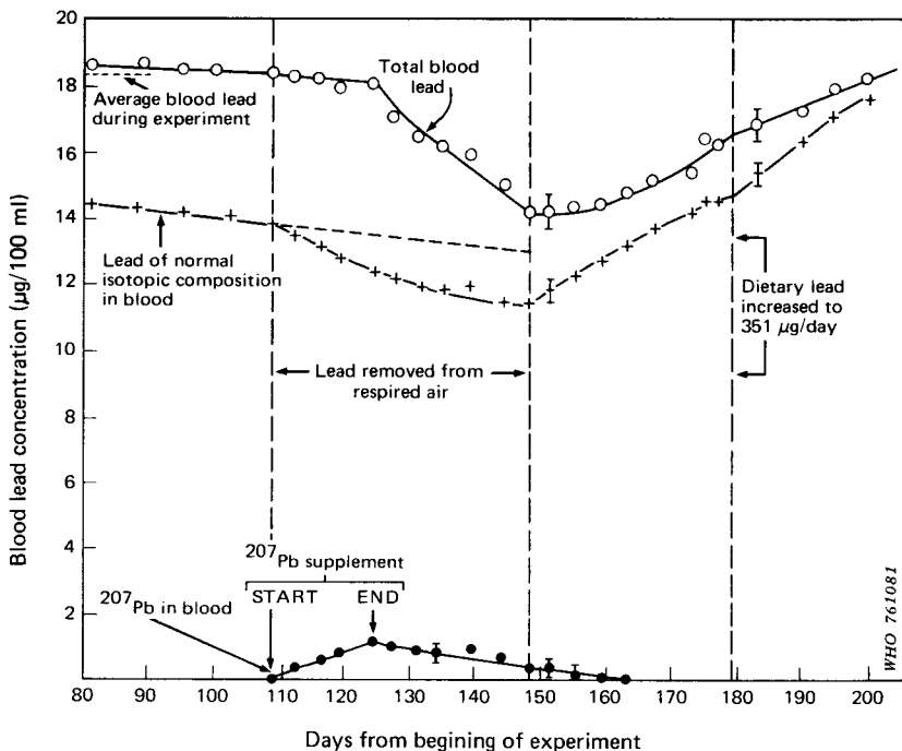
Fig. 2 Effect on blood lead of removal of lead from room air. Adapted from Rabinowitz (1974) with the addition of the dashed line.
