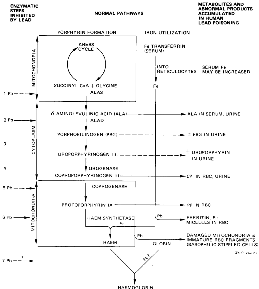
Fig. 3 Lead interference with the biosynthesis of haem (NAS-NRC 1972).
