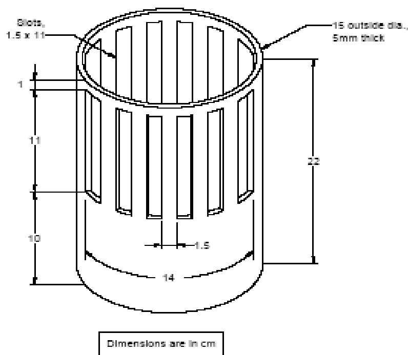
Figure 2.9: Slotted cylinder (shown upside down)
