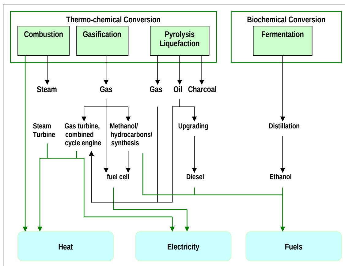
Chart I: Conversion Routes for Cellulosic Agricultural Biomass Waste
