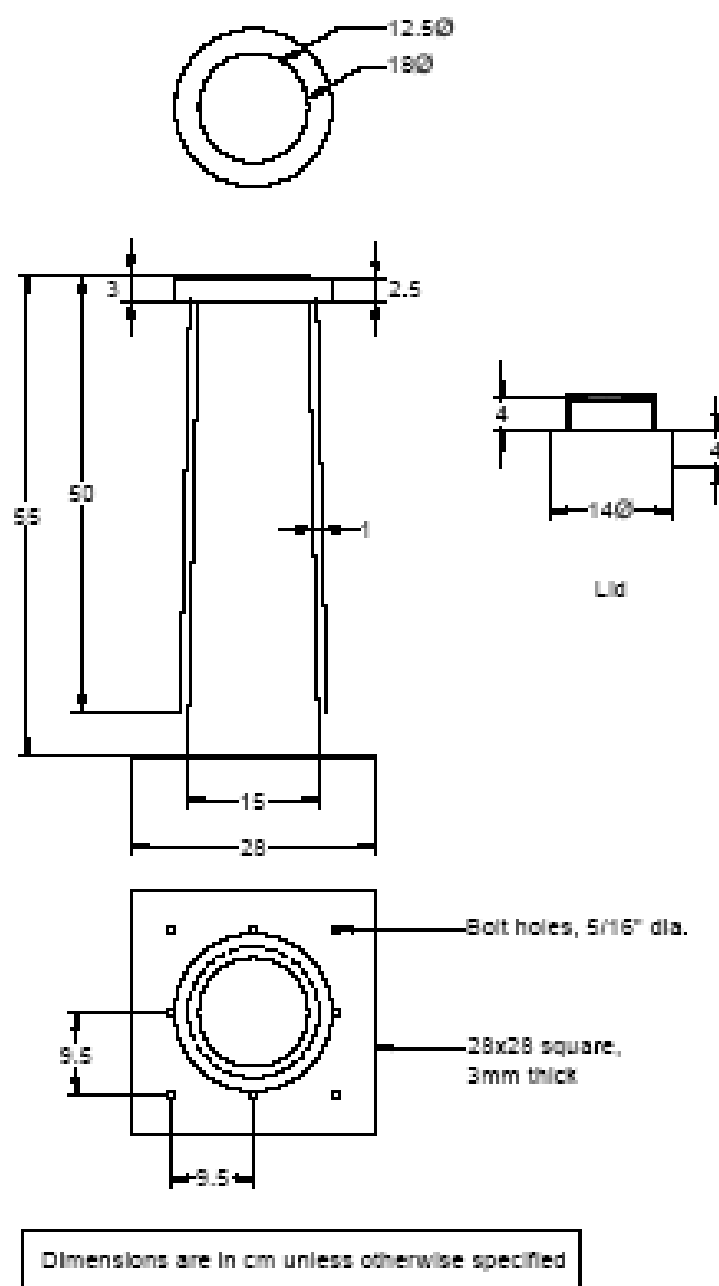
Figure 2.13: Fuel chamber
