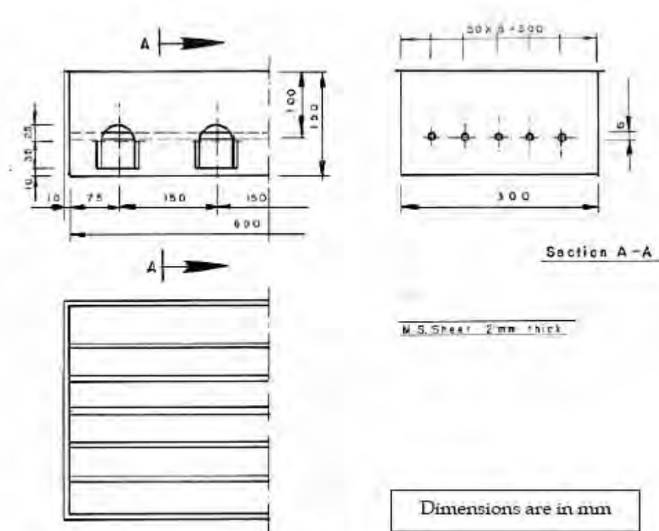
Figure 7.3: Dimensional details of the biomass stove
