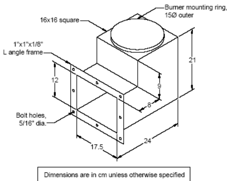
Figure 2.15: Isometric view of gas burner base
