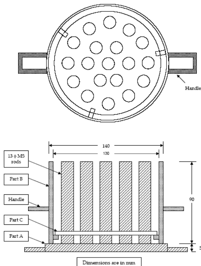
Figure 7.5: Briquette mould
