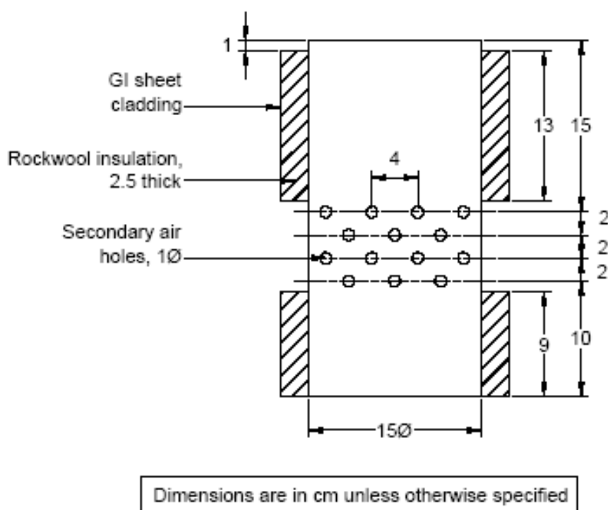
Figure 2.16: Sectional view of the gas burner
