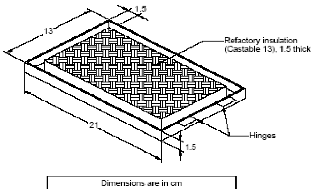
Figure 2.12: Ash pit door (Inside view)
