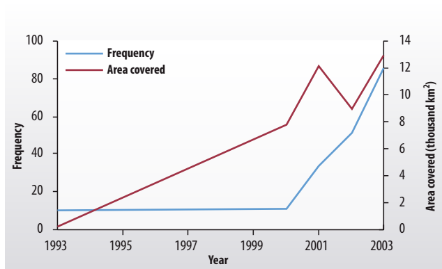
Figure 18 Trends in harmful algal blooms in the East China Sea. (SOA 1999, SOA 2000, SOA 2001, SOA 2002, SOA 2003a, SOA 2003b)
