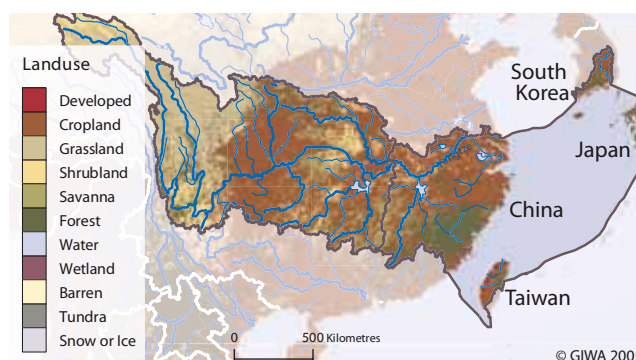
Figure 7 Land use map of the Yangtze River Basin.
