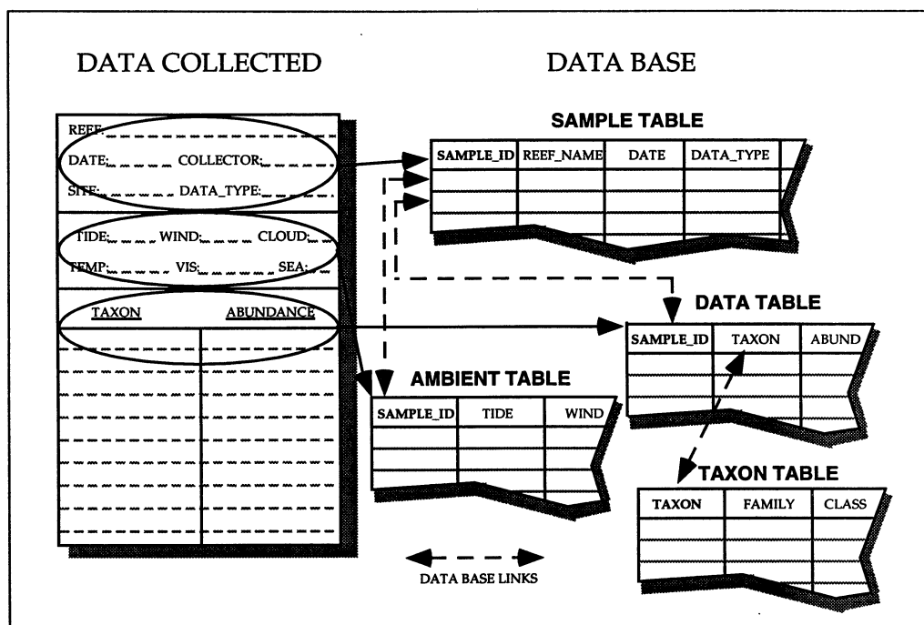
Figure 26. A relational database.
