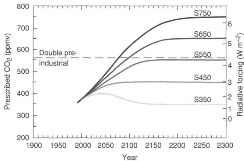
Figure 6: Profiles of atmospheric \text{CO}_2 concentration leading to stabilisation at 350, 450, 550, 650 and 750 ppmv. Doubled pre-industrial \text{CO}_2 concentration is 560 ppmv. The radiative forcing resulting from the increase in \text{CO}_2 relative to pre-industrial levels is marked on the right-hand axis. Note the non-linear nature of the relationship between \text{CO}_2 concentration change and radiative forcing.
