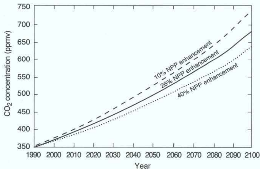
Figure 1.15: Concentration uncertainties associated with the CO 2 fertilisation effect for the IS92a emission scenario. The central curve shows the concentration projection using “best guess” model parameters using the model of Wigley (1993), which is similar to projections using other models. For the upper and lower curves the CO 2 fertilisation effect was decreased to 10% NPP enhancement (from 26% for the “best guess” simulation) and increased to 40% NPP enhancement for a CO 2 doubling from 340 ppmv to 680 ppmv. As explained in Wigley (1993), this assessment also captures some of the uncertainties arising from ocean flux uncertainties, through the need to balance the contemporary carbon budget within realistic limits.
