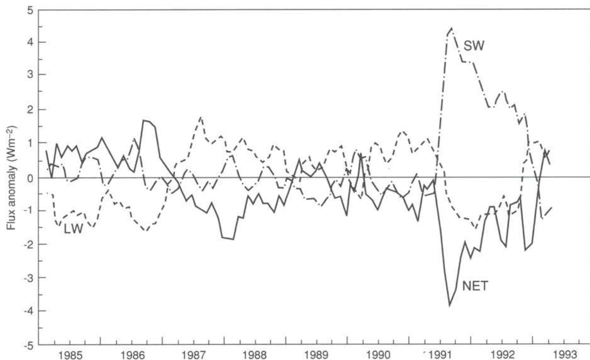
Figure 4.6: Time series of smoothed wide field of view Earth Radiation Budget Experiment long-wave (LW), short-wave (SW) and net (LW-SW) irradiance anomalies (in \text{Wm}^{-2} ) between 40^\circ\text{N} and 40^\circ\text{S} relative to the 5 year (1985-1989) monthly mean (after Minnis et al. , 1993, updated by Minnis, 1994). The deviation starting in mid-1991 is mainly due to the Mt. Pinatubo eruption – the net anomaly in August (about -4 \text{ Wm}^{-2} ) is almost three times higher than the standard deviation computed between 1985 and 1989.
