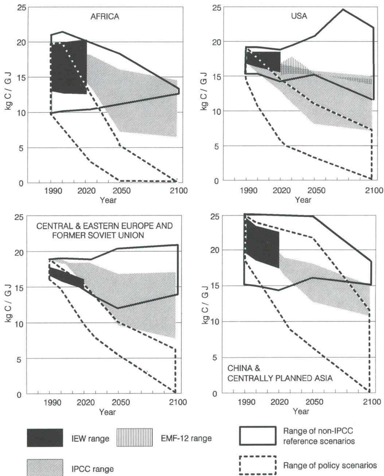
Figure 6.9: Range of regional carbon intensities from IS92 and other published scenarios.
