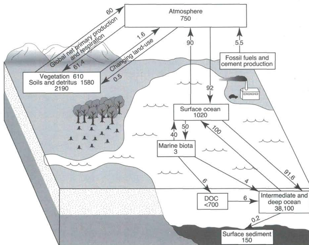
Figure 1.1: The global carbon cycle, showing the reservoirs (in GtC) and fluxes (GtC/yr) relevant to the anthropogenic perturbation as annual averages over the period 1980 to 1989 (Eswaran et al., 1993; Potter et al., 1993; Siegenthaler and Sarmiento, 1993). The component cycles are simplified and subject to considerable uncertainty. In addition, this figure presents average values. The riverine flux, particularly the anthropogenic portion, is currently very poorly quantified and so is not shown here (see text). While the surface sediment storage is approximately 150 Gt, the amount of sediment in the bioturbated and potentially active layer is of order 400 Gt. Evidence is accumulating that many of the key fluxes can fluctuate significantly from year to year (terrestrial sinks and sources: INPE, 1992; Ciais et al., submitted; export from the marine biota: Wong et al., 1993). In contrast to the static view conveyed by figures such as this one, the carbon system is clearly dynamic and coupled to the climate system on seasonal, interannual and decadal time-scales (Schimel and Sulzman, 1994; Keeling and Whorf, 1994).
