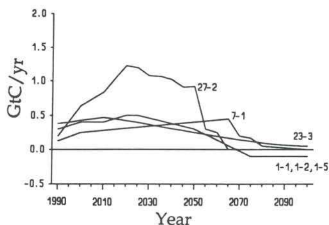
Figure 6.14a: CO 2 fluxes from deforestation for Africa for different scenarios. Numbers correspond to list of scenarios in the Supplementary Table.
