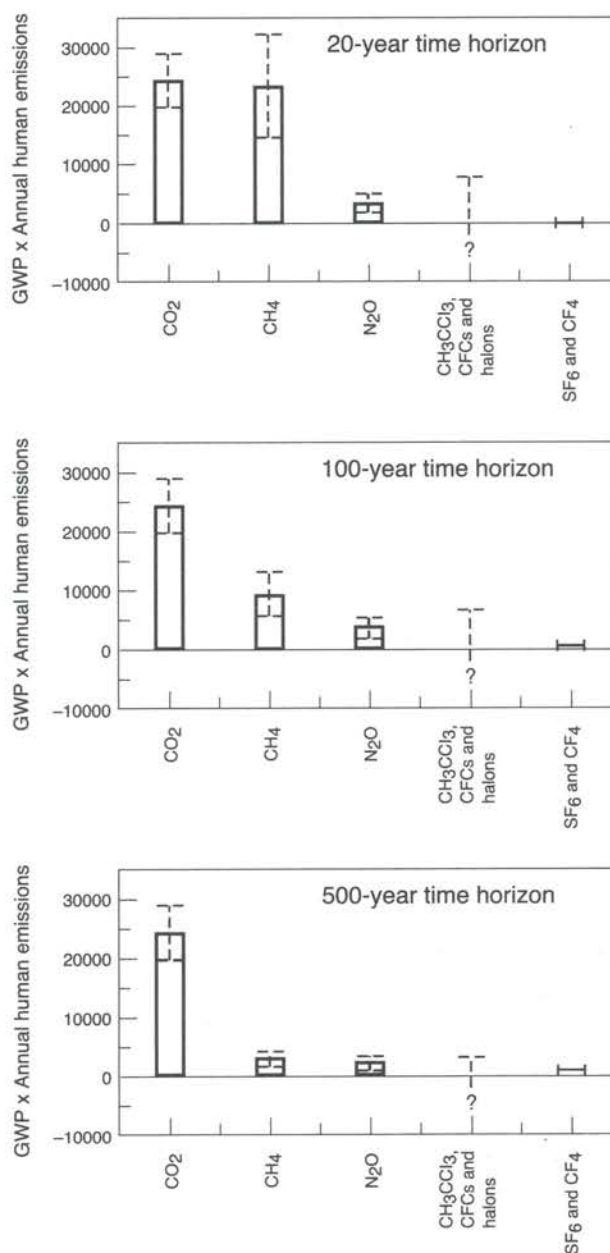
Figure 5.7: The product of GWP with estimated annual anthropogenic emissions typical of the 1980s for various gases, for time horizons of 20, 100 and 500 years. Ranges indicate the range of possible uncertainties considered here in estimating GWPs and total anthropogenic emissions. The estimated emissions are approximate. Note that uncertainties in the indirect radiative forcing of CFCs and halons due to ozone depletion imply that the net GWPs for these gases could be negative, but this is presently uncertain.
