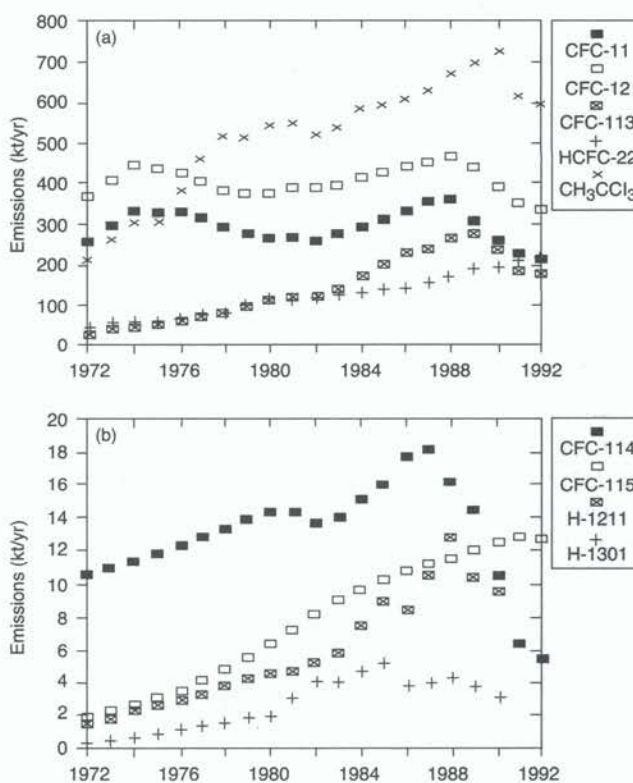
Figure 2.6: Annual emissions of some important industrial halocarbons from 1972 to 1992 based on production statistics (AFEAS, 1993; Fisher et al. , 1994; Fisher, 1994 and unpublished work from D. Fisher and P. Midgley). For CFC-11, CFC-12, CFC-113, CH_3CCl_3 and the halons, the estimates are for global use; for HCFC-22, CFC-114 and CFC-115, the estimates are from reporting companies and may be somewhat less than the global emissions.
