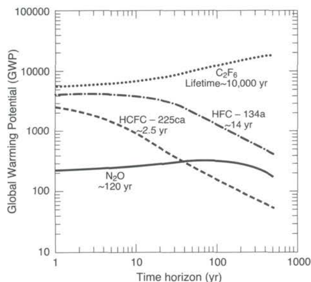
Figure 5.3: Global Warming Potentials (GWPs) for a range of greenhouse gases with differing lifetimes, as in Figures 5.1 and 5.2, using CO_2 as the reference gas.
