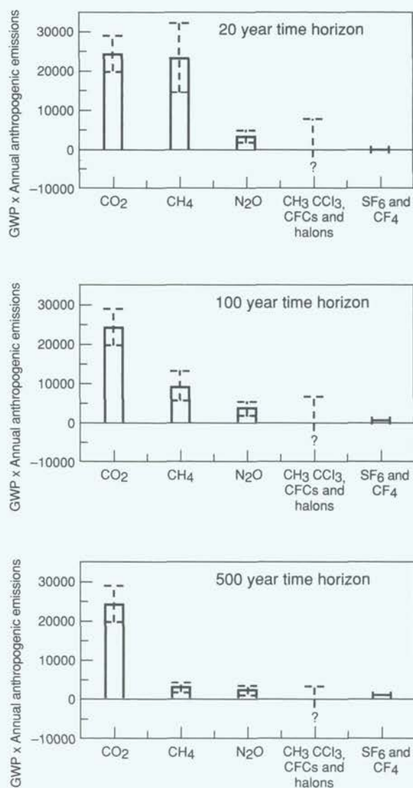
Figure 13: The product of GWP with estimated annual emissions typical of the 1980s for various gases, for time horizons of 20, 100 and 500 years. The dashed bars indicate the range of possible uncertainty considered here in estimating GWPs and total anthropogenic emissions. The estimated emissions are approximate. The indirect radiative forcing of CFCs and halons due to ozone depletion imply that the net GWPs for these gases could be negative, but this is presently uncertain.
