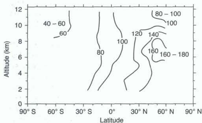
Figure 2.10: The CO mixing ratios (ppbv) as a function of latitude and altitude averaged over the four transects that were measured during the STRAT0Z II and STRAT0Z III flights in April/May 1980 and June 1984. During each of the missions, one distribution along the east coast of North America and the west coast of South America and another along the east coast of South America and the west coast of Africa were determined (Seiler and Fishman, 1981; Marengo et al. , 1990).
