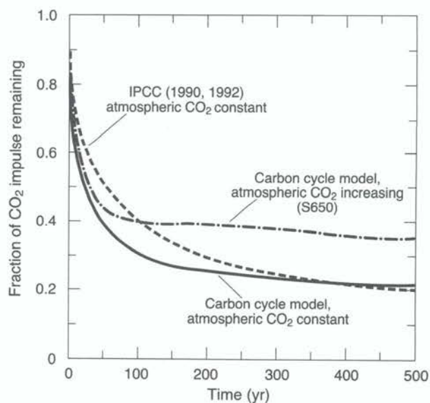
Figure 5.5: Impulse response for an injection of CO 2 versus time for the adopted carbon model for two future CO 2 scenarios: (i) constant current CO 2 concentrations and (ii) the increasing CO 2 concentrations of the S650 profile shown in Figure 1.12. Also shown for reference is the three-exponential function used to represent the CO 2 decay response in IPCC (1990, 1992).
