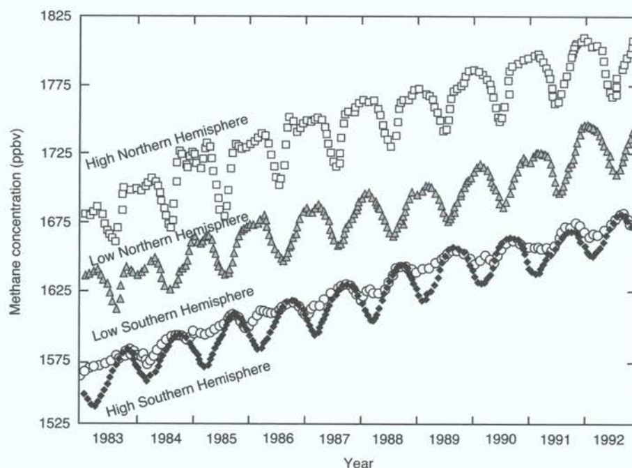
Figure 2.2: Seasonal cycles and trends in atmospheric methane over the decade 1983 to 1992. Results from the NOAA-CMDL global flask network (37 sites) have been gridded to 14-day intervals and averaged over four equal areas of the atmosphere: high northern ( 30^{\circ}\text{N} - 90^{\circ}\text{N} ), low northern ( 0 - 30^{\circ}\text{N} ), low southern ( 0 - 30^{\circ}\text{S} ) and high southern ( 30^{\circ}\text{S} - 90^{\circ}\text{S} ) semi-hemispheres (Steele et al. , 1992; Dlugokencky et al. , 1994c).
