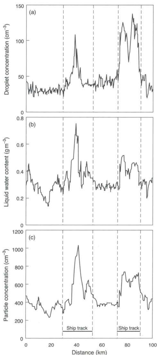
Figure 3.9: Observations of the changes in microphysical properties of stratocumulus clouds on a level flight through cloud in which ship tracks are present (from Radke et al. , 1989). The ship tracks contain high aerosol particle and cloud droplet concentrations leading to increased cloud water content.
