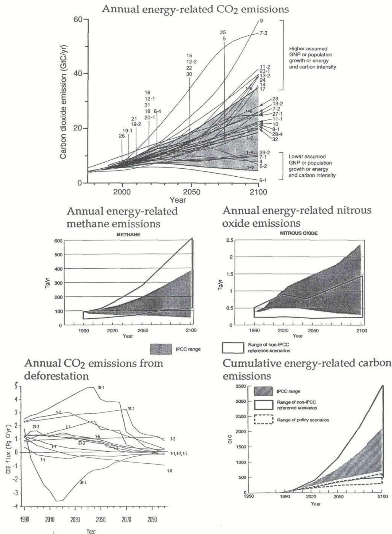
Figure 1: Annual emissions of CO 2 , CH 4 and N 2 O from energy-related sources, annual emissions of CO 2 from deforestation, and cumulative CO 2 emissions from energy related sources.
