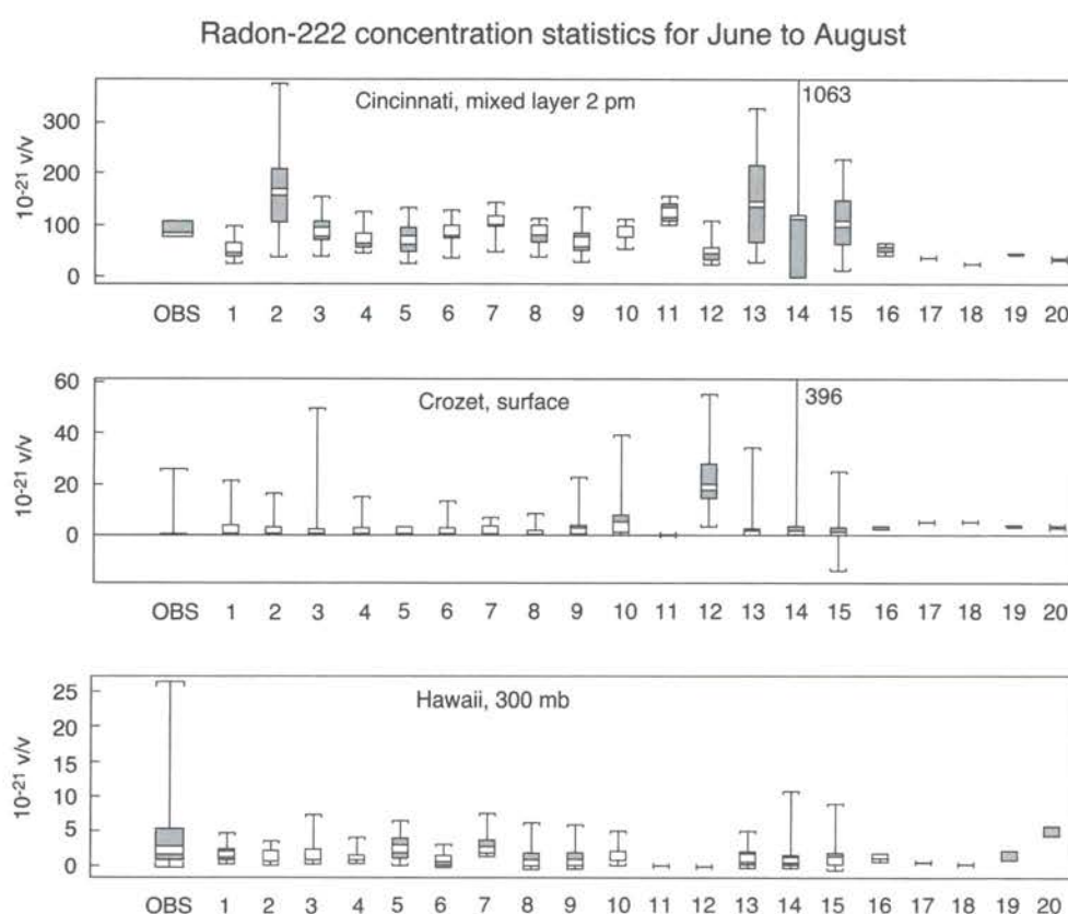
Figure 2.11: Radon-222 concentration statistics (OBS) for June, July and August at Cincinnati OH (40°N, 84°W, mixed layer at 2 p.m.), Crozet I. (46°S, 51°E, surface), and over Hawaii (20°N, 155°W, 300 mbar). Modelled time-series show minima and maxima, quartiles (shaded box), and medians (white band). Identification codes are given in Table 2.7. Observations at Hawaii (Balkanski et al. , 1992) show the same statistics; but for Cincinnati (Gold et al. , 1964) the shaded box gives the interannual range of June-August means; and for Crozet (Polian et al. , 1986), the lower bar gives background concentrations, with the upper bracket showing typical maximum events.
