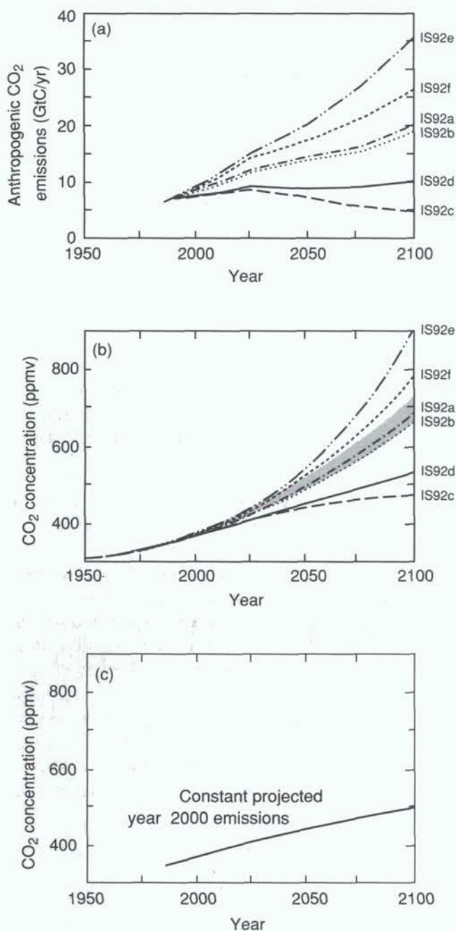
Figure 5: (a) Prescribed anthropogenic emissions of CO 2 (from fossil fuel use, deforestation and cement production) for the IS92 Scenarios, (b) CO 2 concentrations resulting from the IS92 emission scenarios calculated using the "Bern" model, a mid-range carbon cycle model (a range of results from different models is indicated by the shaded area of the IS92a curve) and (c) CO 2 concentrations resulting from constant projected year 2000 emissions (using the model of Wigley).
