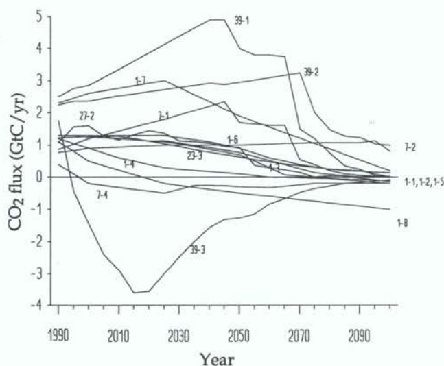
Figure 6.12: Comparison of global scenarios of CO 2 fluxes from deforestation. Numbers correspond to list of scenarios in the Supplementary Table.
