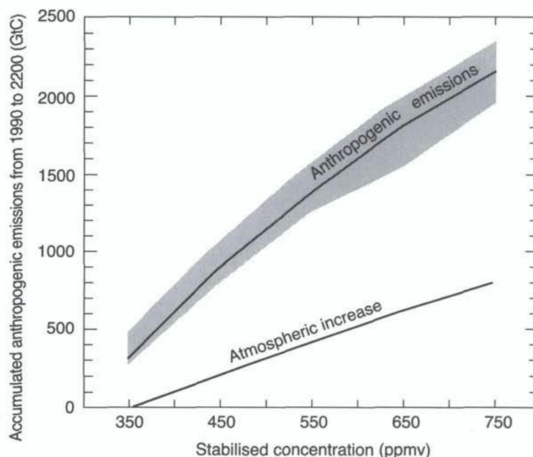
Figure 8: Anthropogenic \text{CO}_2 emissions shown in Figure 7 accumulated from 1990 to 2200 plotted against the final stabilised concentration. For example, accumulated emissions of between 1200 and 1600 GtC lead to stabilisation at a concentration of 550 ppmv. The figure also shows the amount of \text{CO}_2 (in GtC) remaining in the atmosphere at each stabilisation level. The difference between accumulated emissions and atmospheric increase represents the accumulated uptake by the ocean and the marine and terrestrial biospheres. The range of results from different models is indicated by the shaded area.
