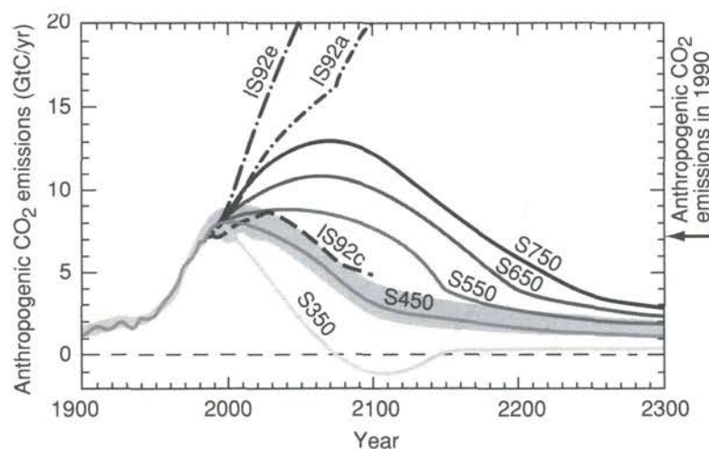
Figure 7: Illustrative anthropogenic emissions of \text{CO}_2 leading to stabilisation at concentrations of 350, 450, 550, 650 and 750 ppmv following the profiles shown in Figure 6 (using a mid-range carbon cycle model). The range of results from different models is indicated on the 450 ppmv profile. The emissions for the IS92a, c and e Scenarios are also shown on the figure. The negative emissions for stabilisation at 350 ppmv are an artefact of the particular concentration profile imposed.
