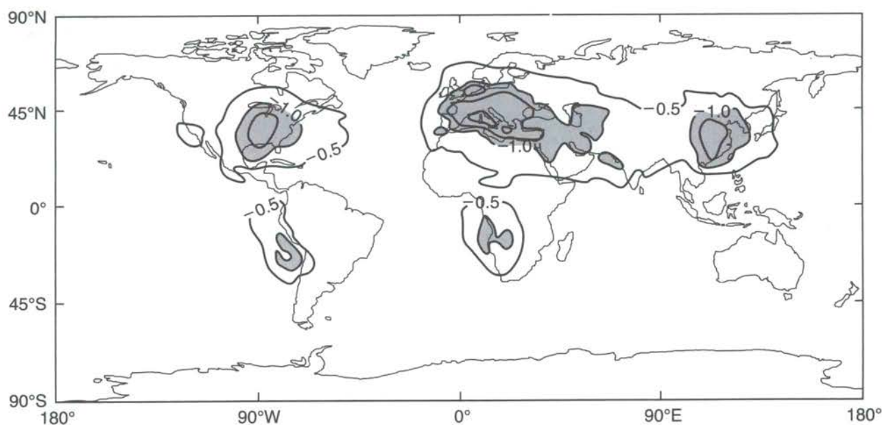
Figure 12: Modelled geographic distribution of annual mean direct radiative forcing ( \text{Wm}^{-2} ) from anthropogenic sulphate aerosols in the troposphere. The negative radiative forcing is largest over or close to regions of industrial activity.
