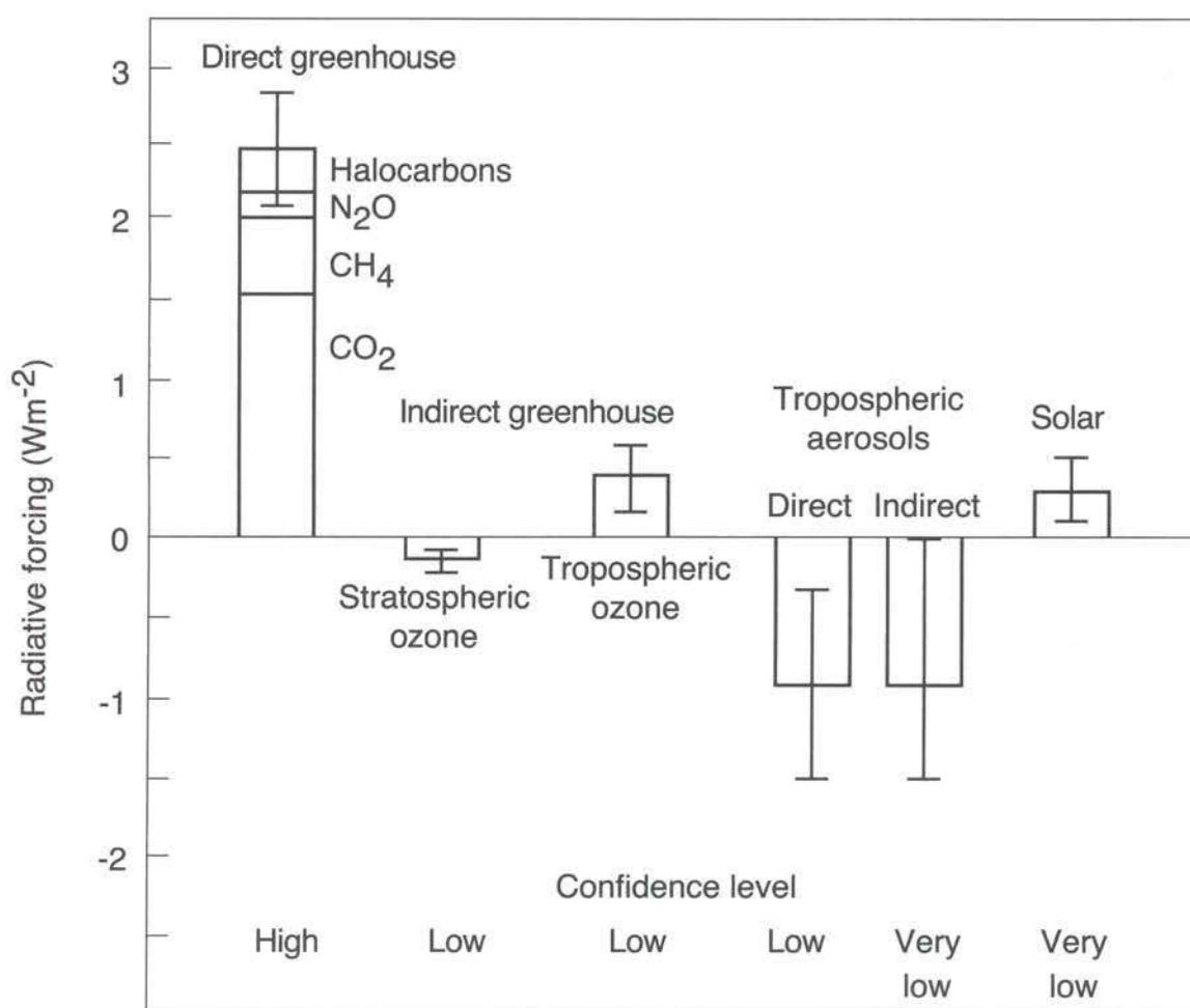
Figure 4.8: Estimates of the global and annual-mean radiative forcing (Wm -2 ) from 1850 to 1990 for a number of potential climate change mechanisms. The height of the column indicates a mid-range estimate of the forcing whilst the error bars show an estimate of the uncertainty range. Our confidence that the actual forcing lies within this range varies greatly from mechanism to mechanism; a subjective confidence level is indicated for each mechanism as either high, low or very low. The contributions of individual greenhouse gases are indicated in the first column. The episodic and transient nature of the effects of volcanic eruptions means that their relative importance depends greatly on the precise period for which forcings are quoted; their effects are not shown in the figure, but they can be of importance on decadal time-scales.
