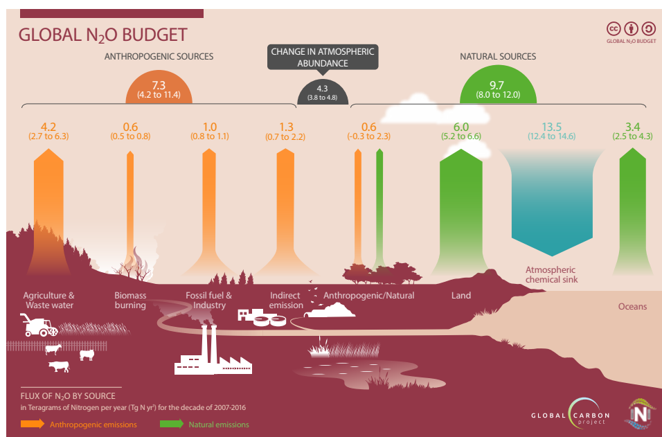
Figure 5. Mean global N 2 O budget for all major anthropogenic and natural sources and sinks for the decade 2007–2016 (redrawn from Tian et al., 2020).
