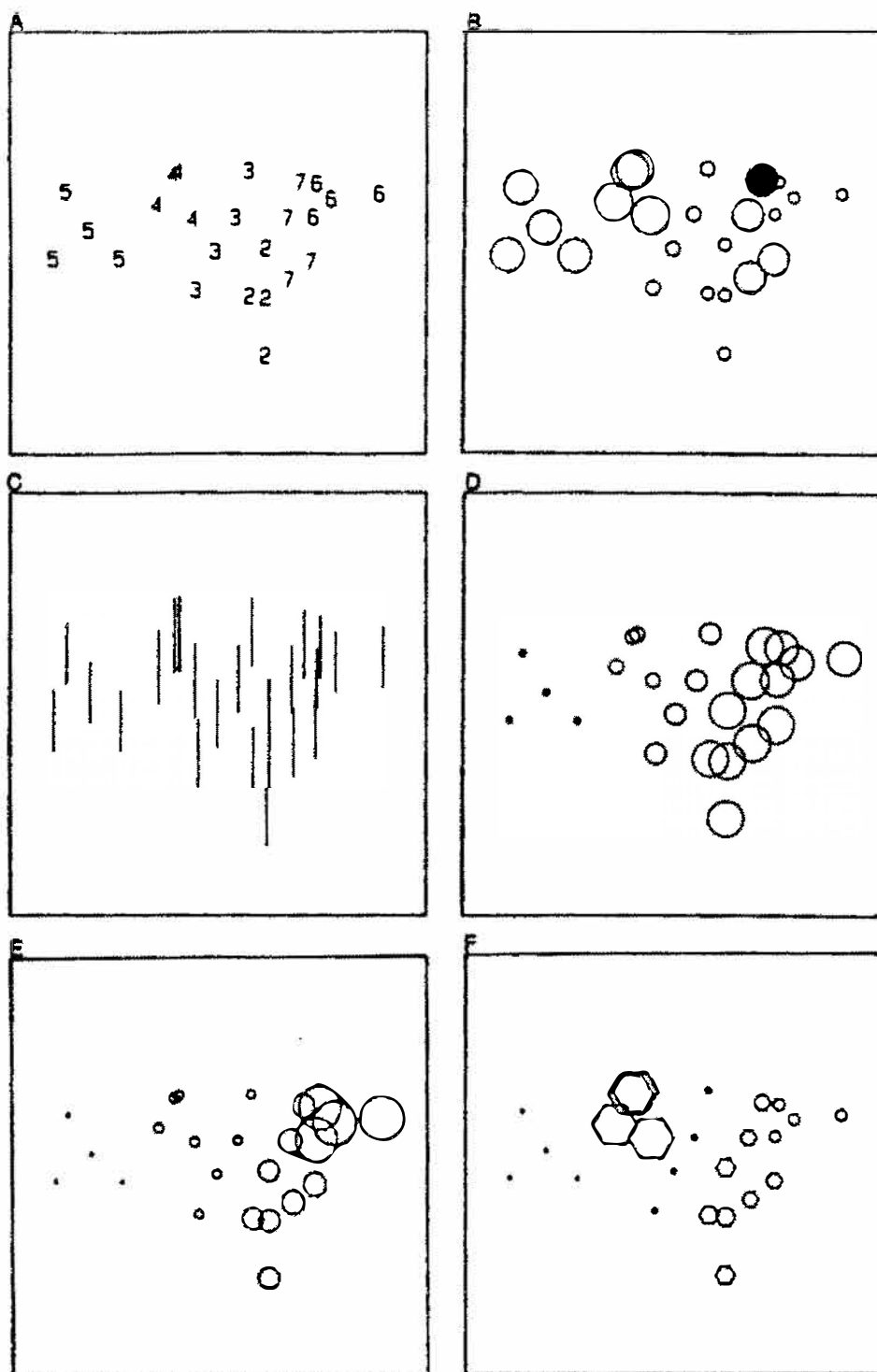
Fig. 14.6. A) 2-D MDS configuration for macrofauna standardised root-transformed abundance. B-F) same configuration with symbols representing values of environmental variables superimposed: B) grain size, C) water depth, D) sediment Pb concentration, E) TBT in water, F) sediment PAH.
