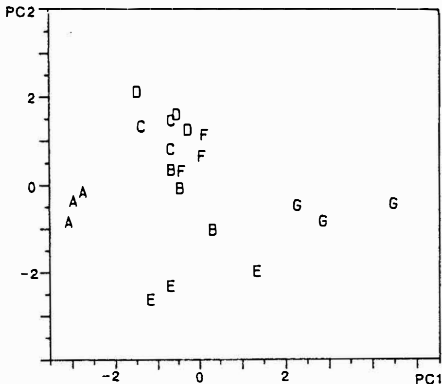
Fig. 11.1. Frierfjord sediments. 2-d PCA of metal data of Table 11.1 ( \sqrt{\cdot} -transformed and normalised).
