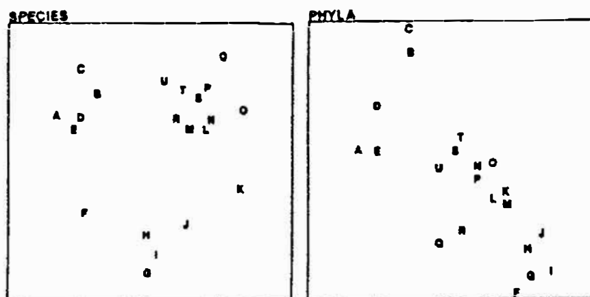
Fig. 10.4. MDS for macrobenthos at station "Pierre Noire". Species data (left) aggregated into phyla (right). Sampling months are A:4/77, B:8/77, C:9/77, D:12/77, E:2/78, F:4/78, G:8/78, H:11/78, I:2/79, J:5/79, K:7/79, L:10/79, M:2/80, N:4/80, O:8/80, P:10/80, Q:1/81, R:4/81, S:8/81, T:11/81, U:2/82. Oil-spill was during 3/78, i.e. between E and F. Note more linear configuration for phyla.
