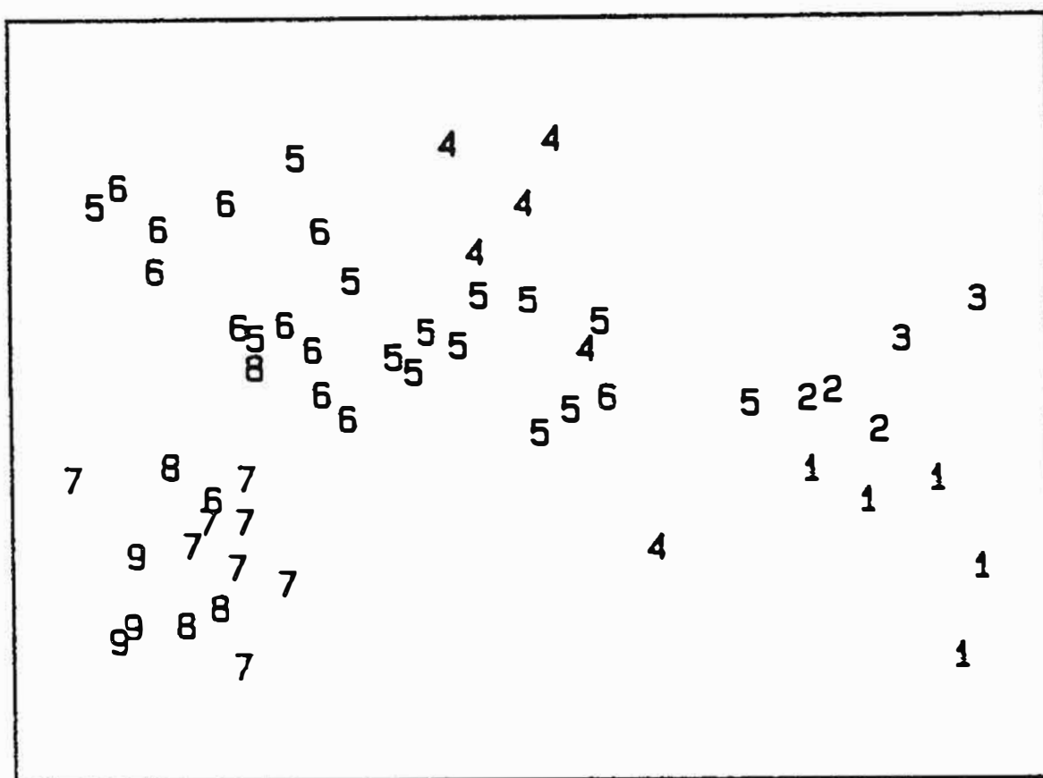
Fig. 11.4. MDS of 57 sites, with increasing salinity categories superimposed. 1: \leq 26.3 , 2: (26.3, 29.0) , 3: (29.0, 31.0) , ..., 8: (34.7, 35.1) , 9: \geq 35.1\text{‰} .
