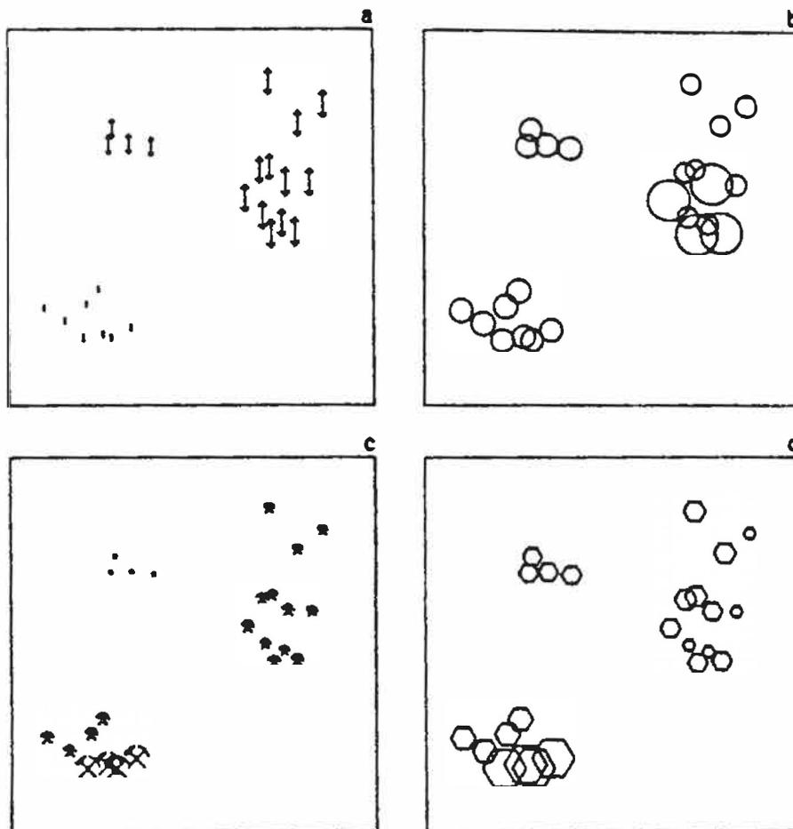
Fig. 11.5. MDS of sites A-E,G with superimposed values of (a) water depth (22-113m), (b) sediment median grain size (7.8-16.5 \mu m), (c) metal levels (PC1 in Fig. 11.1) and (d) "total" PAH (4.4-14.8 \mu g/g).
