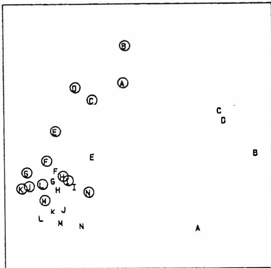
Fig. 5.6. MDS of zooplankton samples at a single site (22/9/78), from 14 depths (5m to 70m, denoted A,B,...,N) for night (circles) and day-time hauls.
