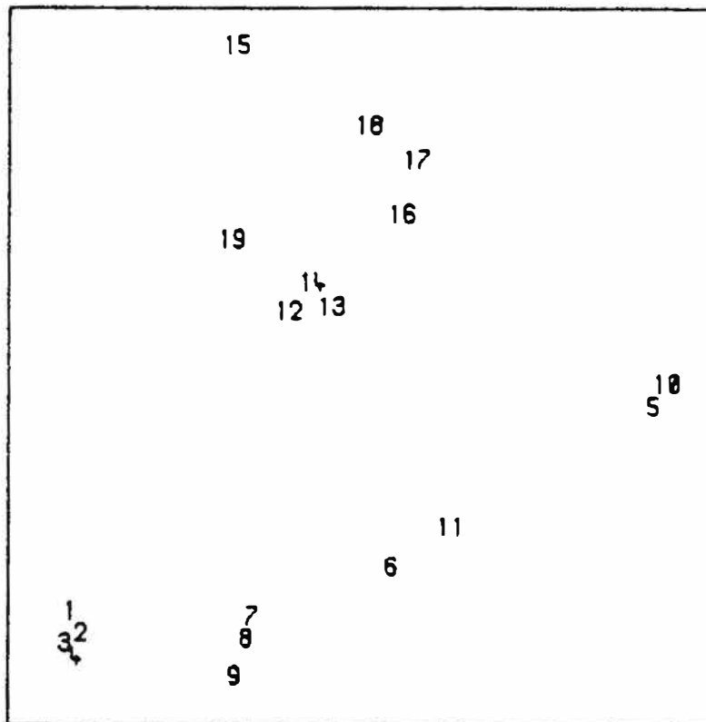
Fig. 5.1. Exe nematodes. 2-d MDS ordination of 19 sites, from Bray-Curtis similarities on \sqrt{\sqrt{}} transformed abundances (182 species).
