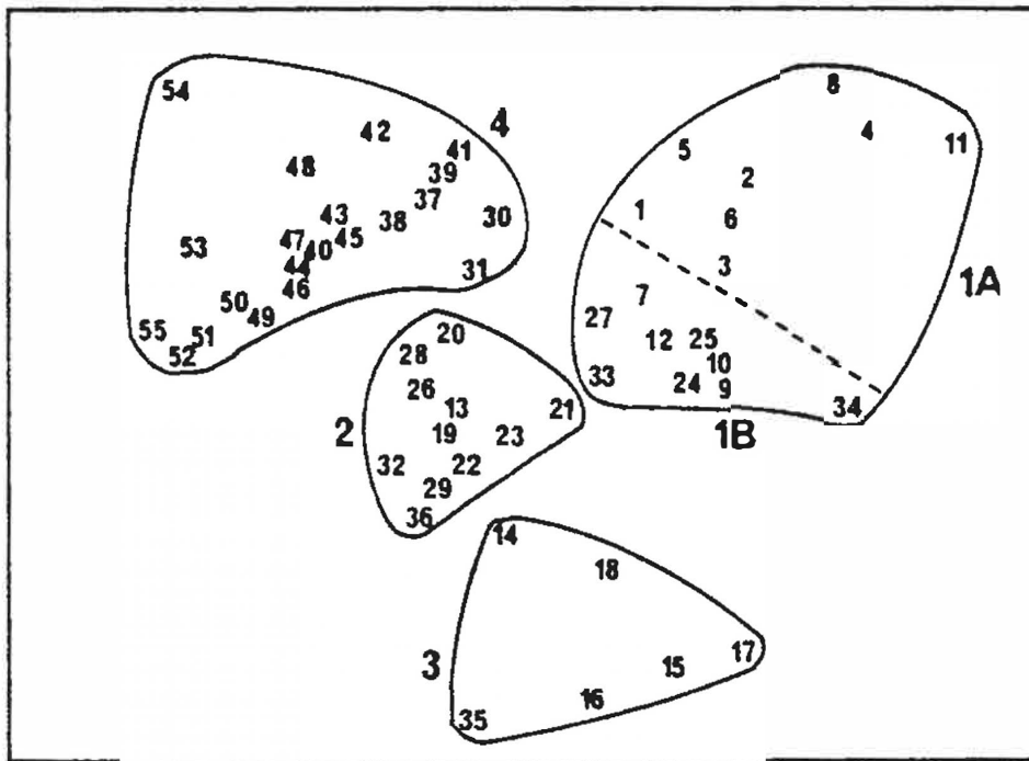
Fig. 7.2. Exe nematodes . MDS of 55 commonest species using Bray-Curtis similarities on standardised abundances. Main groups from cluster analysis (Fig. 7.1) indicated; they correspond closely to groupings of sites (Fig. 5.4).
