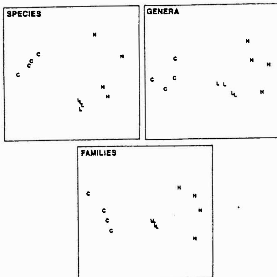
Fig. 10.2. Mesocosm copepod counts - 3 levels of nutrient enrichment (Gee et al. 1985). Sample MDS plot (Bray-Curtis, \sqrt{} transform); species data aggregated into genera and families (Warwick 1988).
