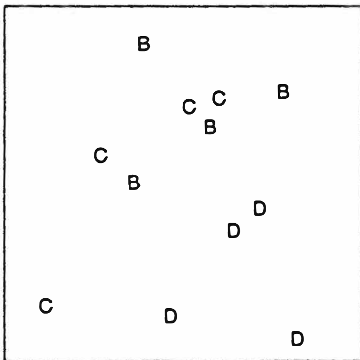
Fig. 6.4. Frierfjord macrofauna. MDS plot (Bray-Curtis, \sqrt{} transform) of 4 replicates from B,C,D.
