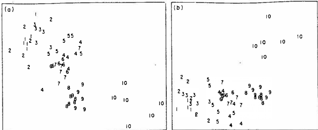
Fig. 14.16. MDS for nematodes (left) and copepods (right) for six replicate cores at each of 10 stations. Note that, allowing for the difference in orientation, the configurations are almost identical.
