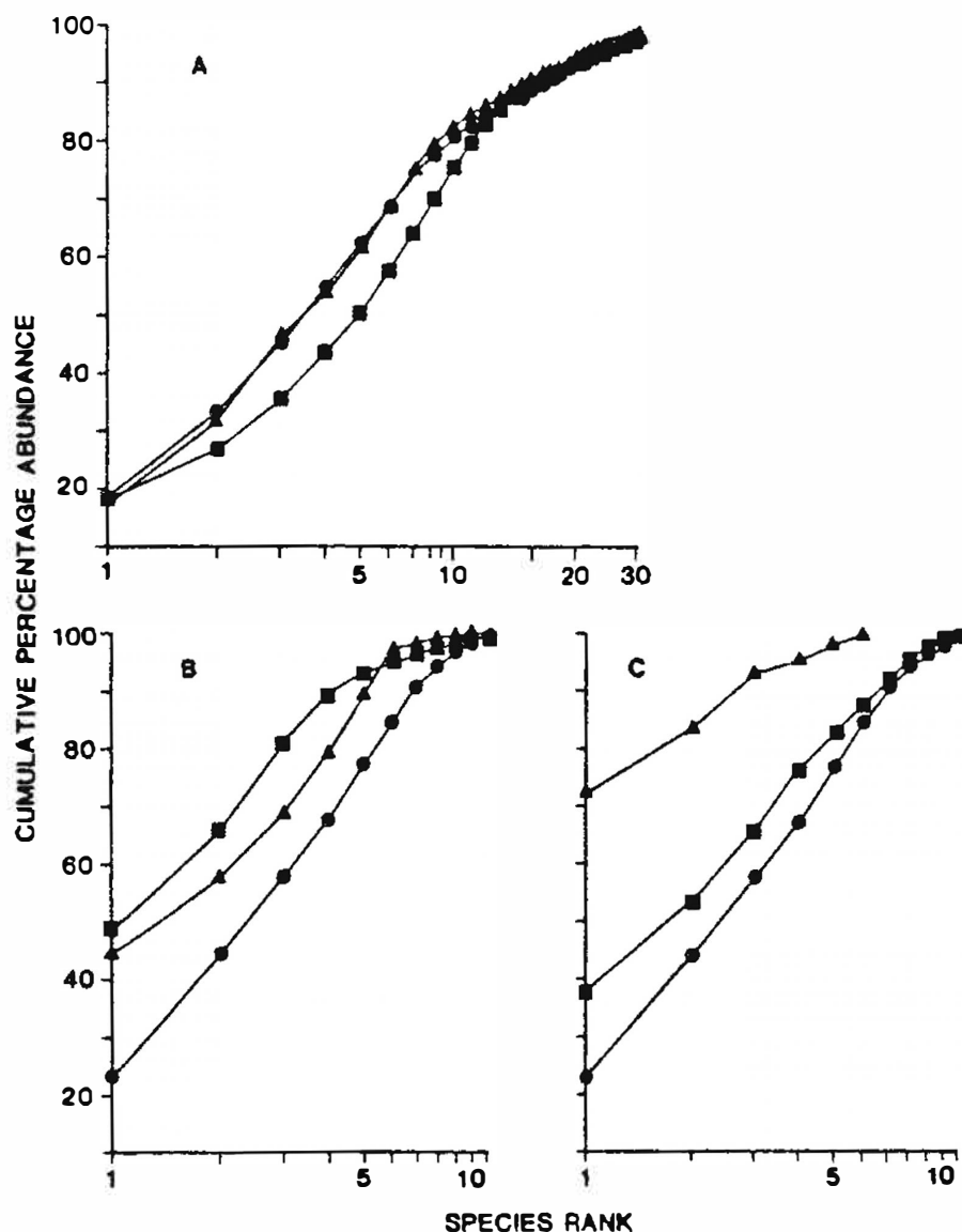
Fig. 12.6. k -dominance curves for A nematodes, B total copepods and C copepods omitting the 'weed' species of Tisbe for summed replicates of each treatment. Circles - control, squares - low dose, triangles - high dose.
