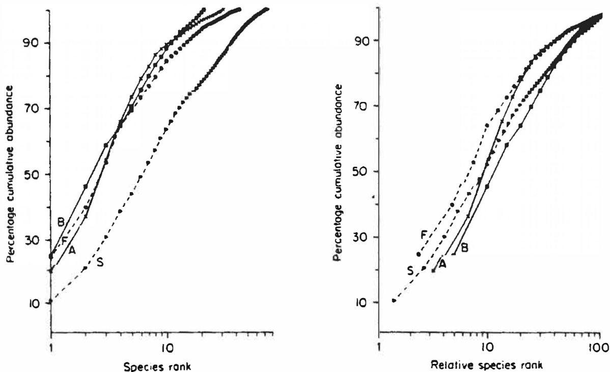
Fig. 8.5. k -dominance curves (left) and Lorenz curves (right) for 20 cm deep cores taken from experimental sand columns 20 days (A) and 77 days (B) after initial setup, and from intertidal (F) and subtidal (S) sand from the study site (from Lamshead et al. , 1983).
