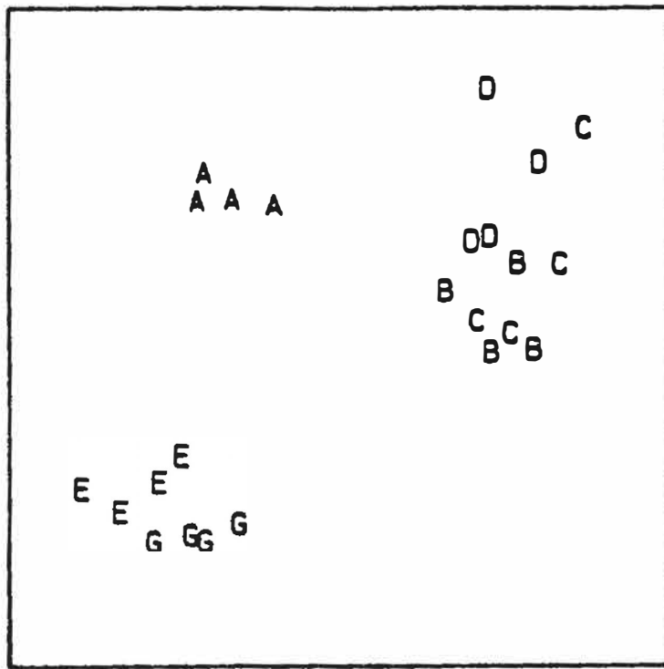
Fig. 14.3. MDS of 4 replicates at each of sites A-E,G (Bray-Curtis similarities on \sqrt{} -transformed counts).
