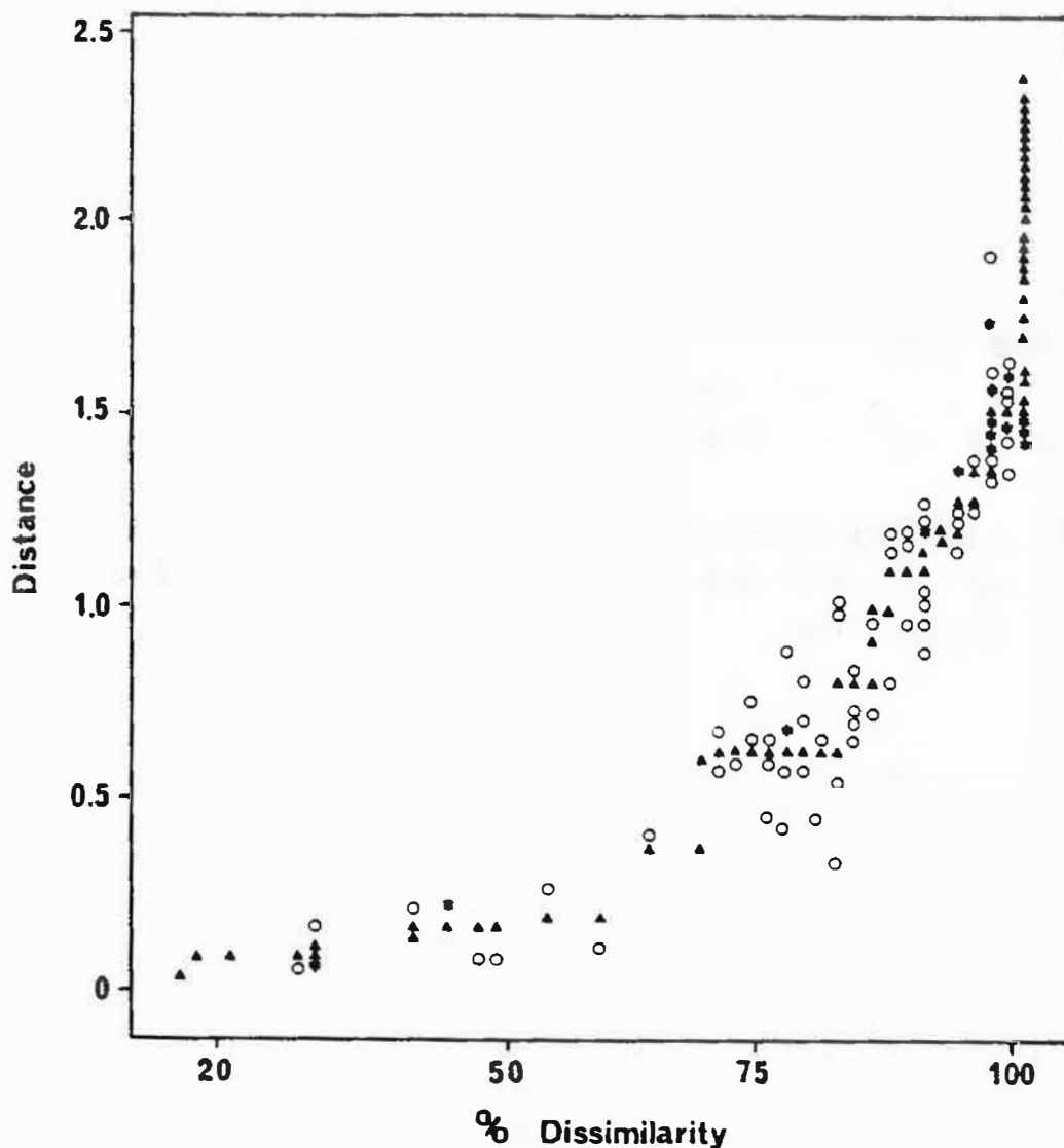
Fig. 5.2. Exe nematodes. "Shepard diagram" of distance ( d ) in MDS plot (Fig. 5.1) against dissimilarity ( \delta ) in Bray-Curtis matrix.
