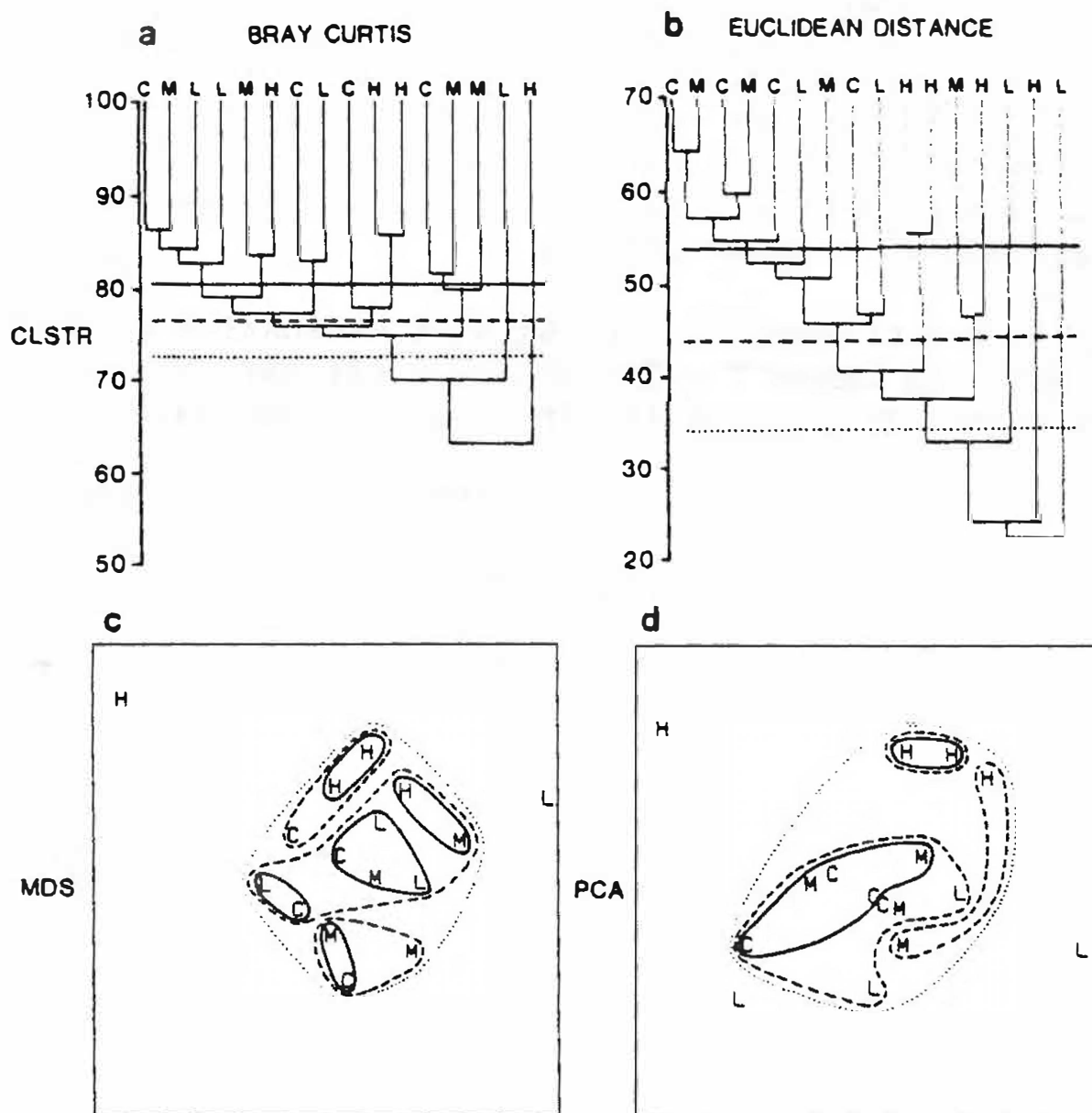
Fig. 5.5. Mesocosm: 4 replicates from 4 treatments (reduced species and log transform, as Fig. 4.2). a),c) Group-average clustering from Bray-Curtis similarities; clusters formed at 3 (arbitrary) levels superimposed on the MDS obtained from the same similarities (stress = 0.19). b),d) Group average clustering from "Euclidean distance" (dis)similarities superimposed on the PCA (Fig. 4.2). (Euclidean distance is the dissimilarity measure implicit in a PCA ordination.)
