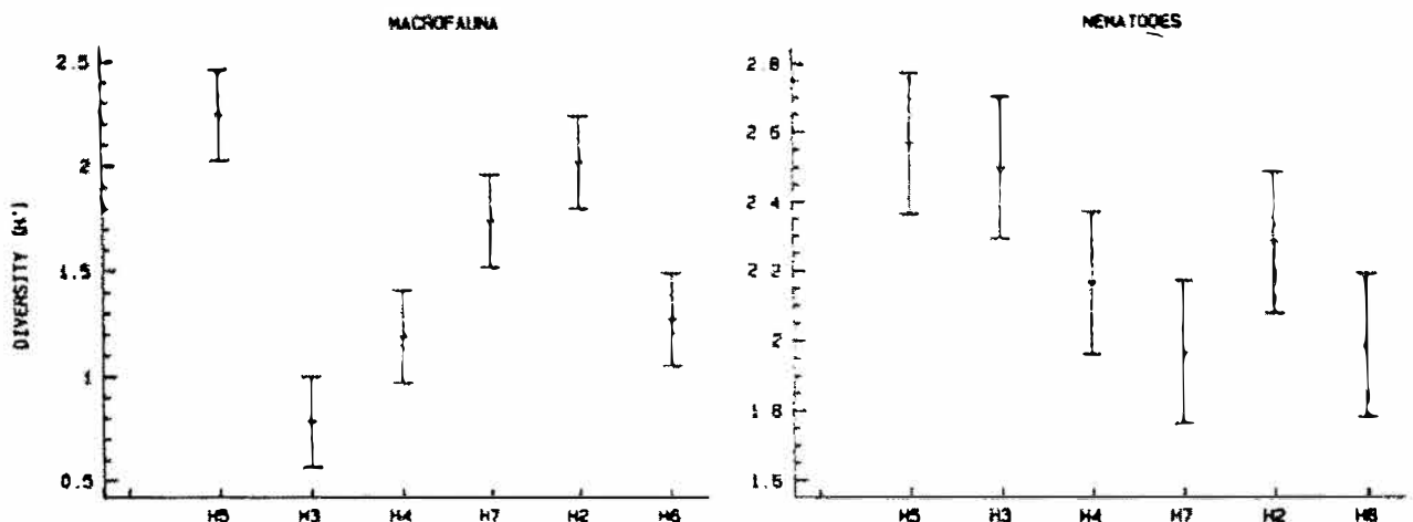
Fig. 8.1. Diversity ( H' ) and 95% confidence intervals for macrobenthos (left) and meiobenthic nematodes (right) at six stations.
