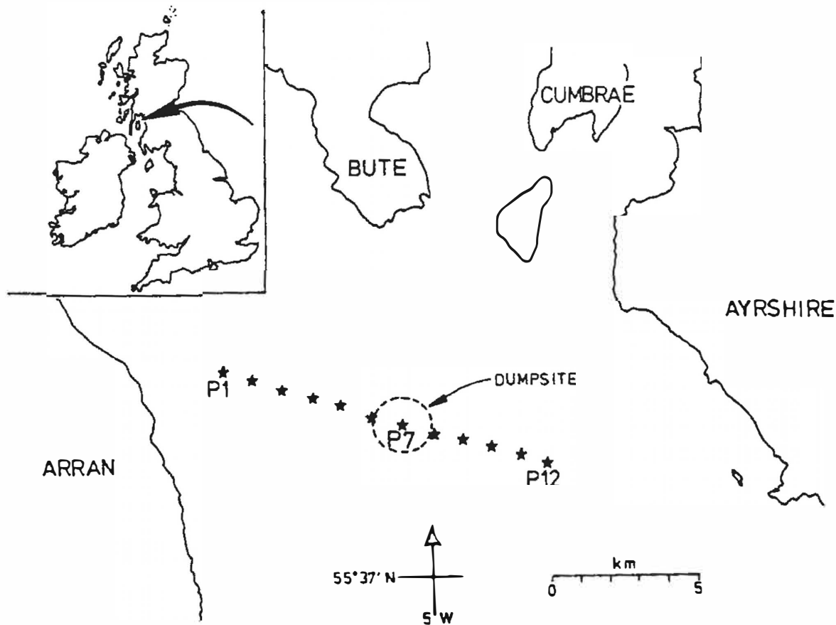
Fig. 8.7. Map showing location of dumping-ground. Centre of dump-site denoted by dashed circle: positions of sampling stations (P1 - P12) identified by asterisks.
