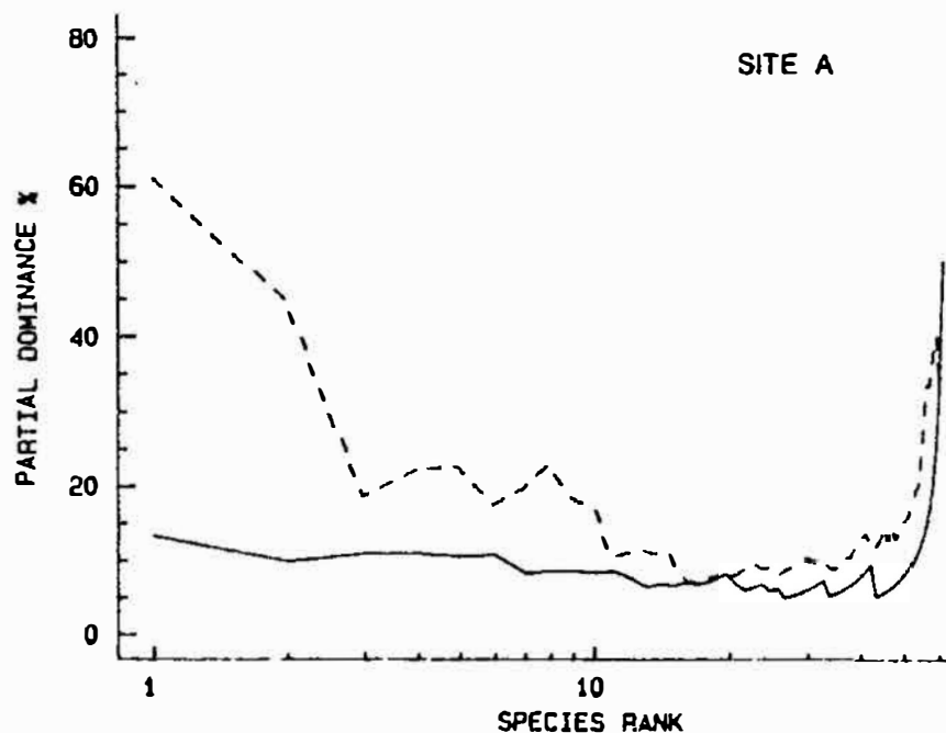
Fig. 8.10. Partial dominance curves (abundance/biomass comparison) for reference station A (c.f. Figs 8.9a and c for corresponding standard and transformed ABC plots). This illustrates the typically undisturbed condition.
