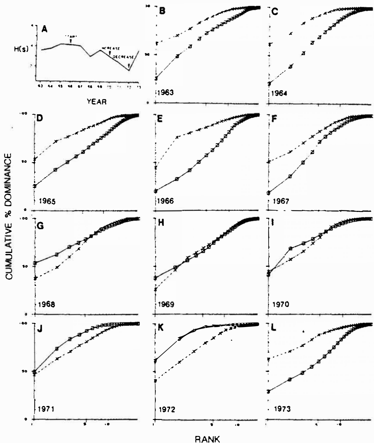
Fig. 10.7. Loch Linnhe macrofauna. (A) Diversity H' , (B)-(L) "ABC" curves for 11 years, of biomass (crosses) and abundance (squares), for data aggregated to families, Warwick (1988).
