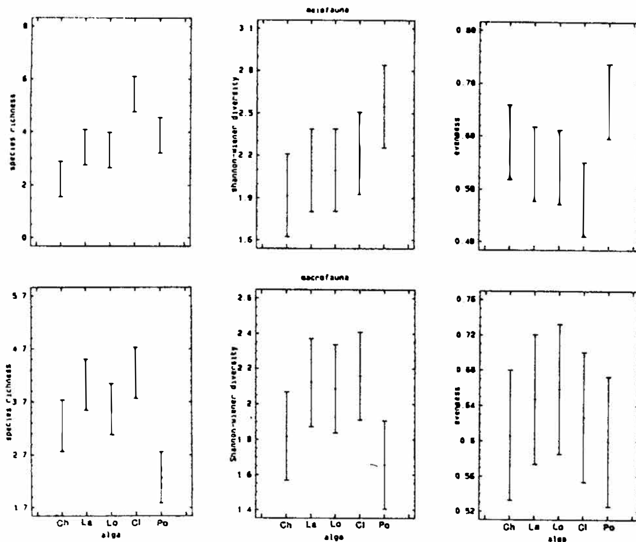
Fig. 14.12. Species richness (left), Shannon diversity (middle) and evenness (right) for meiofauna (top) and macrofauna (bottom), with 95% confidence intervals. Ch = Chondrus, La = Laurencia, Lo = Lomentaria, Cl = Cladophora, Po = Polysiphonia.
