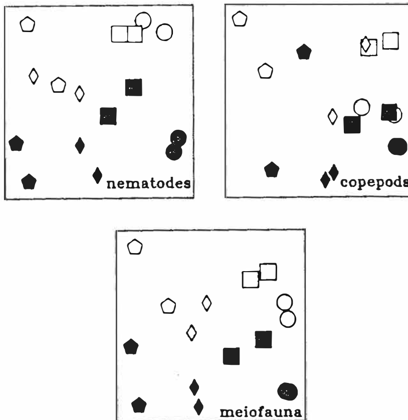
Fig. 14.17. MDS plots for nematode, copepod and 'meiofauna' (nematodes + copepods) abundance. Open symbols = disturbed samples, closed = undisturbed (different shapes denote the four blocks).
