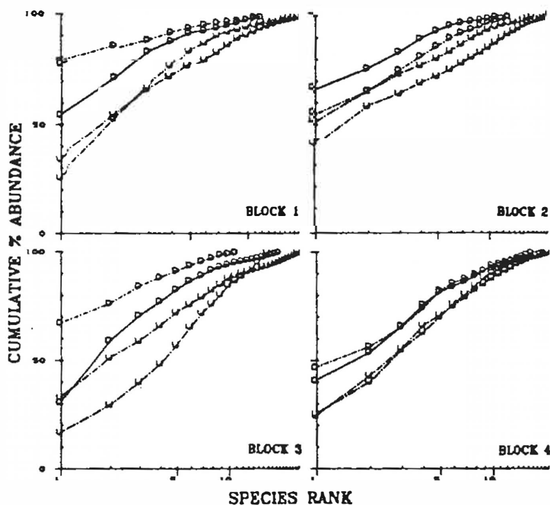
Fig. 13.4. k -dominance curves for disturbed (D) and undisturbed (U) samples in 4 separate sampling blocks.
