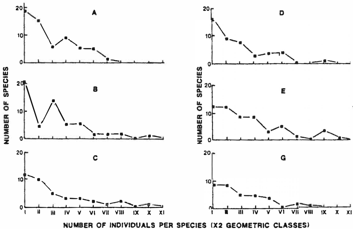
Fig. 1.5. Frierfjord macrofauna, sites A-E,G. Number of species against number of individuals per species in geometric classes (I = 1 individual per species, II = 2-3 ind. per spp., III = 4-7, IV = 8-15 etc.). Gray et al. (1988).
