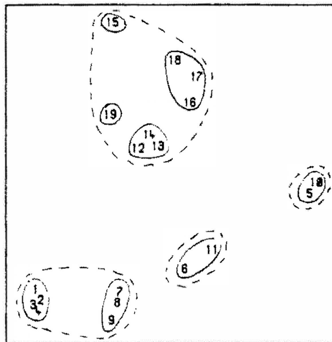
Fig. 5.4. Exe nematodes. MDS (as Fig. 5.1) with clusters indicated at: --- 15%, — 30% similarity.
