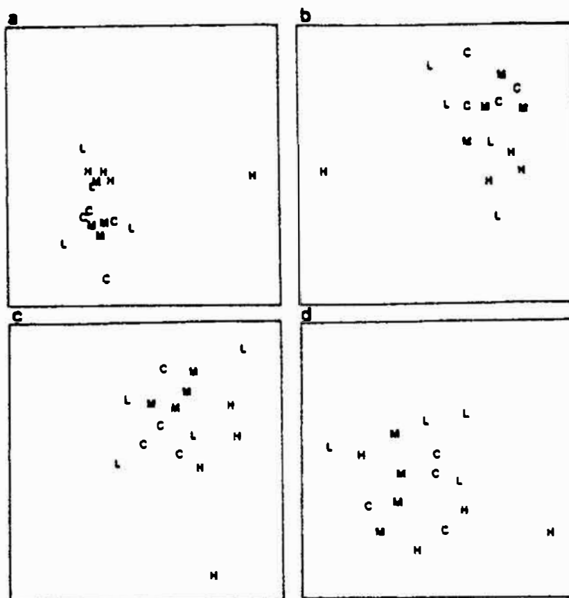
Fig. 9.1. GEEP mesocosm nematodes (Warwick et al. 1988). MDS of 4 boxes from 4 treatments (C,L,M,H). Bray-Curtis similarities from transformed counts: a) no transform, b) \sqrt{y} , c) \log(1+y) , d) presence/absence. Stress: a) 0.08, b) 0.14, c) 0.19, d) 0.19.
