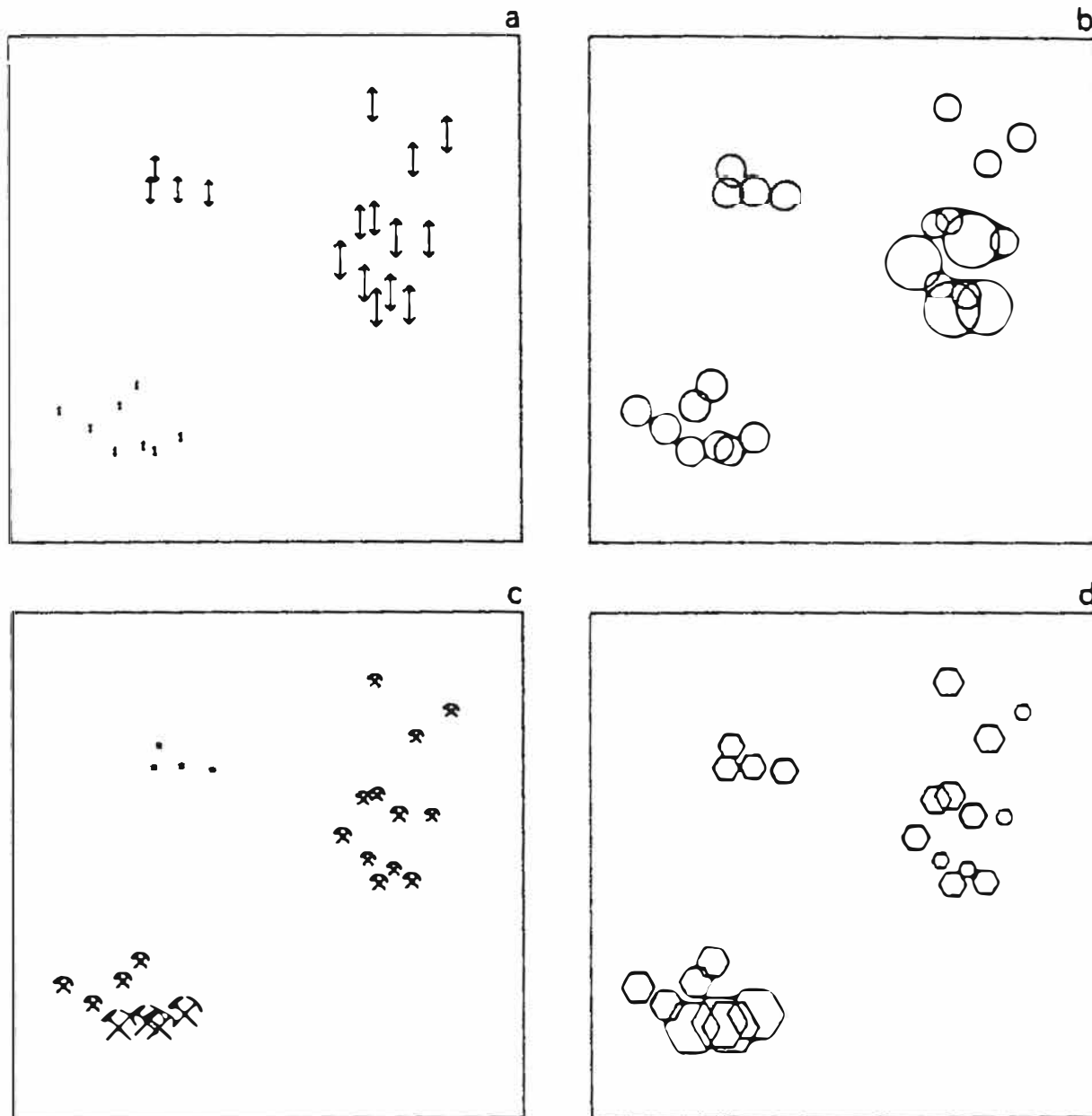
Fig. 1.9. Frierfjord macrofauna. Values of four environmental variables: (a) water depth, (b) sediment grain size, (c) metal and (d) PAH concentrations in sediment, superimposed on the abundance-based MDS.
