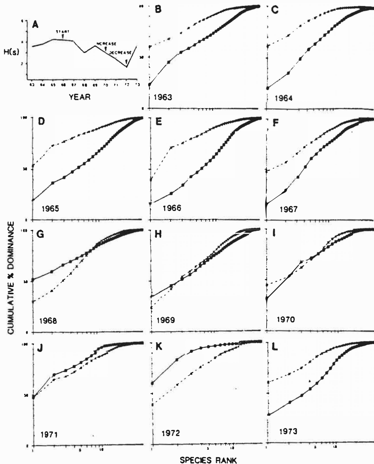
Fig. 10.6. Loch Linnhe macrofauna. (A) Diversity H' , (B)-(L) "ABC" curves for 11 years, of biomass (crosses) and abundance (squares). Analysis at species level, Warwick (1986).
