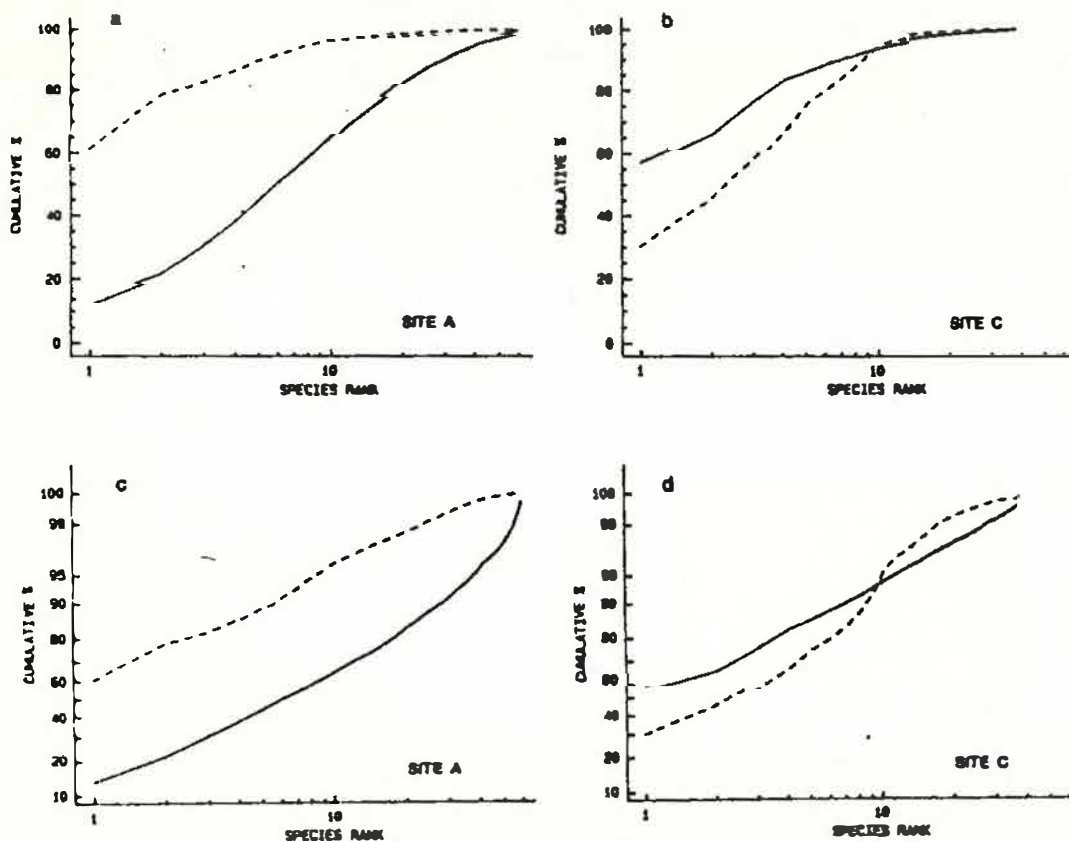
Fig. 8.9. a), b) Standard ABC plots for sites A (reference) and C (potentially impacted). c), d) ABC plots for sites A and C with the y-axis subjected to modified logistic transformation. Abundance = continuous line, biomass = dashed line.
