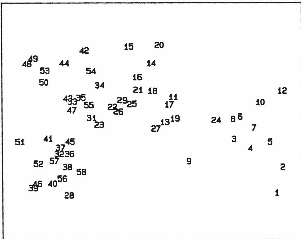
Fig. 11.3. MDS of 57 sites (from Bray-Curtis similarities, on \sqrt{} -transformed counts; stress = 0.11). For map of sites and corresponding cluster analysis, see Figs. 3.2 and 3.3.
