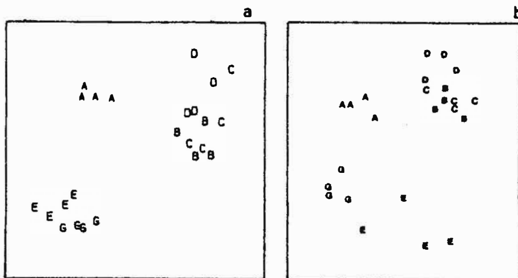
Fig. 10.1. Frierfjord macrofauna counts. Sample MDS (Bray-Curtis, \sqrt{\sqrt{\phantom{x}}} ) for: a) all 110 species, b) 19 random species. (Stress: a) 0.14, b) 0.13).
